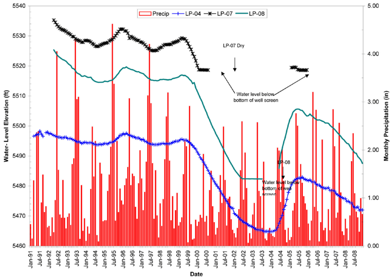
Figure 2-9. Water-level hydrograph for LP-04, LP-07 and LP-08 wells.
