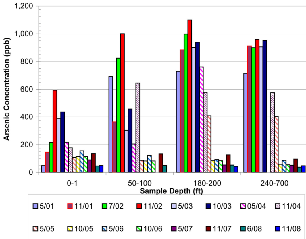
Figure 2-53. Recent changes in the concentration of arsenic at four depths. Both spring and fall sampling events are represented in this figure.
