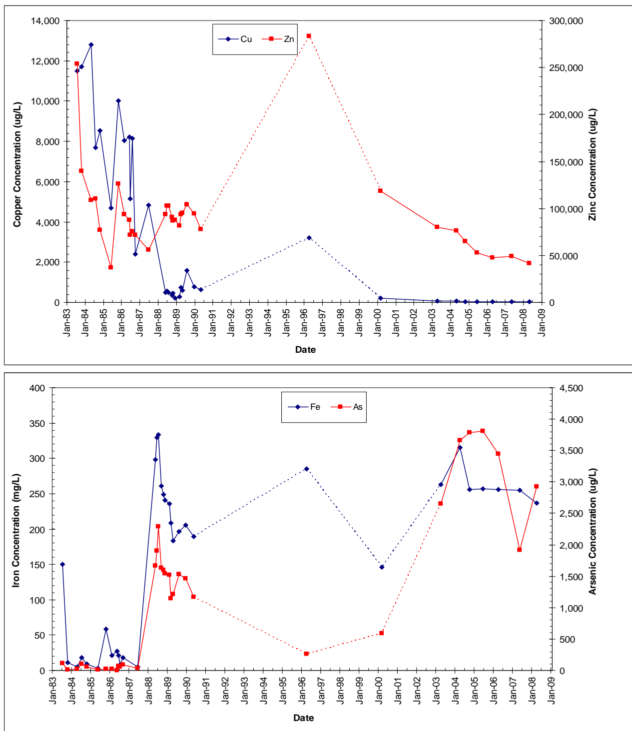
Figure 2-31. Steward Mine quality changes over time.
