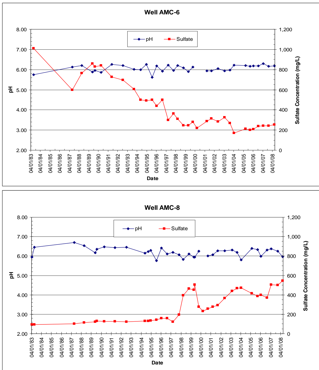
Figure 2-6. Graphs showing pH and sulfate concentration changes over time for wells AMC-6 (top) and AMC-8 (bottom).
