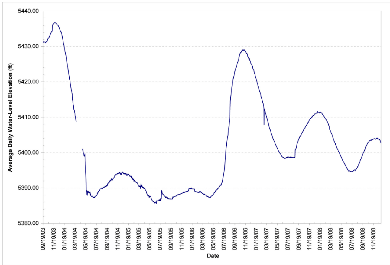
Figure 5-7. Average daily water-level elevations hydrograph for the Belmont Well #1.
