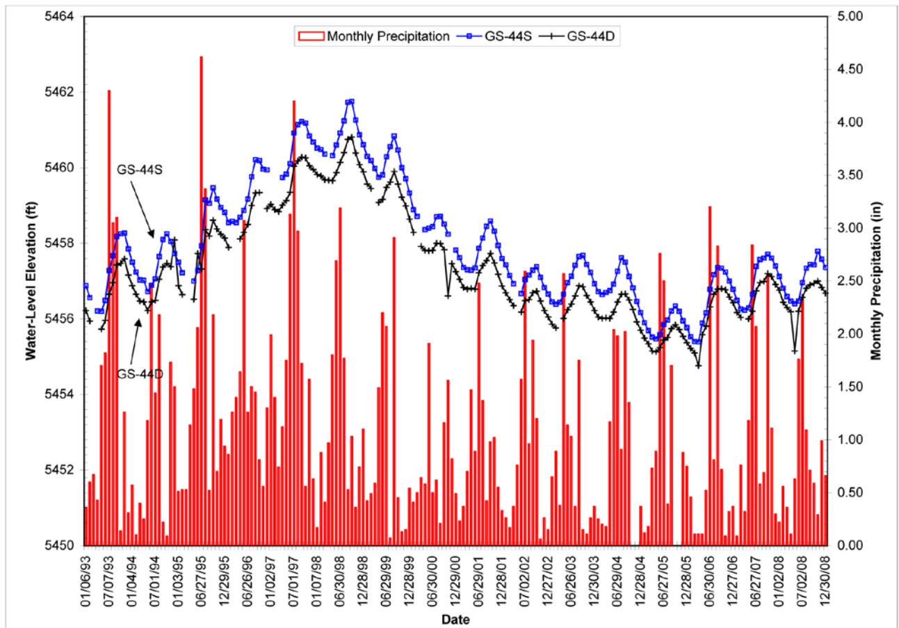
Figure 2-19. Water-level hydrographs for GS-44S and GS-44D wells.
