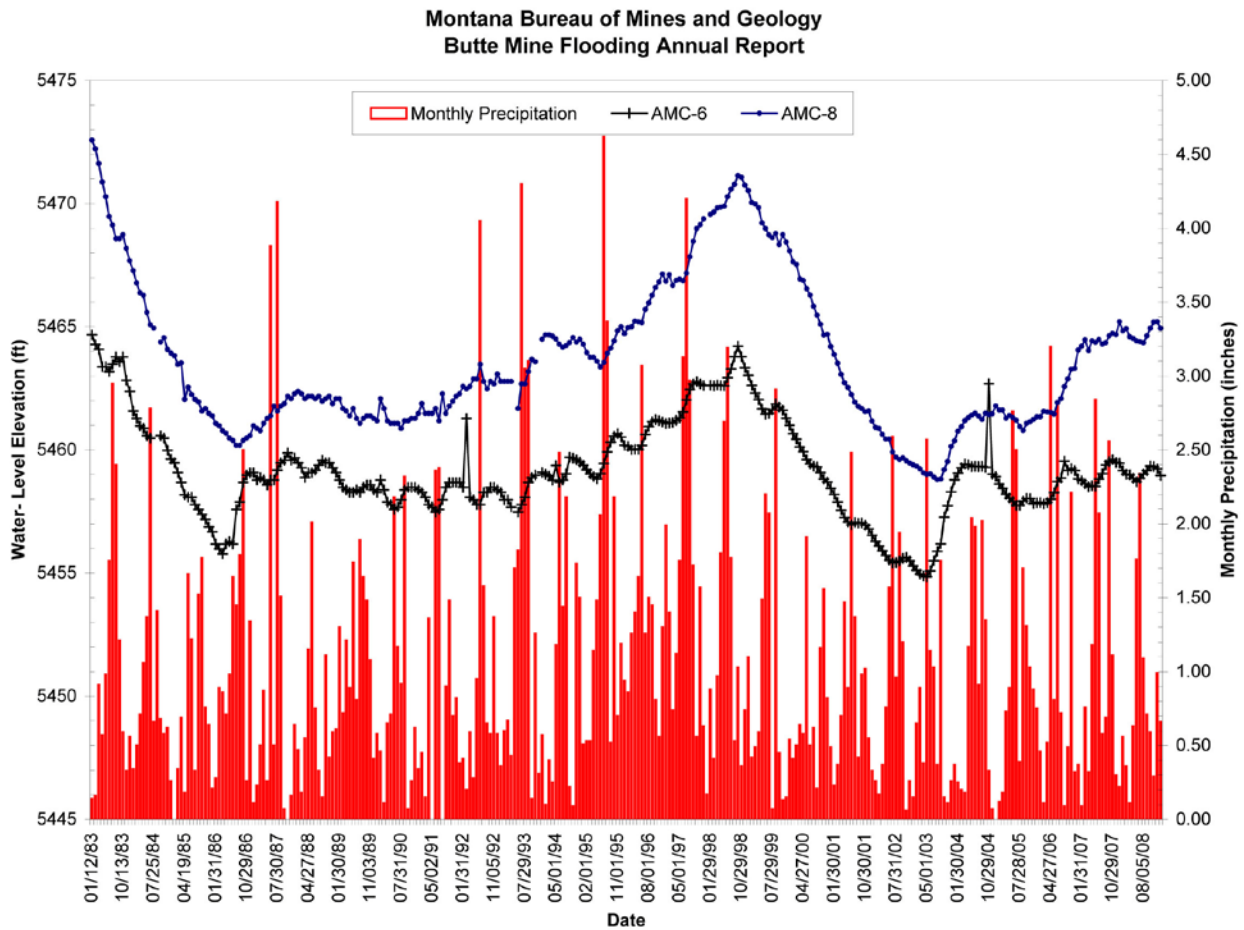
Figure 2-4. Water-level hydrographs for AMC-6 and AMC-8 wells.
