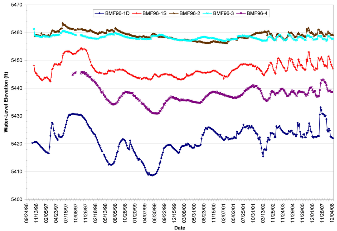
Figure 3-7. Water-level hydrographs for BMF96 series wells.
