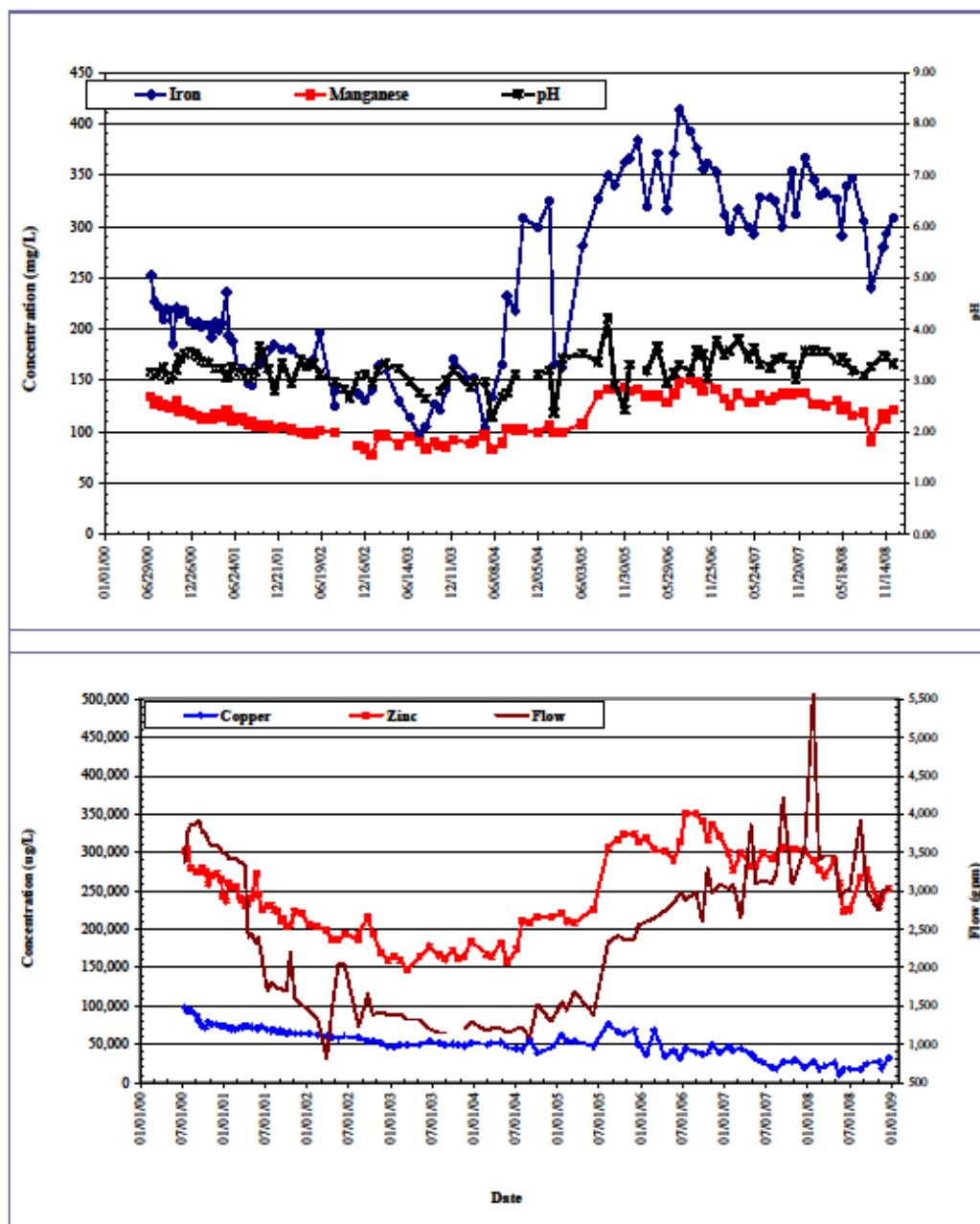
Figure 2-54. Horseshoe Bend water quality comparisons of selected constituents, 2000-2008.
