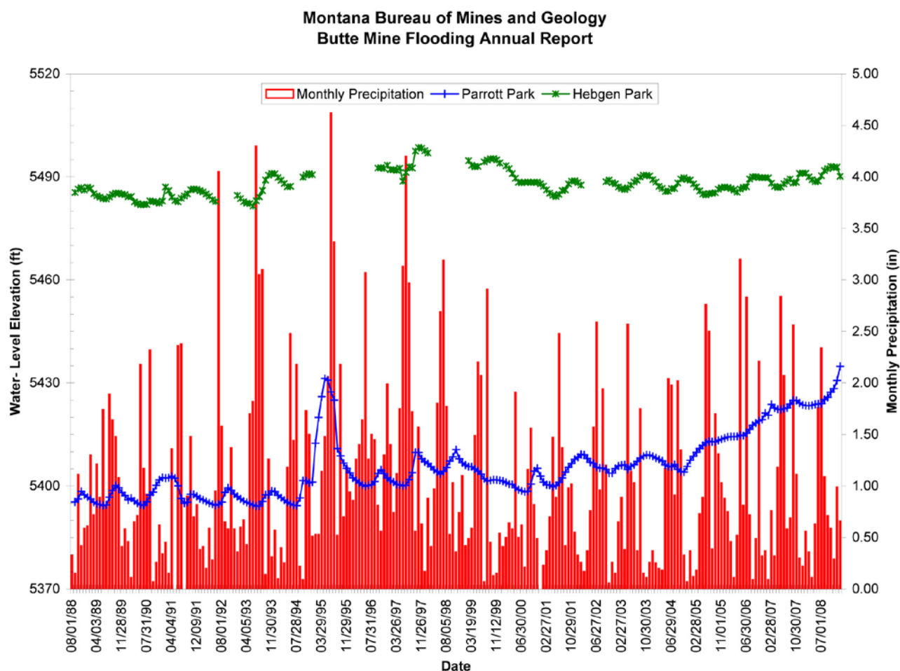
Figure 5-5. Water-level hydrograph for Parrott and Hebgen Park wells.
