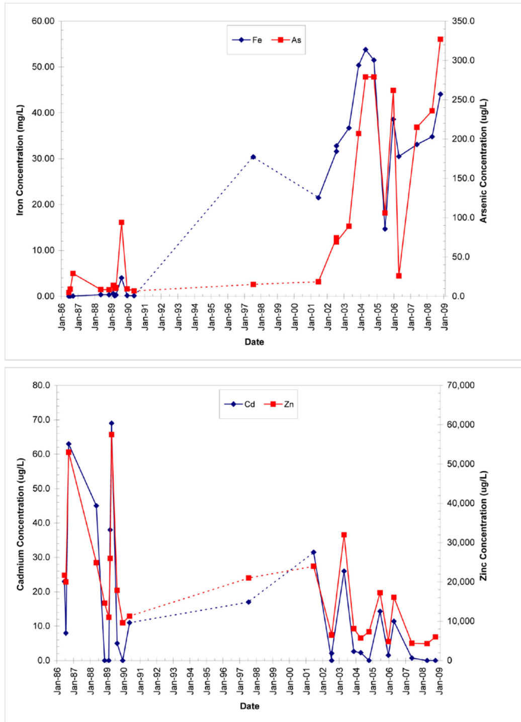
Figure 2-30. Anselmo Mine water quality changes over time.
