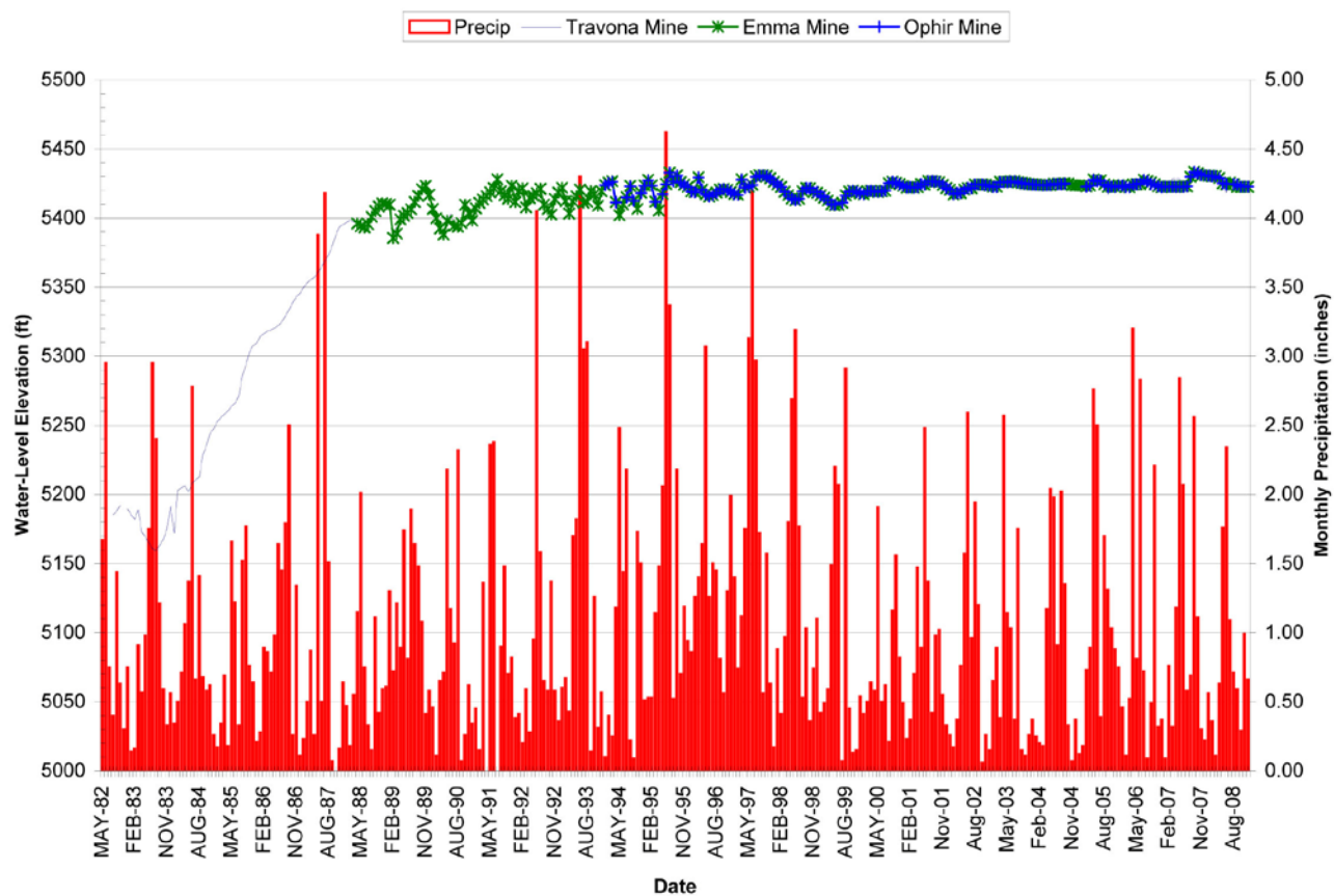
Figure 3-4. West Camp Mines water-level hydrographs and monthly precipitation totals.
