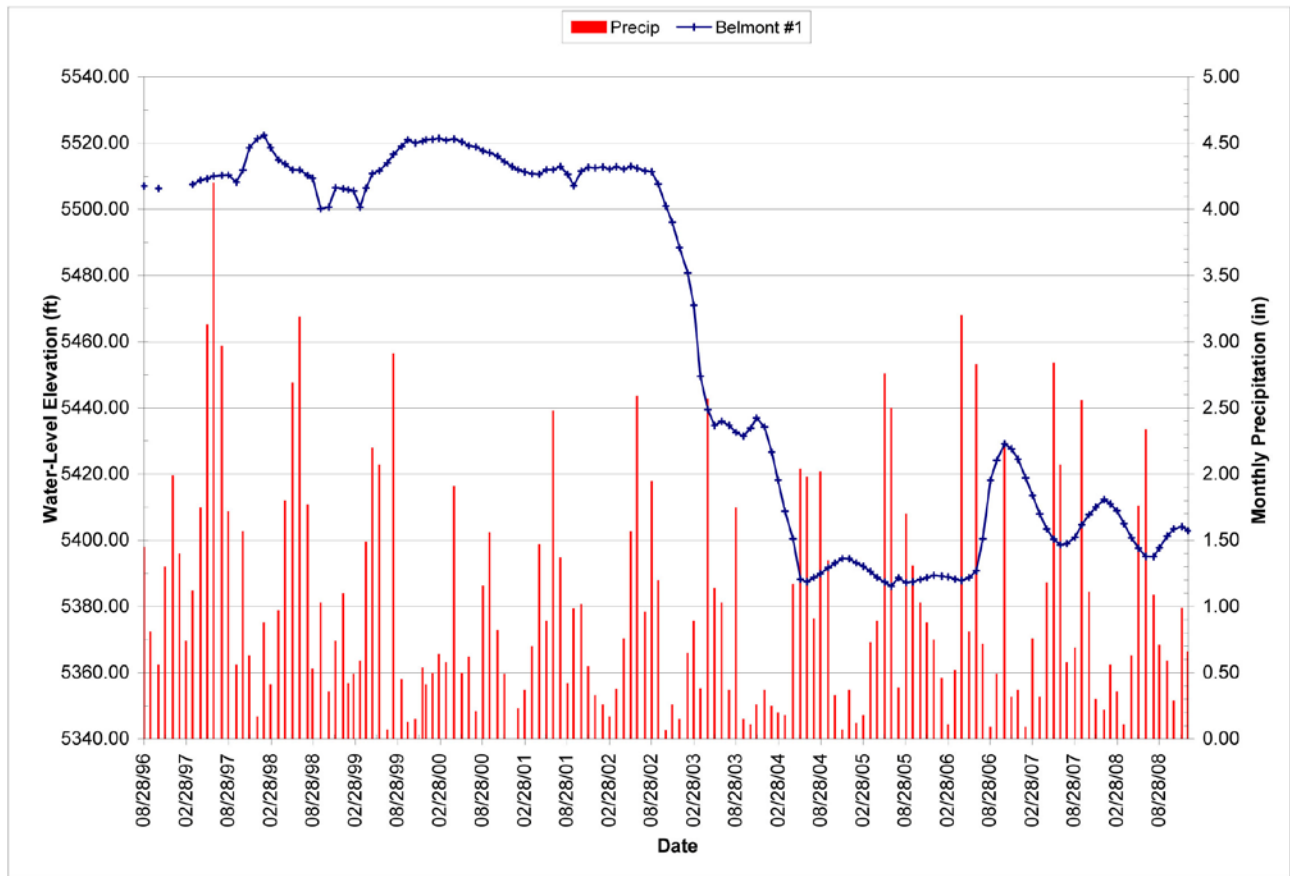
Figure 5-6. Water-level hydrograph for Belmont Well #1.
