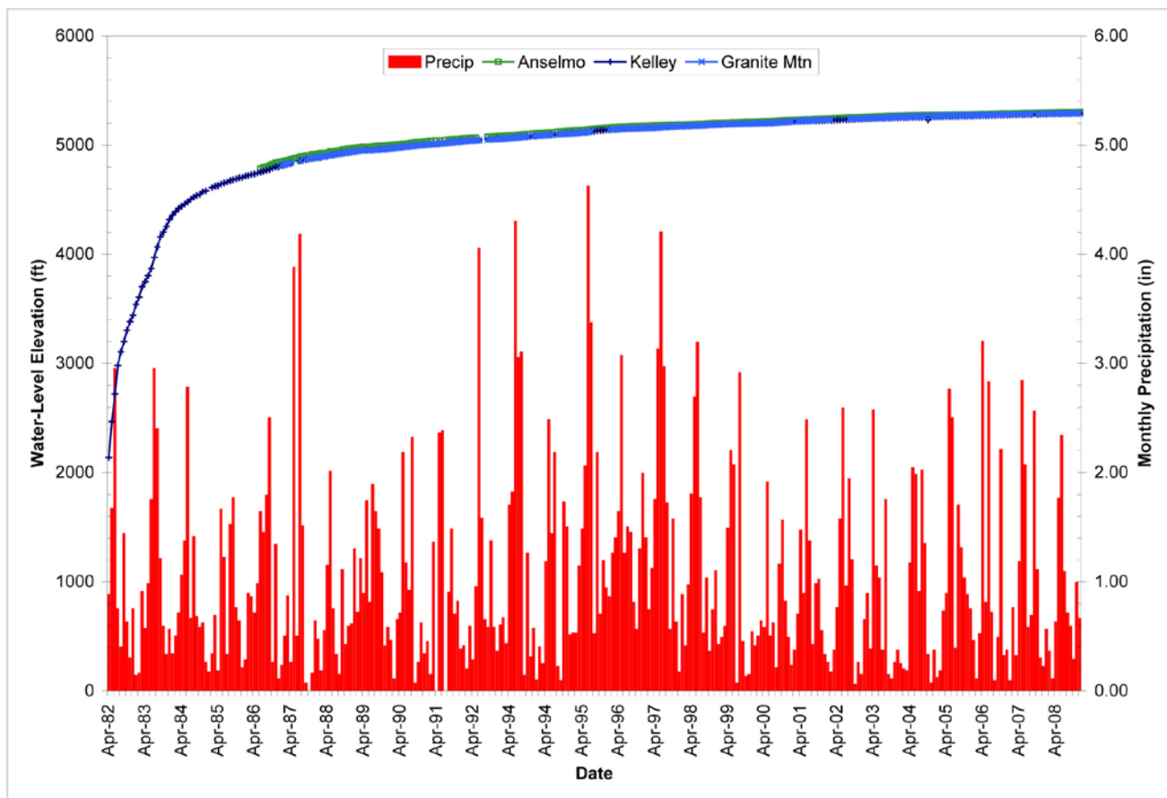
Figure 2-28. Water-level hydrographs for selected East Camp Mines, with monthly precipitation.
