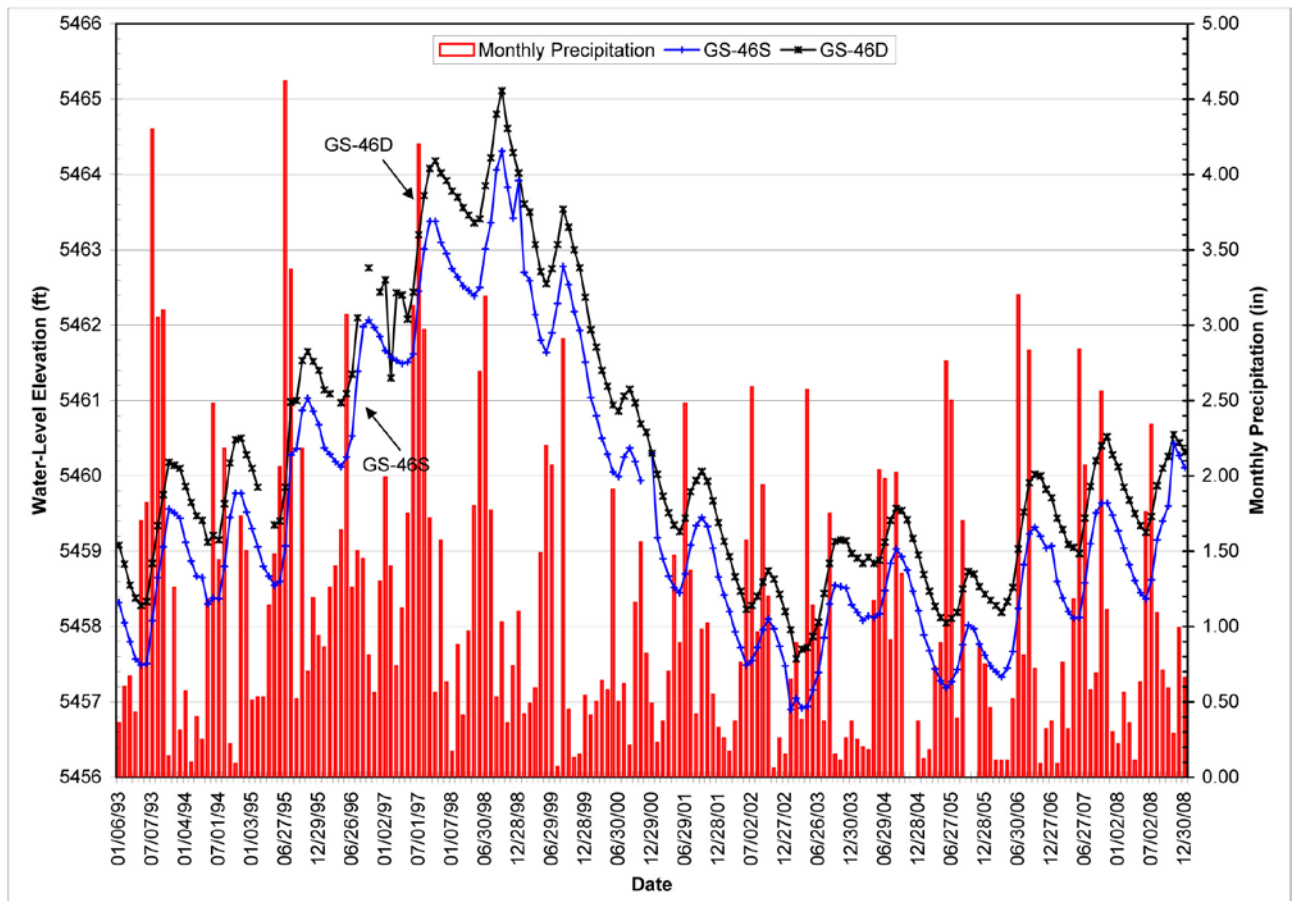
Figure 2-20. Water-level hydrographs for GS-46S and GS-46D wells.
