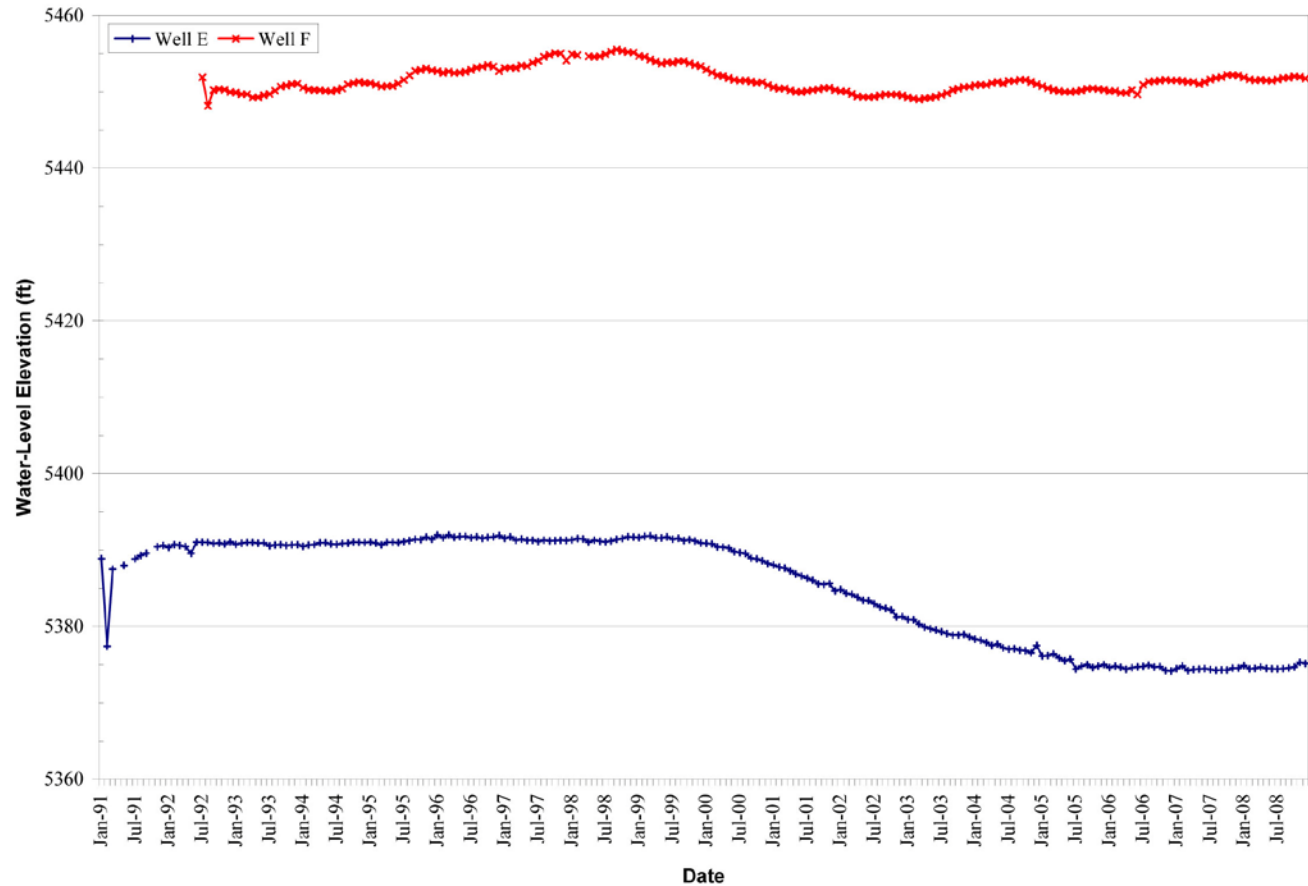
Figure 2-36. Water-level hydrograph for bedrock wells E and F.
