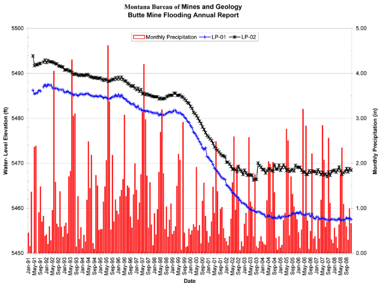
Figure 2-8. Water-level hydrographs for LP-01 and LP-02 wells.
