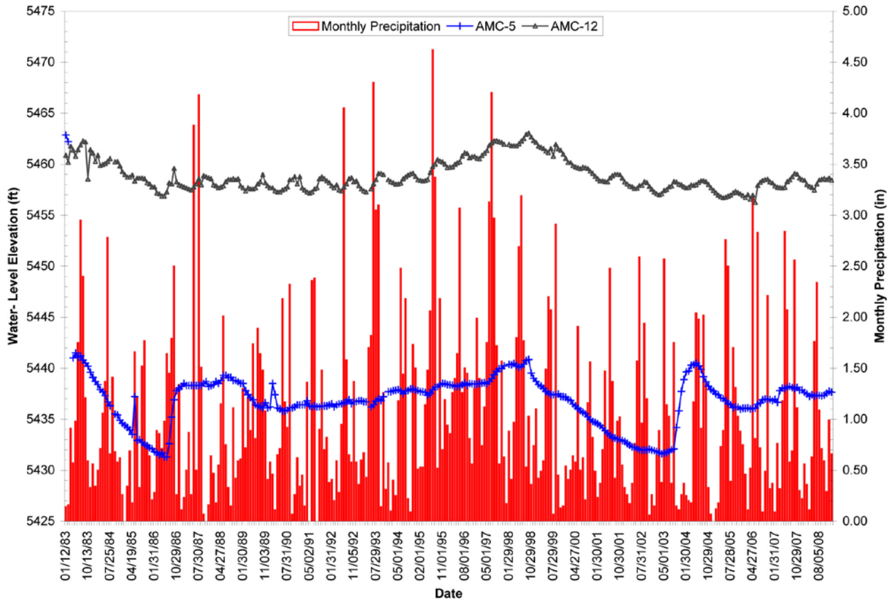
Figure 2-3. Water-level hydrographs for AMC-5 and AMC-12 wells.
