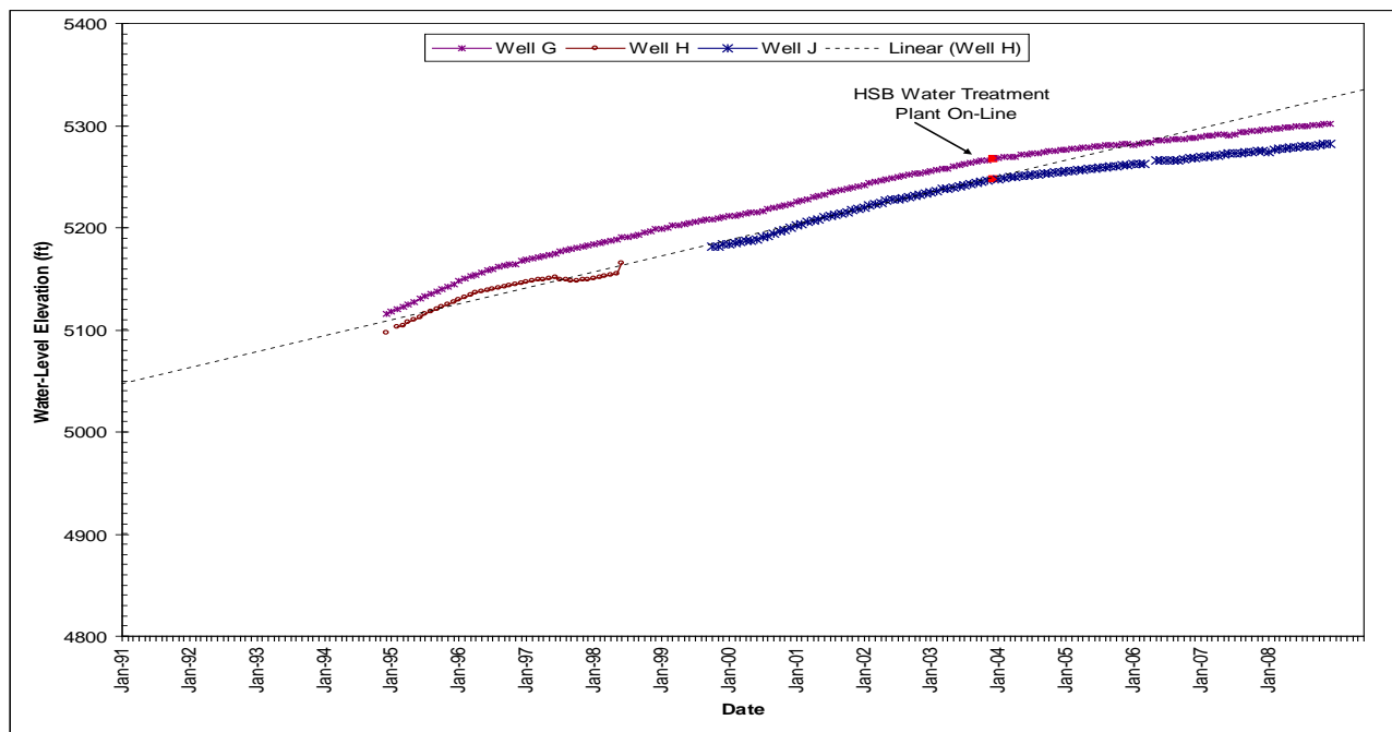
Figure 2-34. Water-level hydrographs for bedrock wells G, H, and J.
