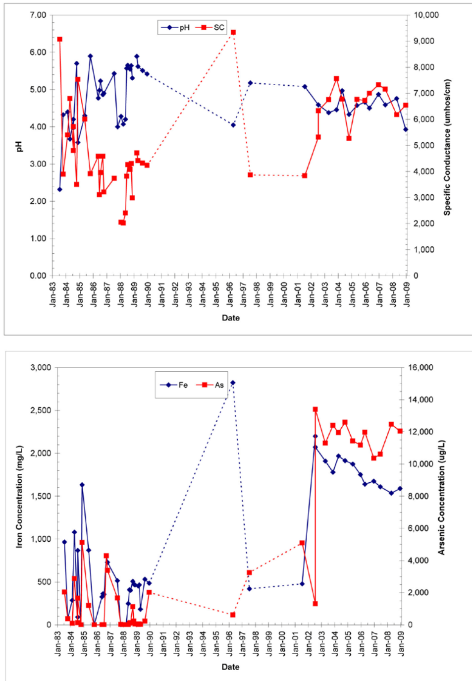
Figure 2-29. Kelley Mine water quality changes over time.
