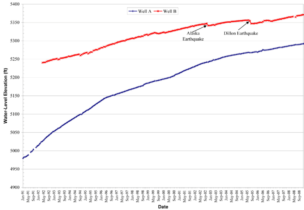
Figure 2-35. Water-level hydrograph for bedrock wells A and B.
