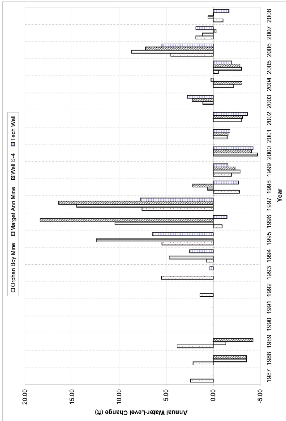
Figure 4-2. Outer Camp sites annual water-level change.
