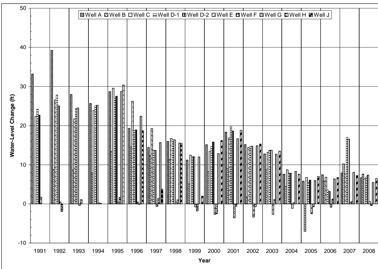
Figure 2-32. RI/FS bedrock wells annual water-level change.
