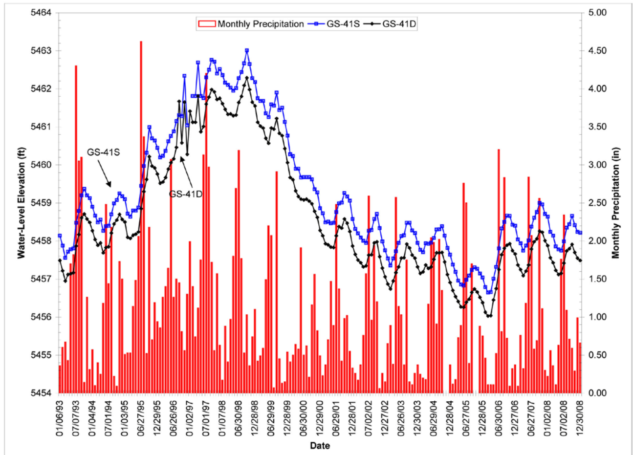
Figure 2-18. Water-level hydrographs for GS-41S and GS-41D wells.
