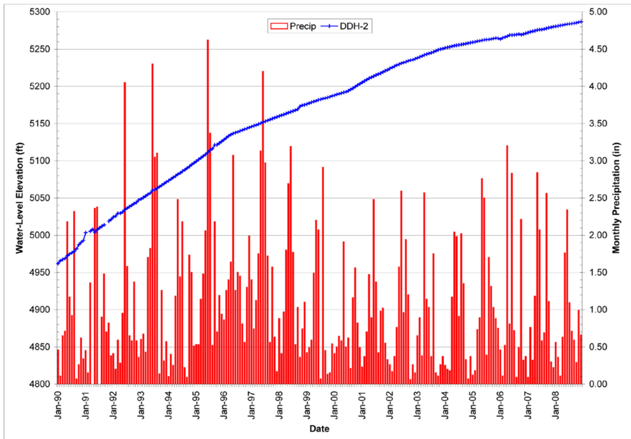
Figure 2-41. Water-level hydrograph for bedrock well DDH-2.
