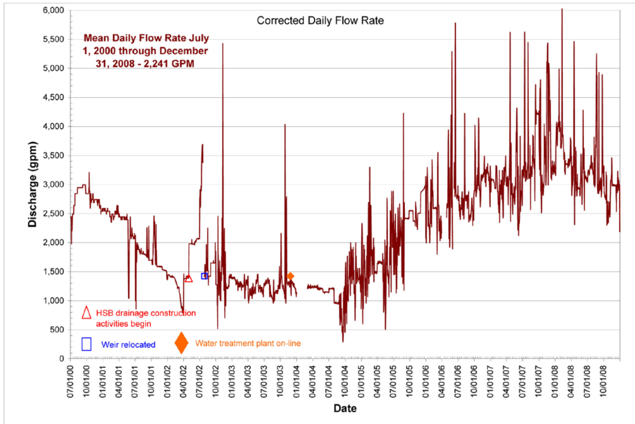
Figure 2-43. Horseshoe Bend Drainage flow rate, July 2000 through December 2008.
