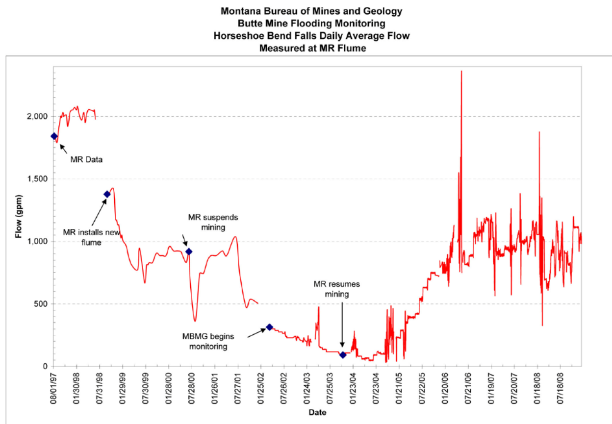
Figure 2-44. Horseshoe Bend Falls long-term daily average flow rates, includes both MR and MBMG data.
