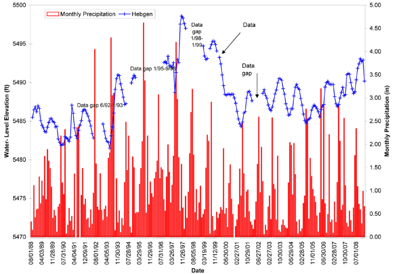
Figure 5-3. Water-level hydrograph for the Hebgen Park Well.
