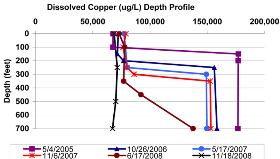
Figure 2-52. Time-series depth profile of copper concentration in the Berkeley Pit.
