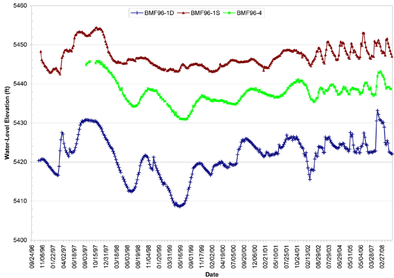
Figure 3-5. Water-level hydrographs for West Camp BMF96-1D, BMF96-1S, and BMF96-4 wells.
