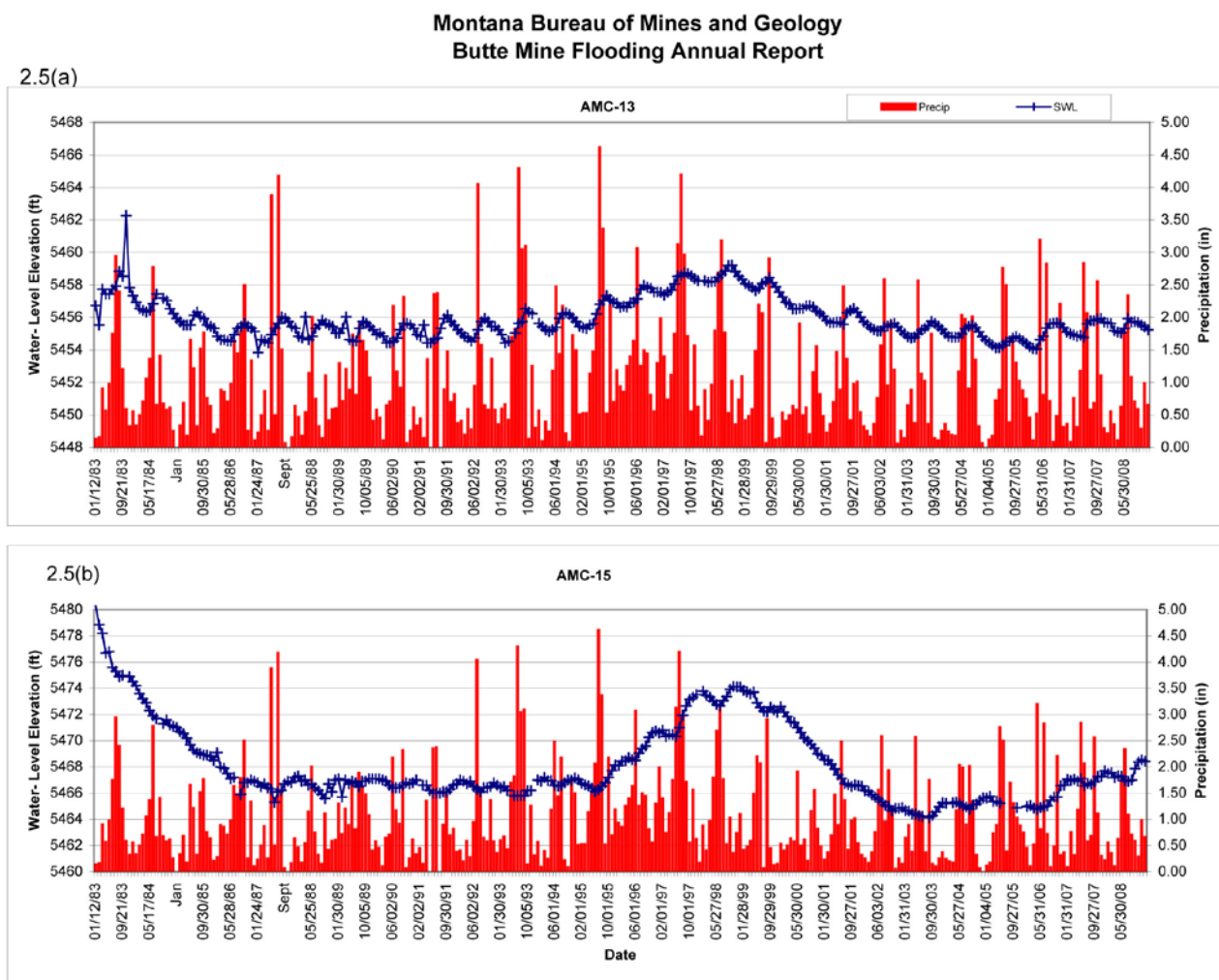
Figure 2-5. Water-level hydrographs for AMC-13 (a), and AMC-15 (b) wells.
