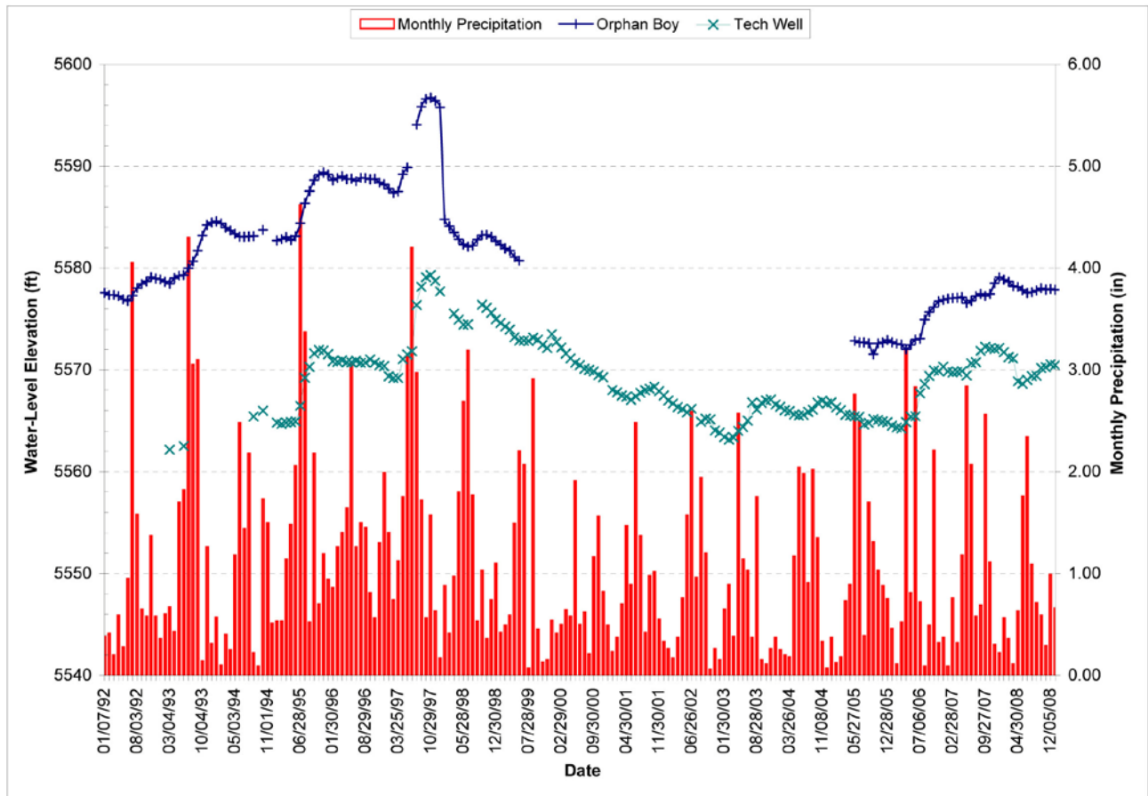
Figure 4-3. Water-level hydrograph of the Orphan Boy Mine and Montana Tech wells.
