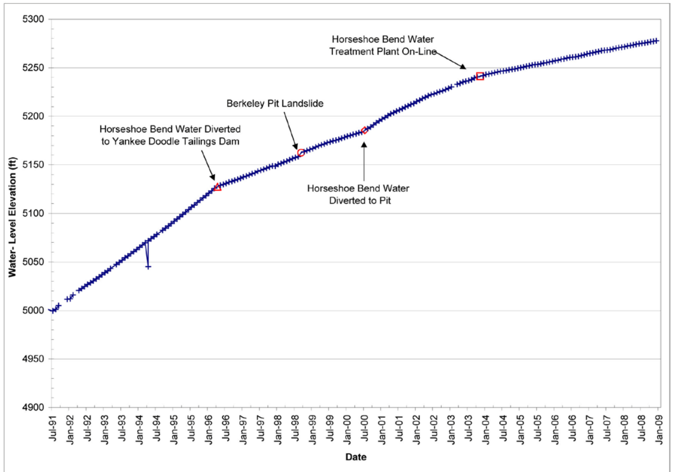
Figure 2-27. Water-level hydrograph for the Berkeley Pit.
