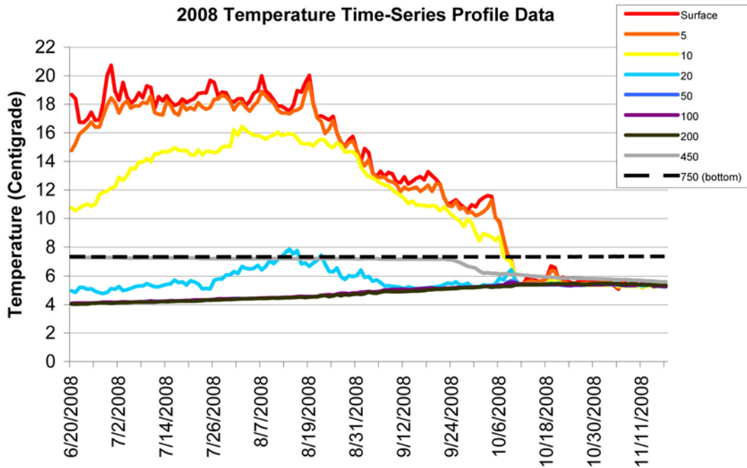
Figure 2-49 Time series temperature profiles at nine varying depths in the Berkeley Pit.
