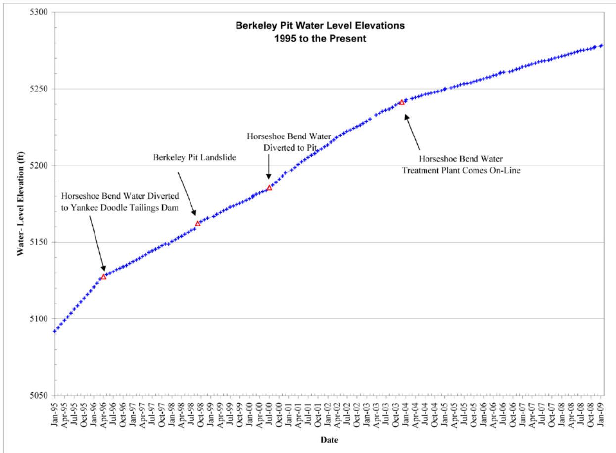
Figure 2-42. Water-level hydrograph of Berkeley Pit, 1995-2008.
