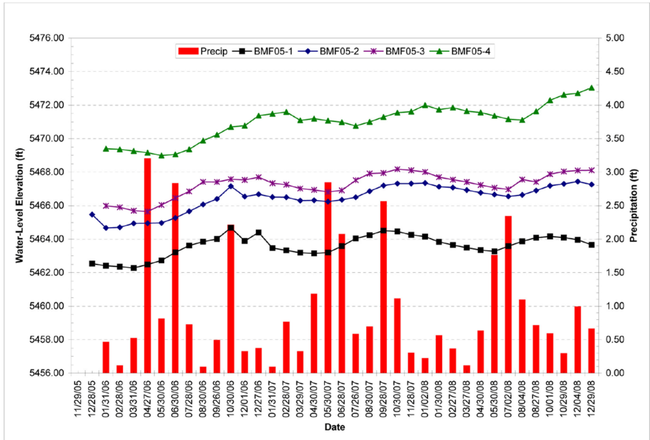
Figure 2-22. Monthly water-levels versus precipitation, BMF05 series wells.
