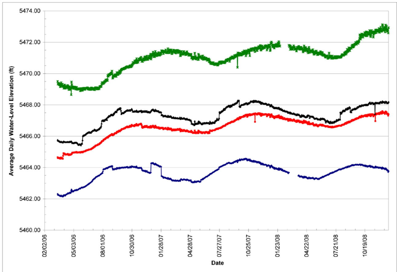
Figure 2-21. Average daily water-levels for BMF05 series wells.
