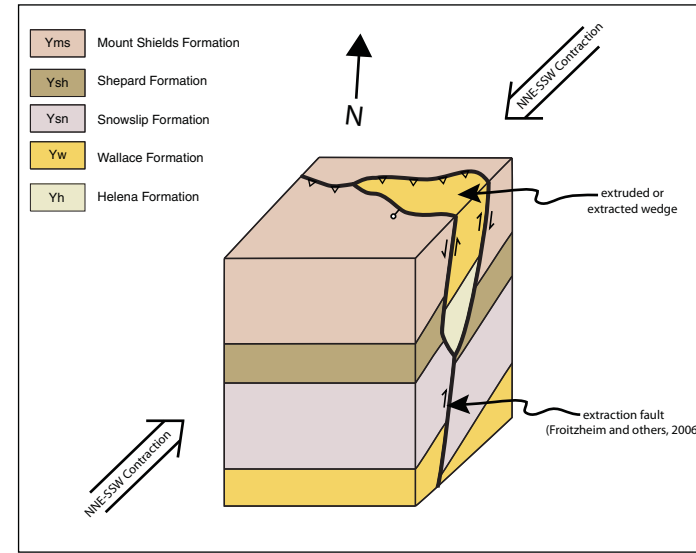
Figure 3. Block diagram showing how horizontal contraction can generate synchronous reverse and normal faults through an extrusion or extraction process. This type of normal fault has been termed a "shortening-induced normal fault" (Ring and Glodny, 2010). Modified from Reid and others (1995).
