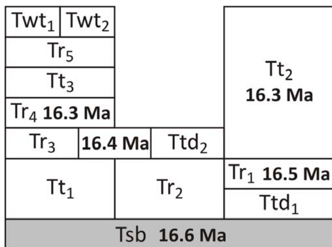
Figure 4: Middle Miocene stratigraphy, chronology, and map unit abbreviations and names. Also pictured are symbols associated with these units as they appear on the geochemical plots.
