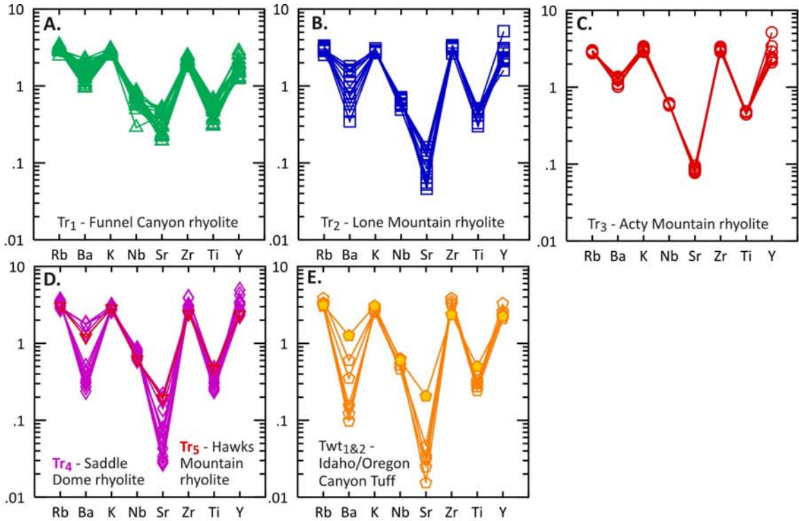
Figure 11: Rhyolite multi-element plots. Elements normalized to average total crust of Rudnick and Fountain (1995). (A) Funnel Canyon rhyolite; (B) Lone Mountain rhyolite; (C) Acty Mountain rhyolite; (D) Saddle Dome and Hawks Mountain rhyolites; (E) proposed correlatives to Idaho/Oregon Canyon Tuff.
