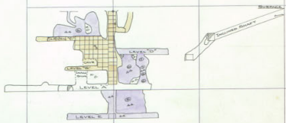
SECTION NORTH PLANE OF VEIN DIP 20° SOUTH
