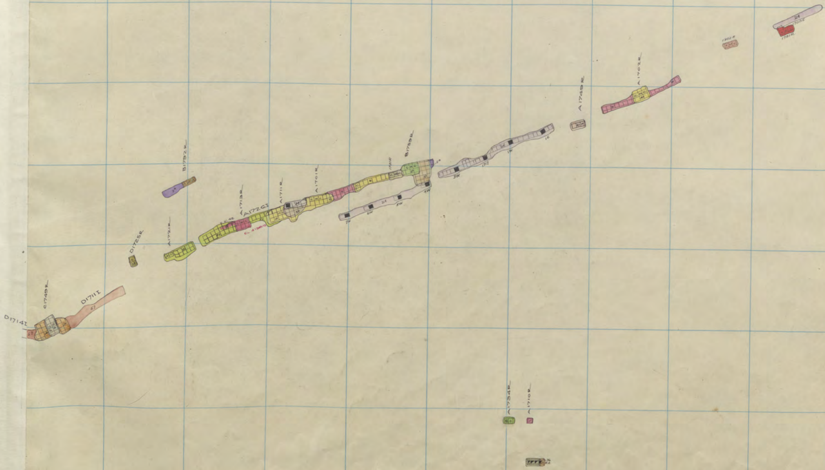
Anselmo 1700 Level, 3 rd Floor.
