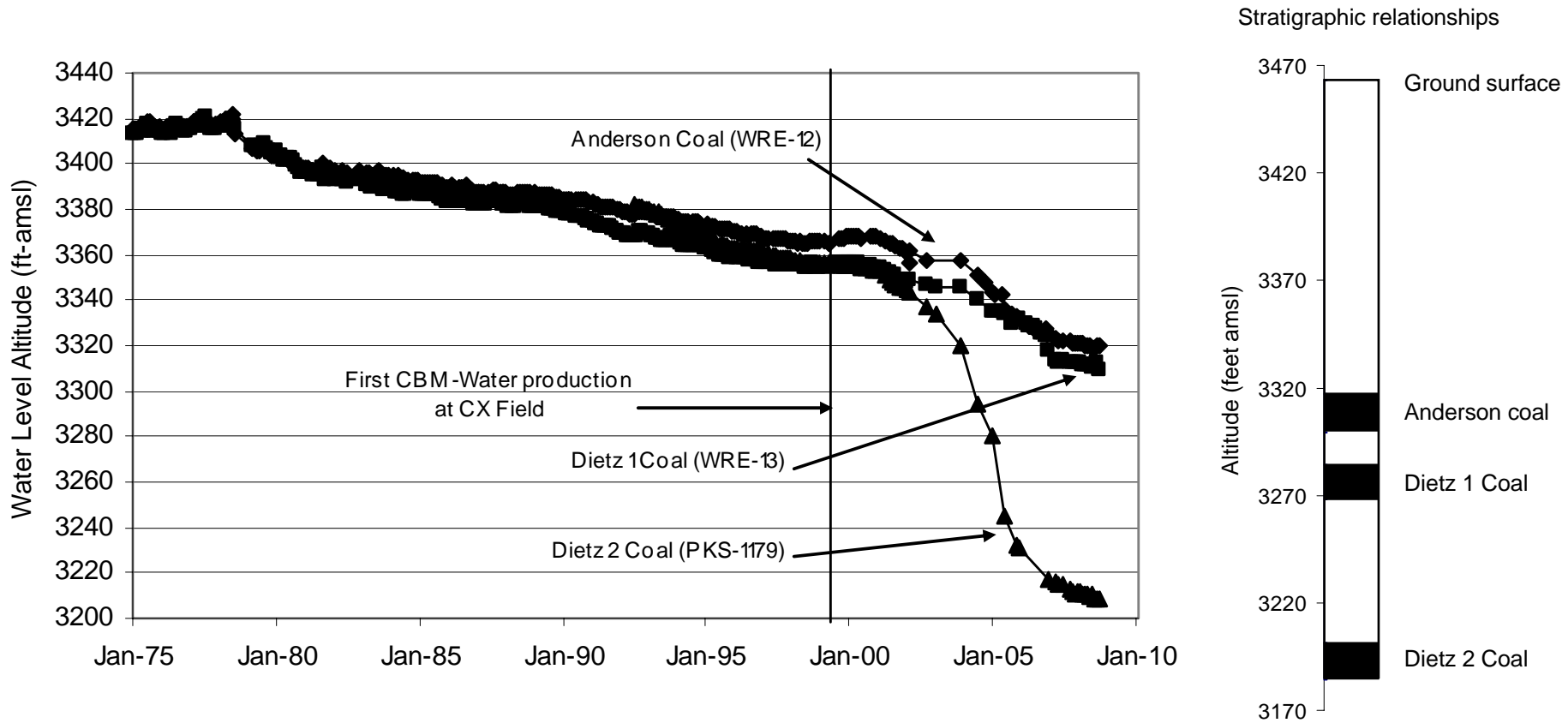
Figure 25. In some locations, the water level response to CBM production in deeper coal seams (PKS-1179) is far greater than in shallower coal seams (WRE-12 and WRE-13). This trend has been noted in coal mining areas also.
