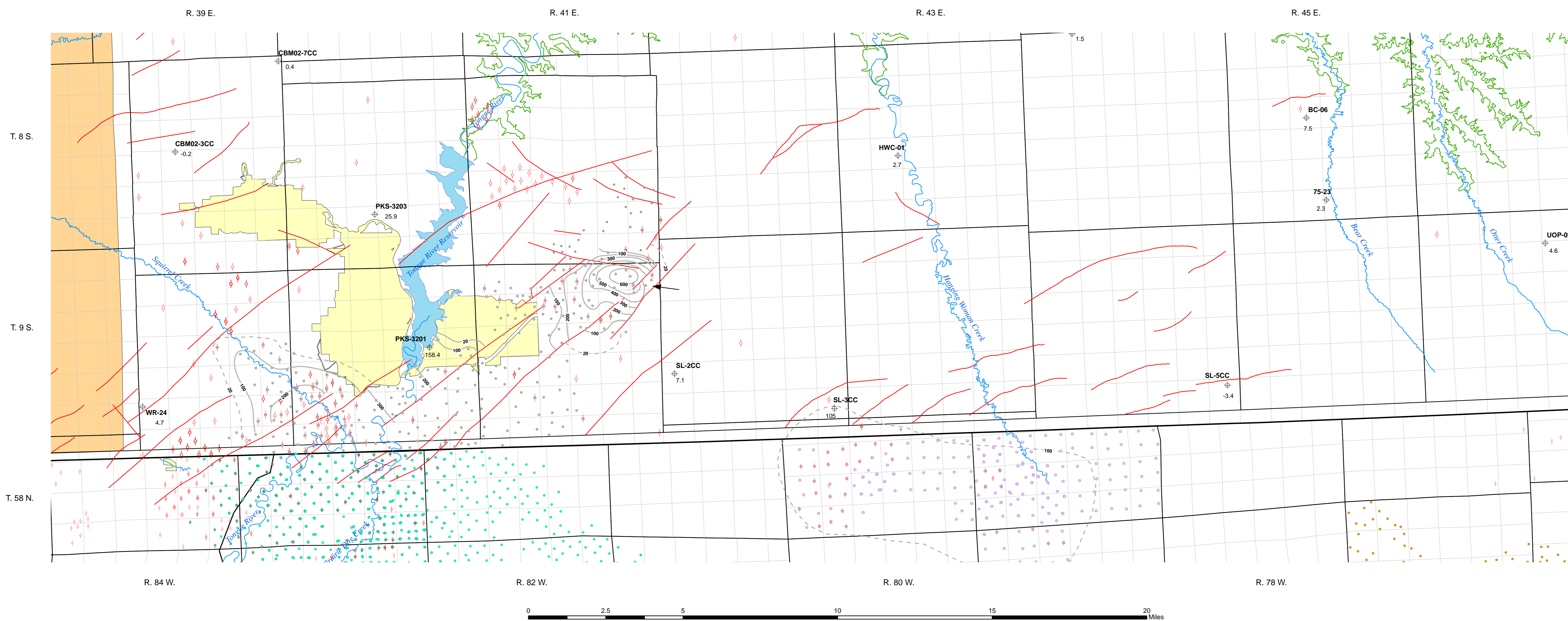
Plate 5. Area of CBM-related potentiometric decline for the Canyon coal in the southern portion of the Powder River Basin, Montana
