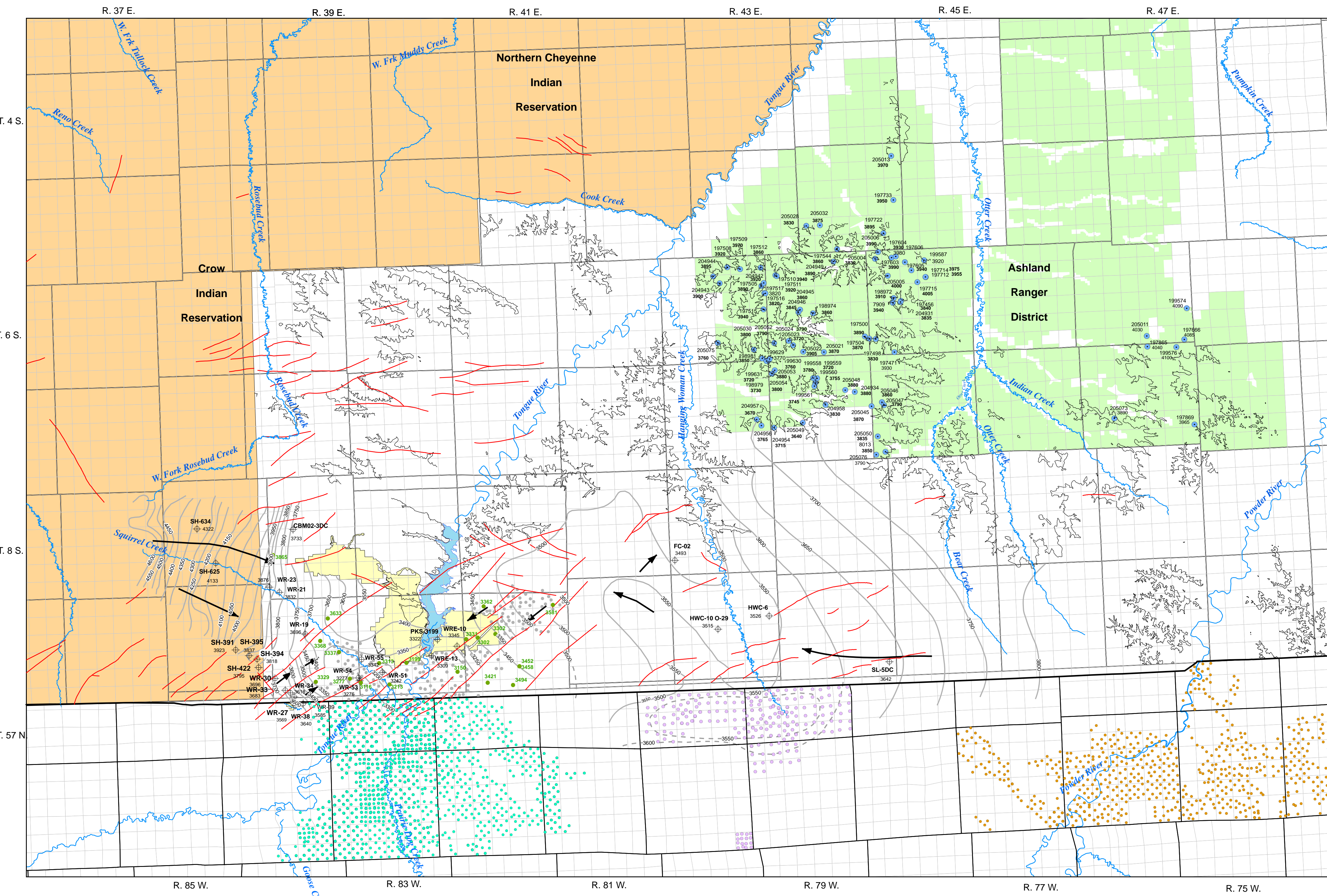
Plate 2. Potentiometric surface of the Dietz coal in the southern portion of the Powder River Basin, Montana, 2008.
