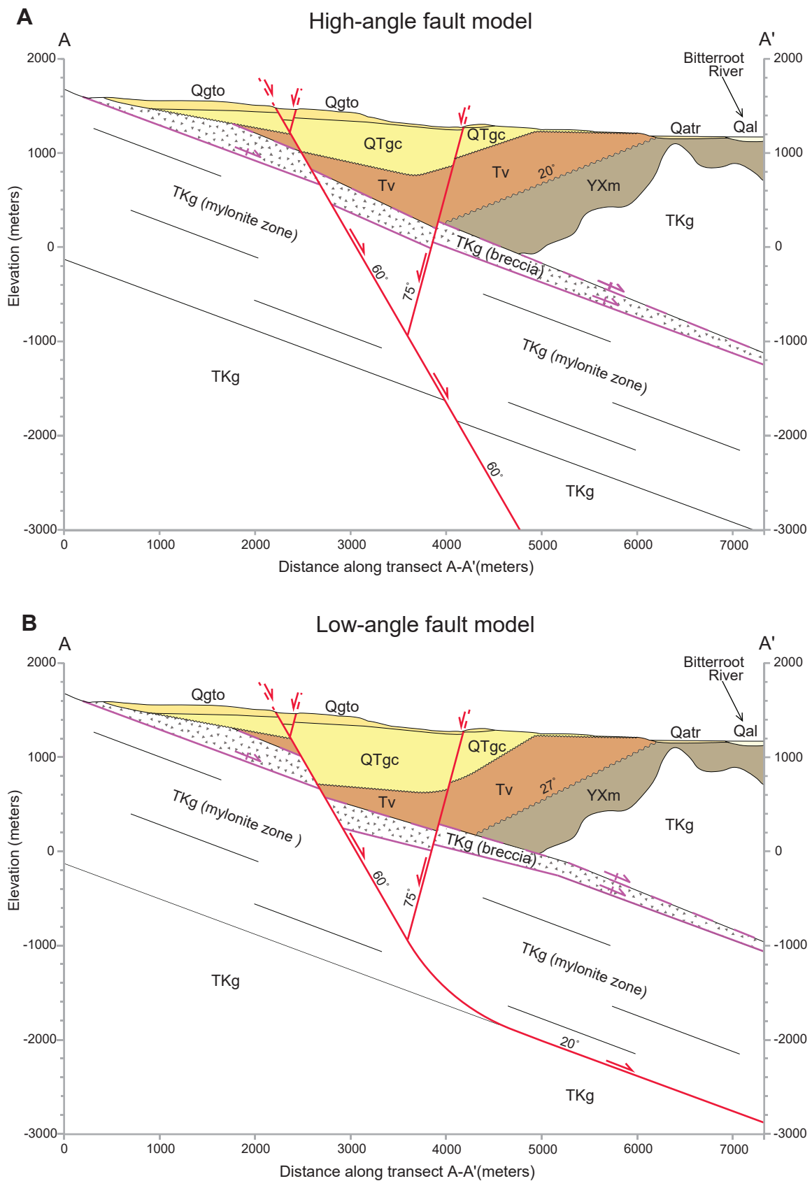
Figure 5. Structural cross-sections of the Bitterroot fault along transect A–A' showing two viable subsurface fault models that restore to the same pre-Bitterroot fault geometry: (A) high-angle fault model; (B) low-angle fault model. See figure 4 for transect location.
