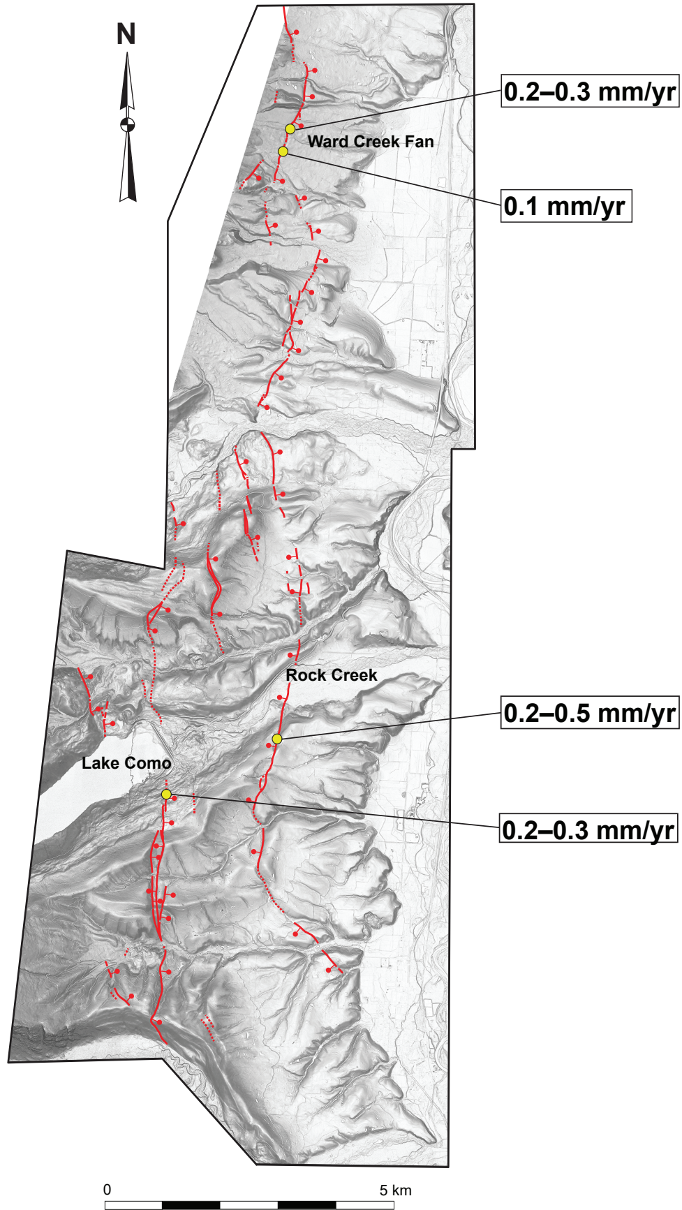
Figure 14. Slip rates distribution map along the southern Bitterroot fault showing results from our study sites (yellow). Rates on the main east-dipping fault strand range between 0.1 and 0.3 mm/yr (table 2). Slip rates on the antithetic west-dipping fault are 0.2–0.5 mm/yr, which broadly overlap with the rates on the main strand of 0.2–0.3 mm/yr for the Lake Como area.
