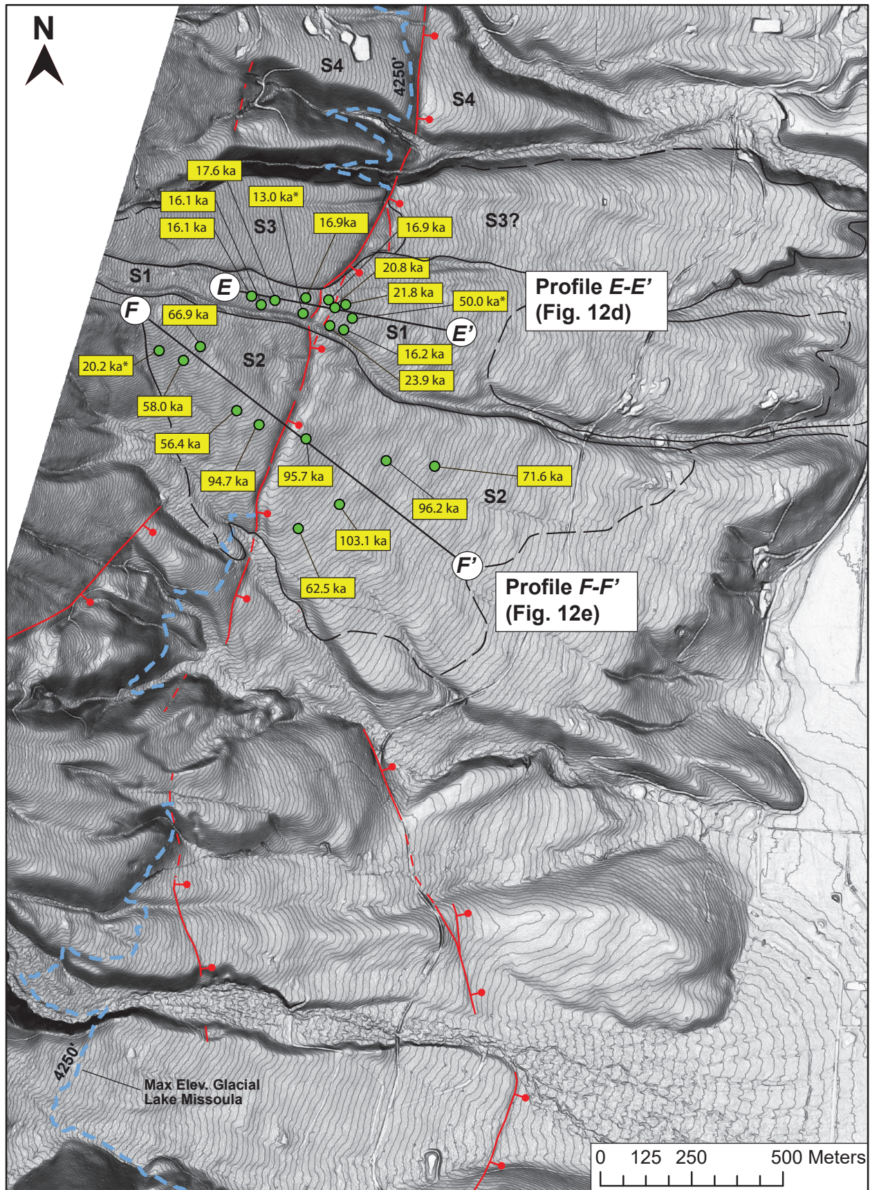
Figure 9. Detailed map of the Bitterroot fault scarps and surfaces S1–S4 at the Ward Creek fan showing cosmogenic 10 Be ages from sampled boulders. Base map is lidar slopeshade DEM with 2 m contour interval. See figure 4 for location and table 1 for age data results. S1, Pinedale young glacial debris fan (Qdfy); S2, middle-aged glacial debris fan (Qdfm); S3, middle-aged glacial debris fan (Qdfm) with bedrock pediment exposures; S4, Bedrock pediment surface with thin or no deposits preserved. *Ages interpreted as outliers based on probability density plots age models (figs. 10C, 10D).
