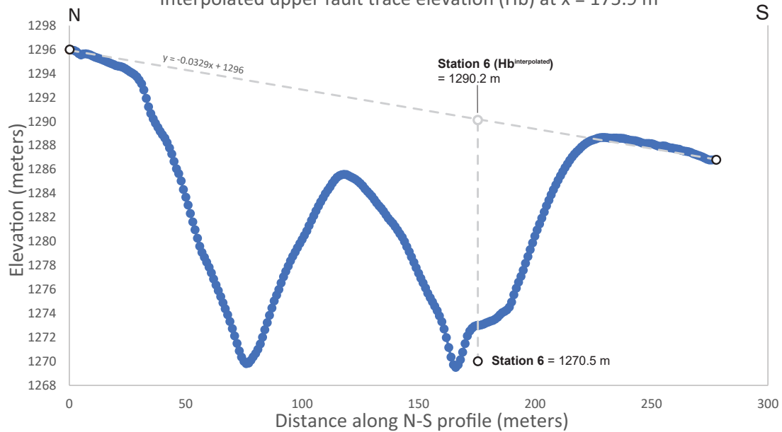
Interpolated upper fault trace elevation (Hb) at x = 175.9 m
