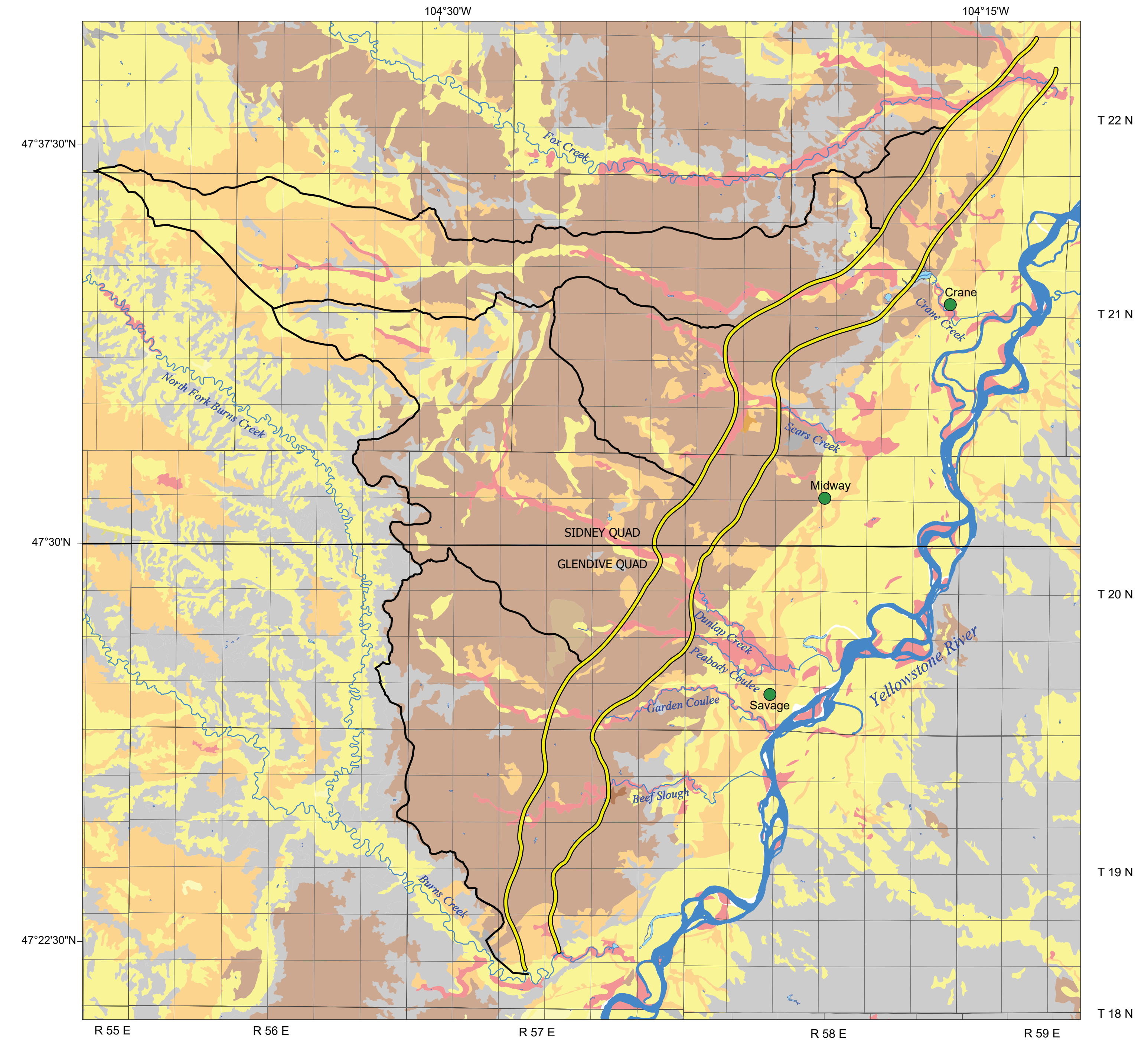
B. Geologic map based on interpretations of soil maps
