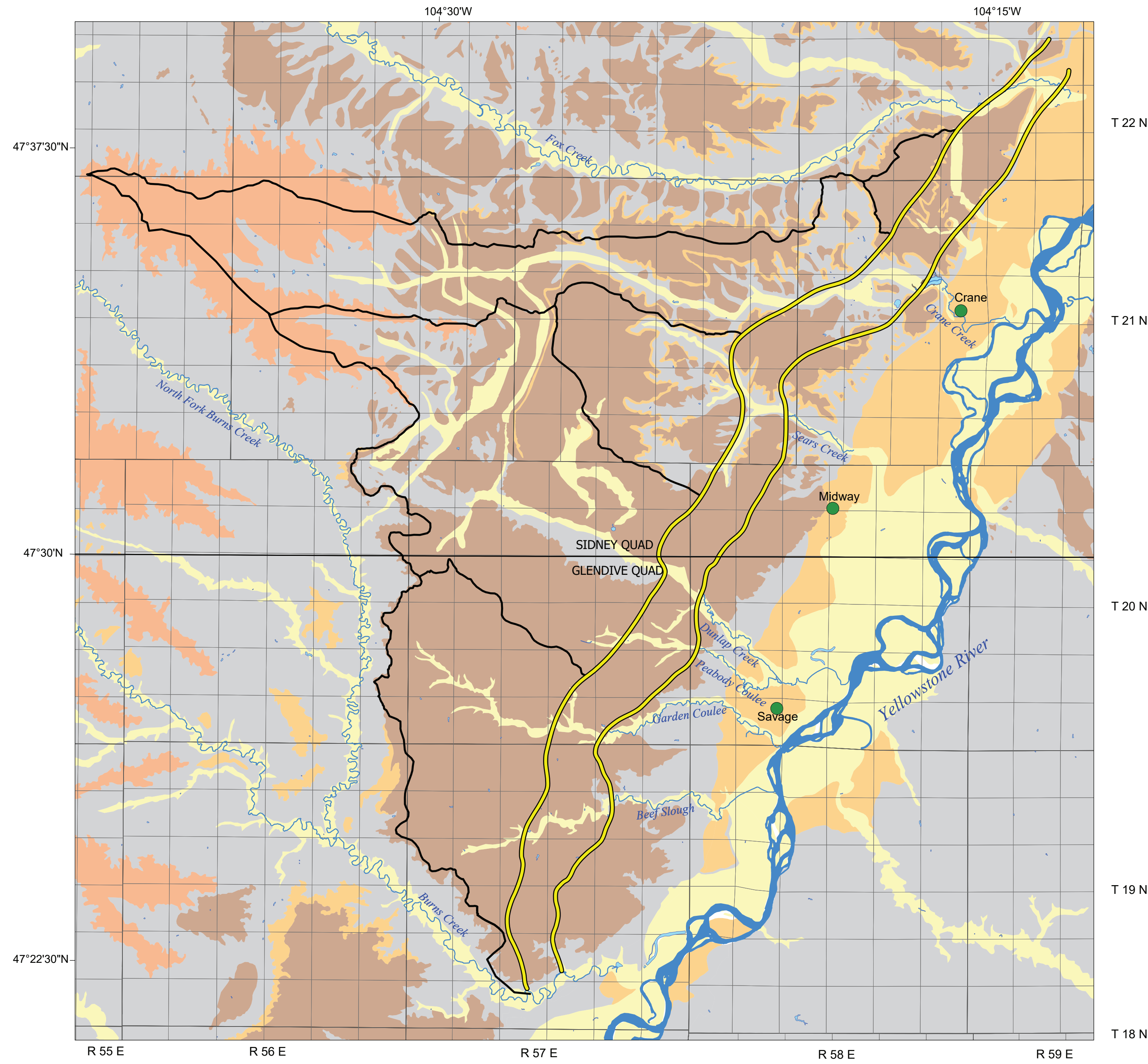
A. Geologic map based on previous geologic interpretations
