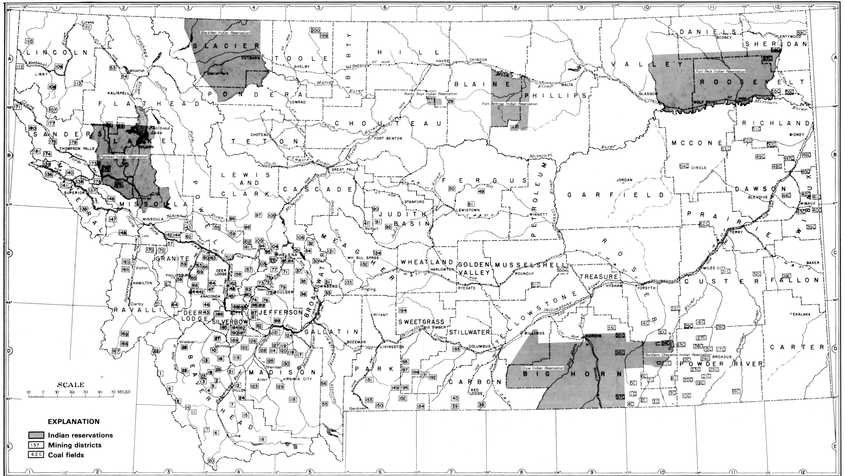
MAP SHOWING DISTRIBUTION OF MINING DISTRICTS AND STRIPPABLE COAL FIELDS IN MONTANA compiled by Uno M. Sahinen 1973 (Revised Edition)
