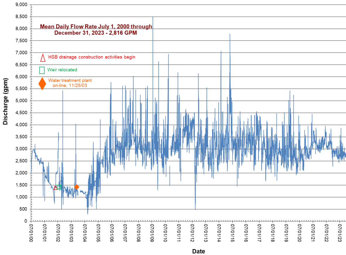
Figure 3-26. Horseshoe Bend Drainage flow rate, July 2000 through December 2023.
