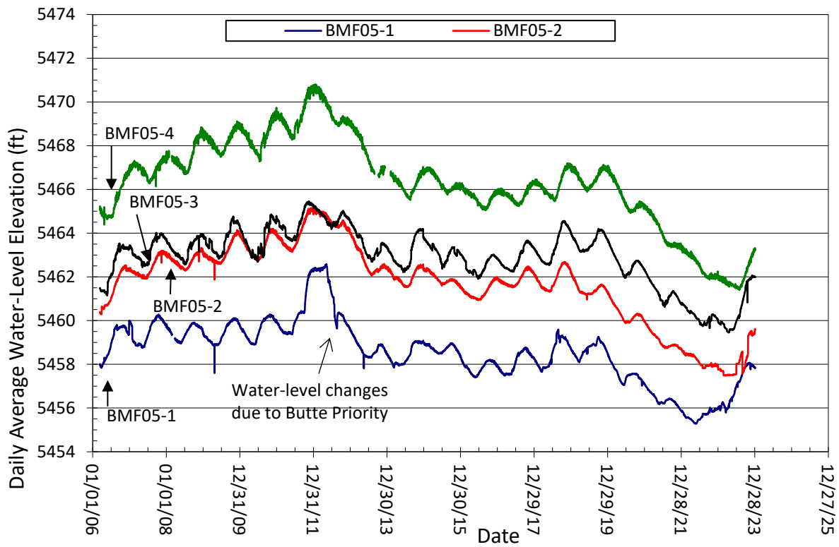
Figure 2-23. Daily average water levels for BMF05-series wells.
