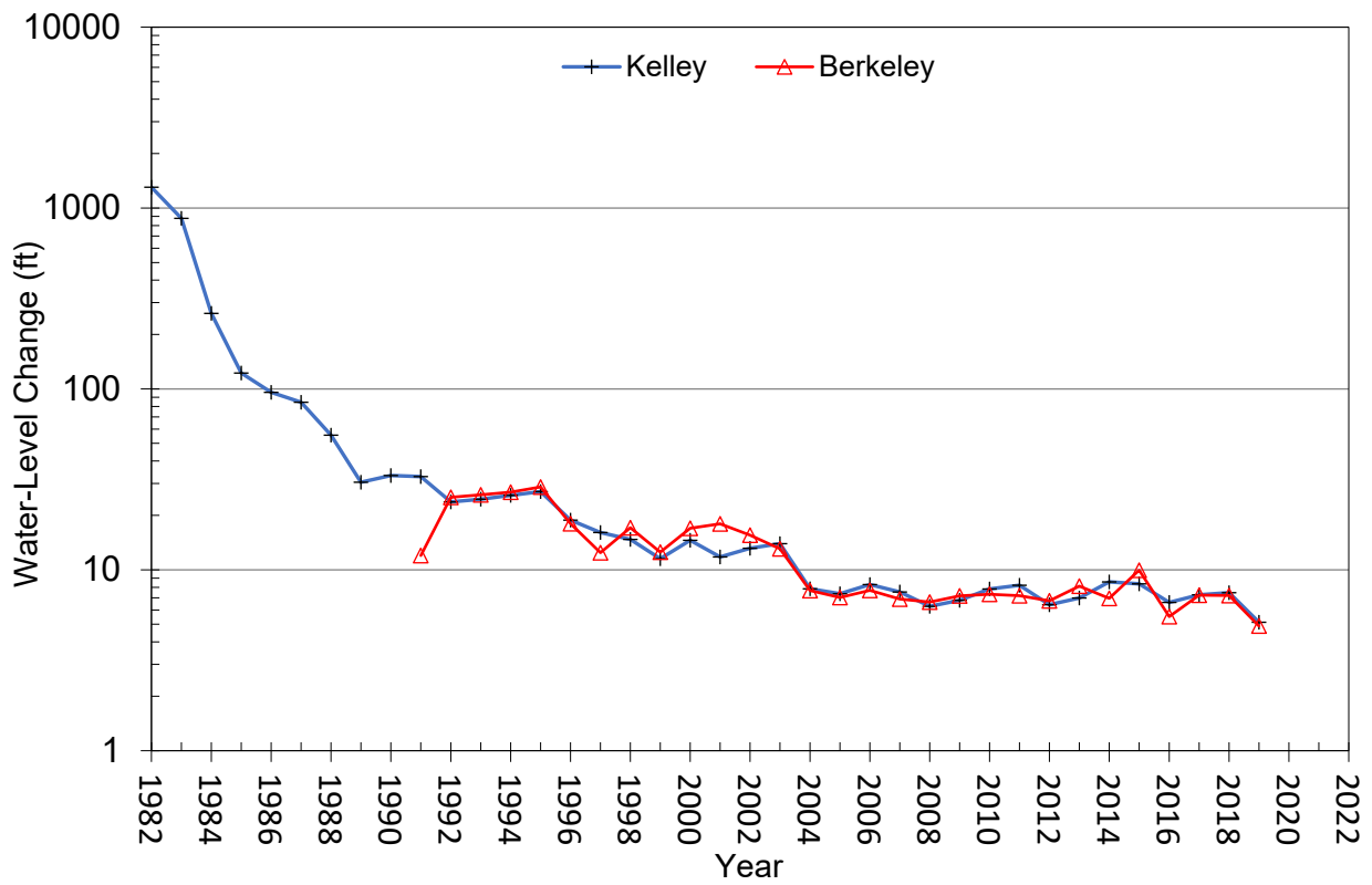
Figure 3-2A. Kelley Mine and Berkeley Pit annual water-level changes, 1982–2020.
