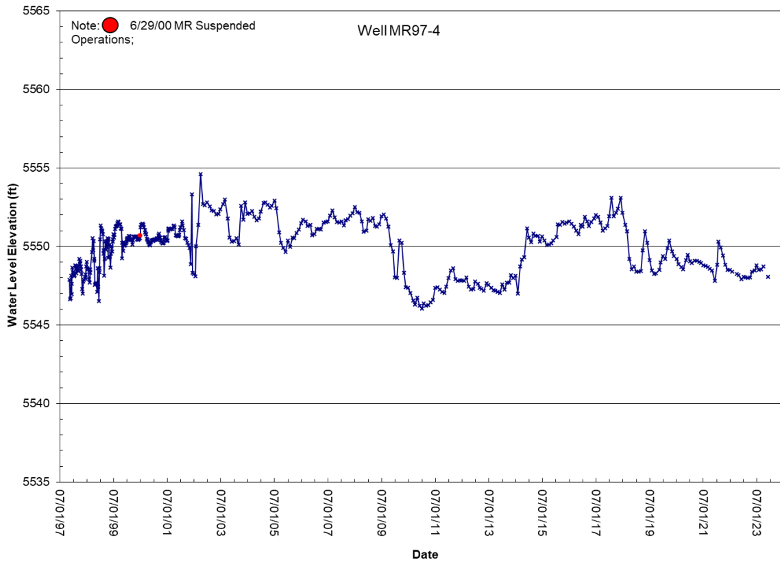
Figure 2-19. Water-level hydrograph for wells MR97-3 (top) and MR97-4 (bottom).
