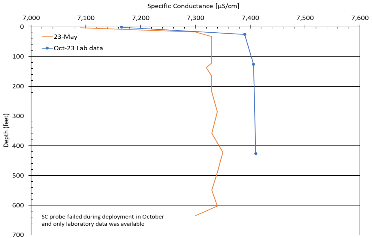
Figure 3-32. Berkeley Pit 2023 specific conductance profiles.
