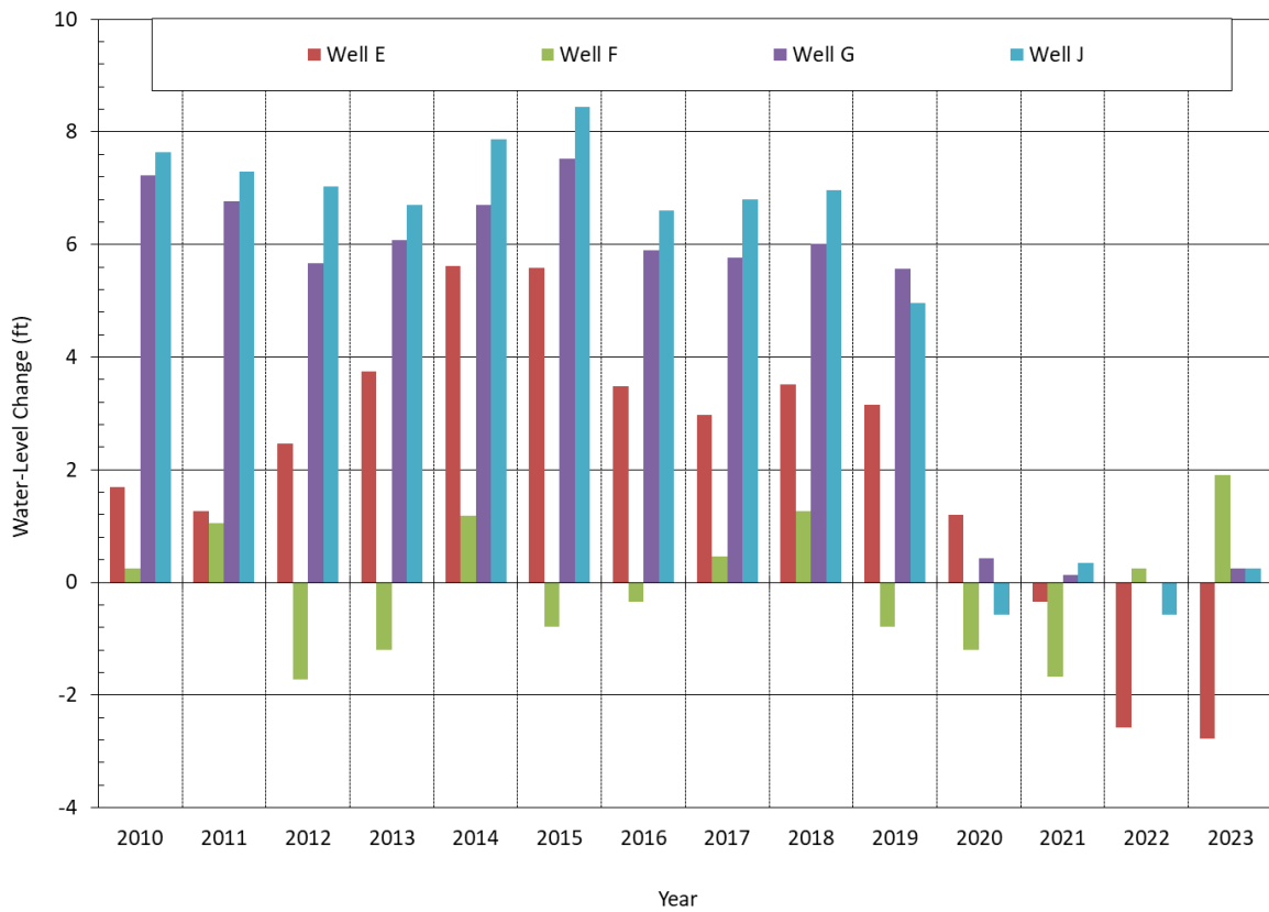
Figure 3-9. Annual water-level change in bedrock wells from 2010 to 2023.
