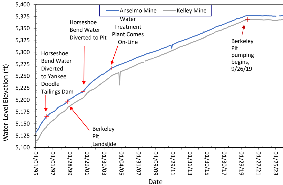
Figure 3-3. Water-level hydrograph for the Anselmo and Kelley mines from 1995 to 2023, and significant events that affected the rate of water-level rise.
