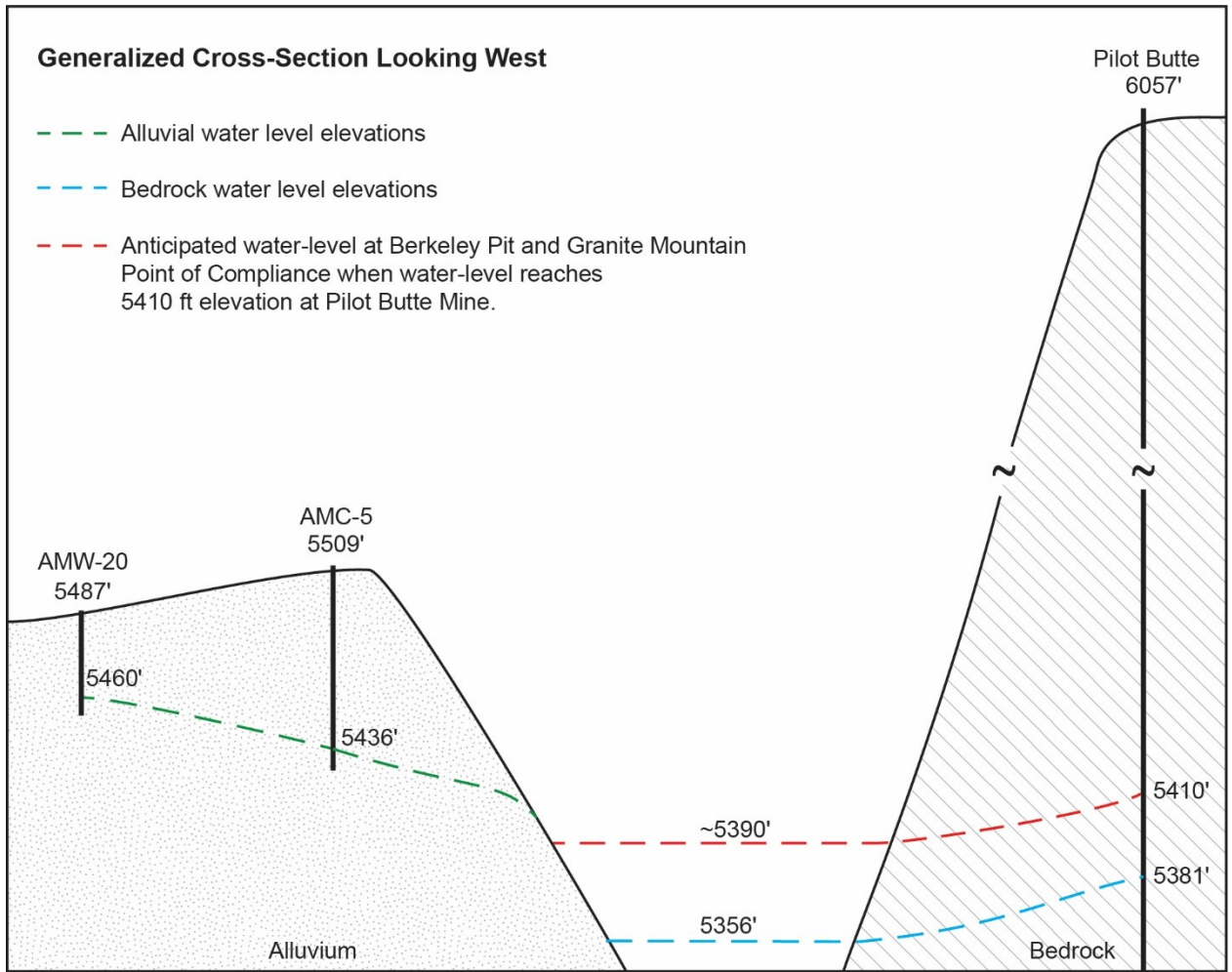
Figure 1-11. Generalized cross-section looking west through the Berkeley Pit depicting water-level elevations in bedrock and alluvial systems in December 2023 and projected elevations when the 5,410 Protective Water Elevation is reached at the Pilot Butte Mine (location shown in figure 1-10).
