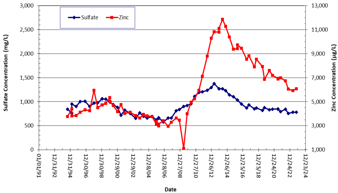
Figure 2-16. Sulfate and zinc concentrations in well LP-16.
