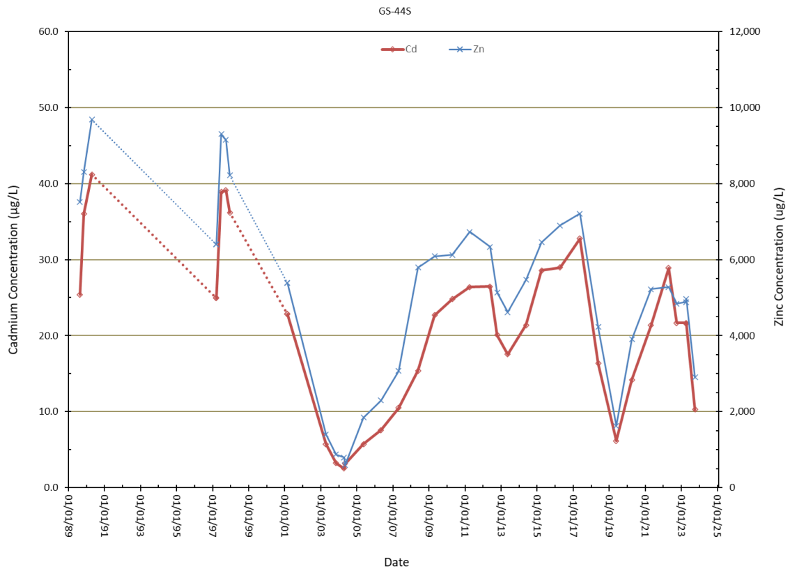
Figure 2-25. Cadmium and zinc concentration trends in well GS-44S. The DEQ-7 human health water quality standard for cadmium in groundwater is 5 µg/L, and for zinc is 2000 µg/L.
