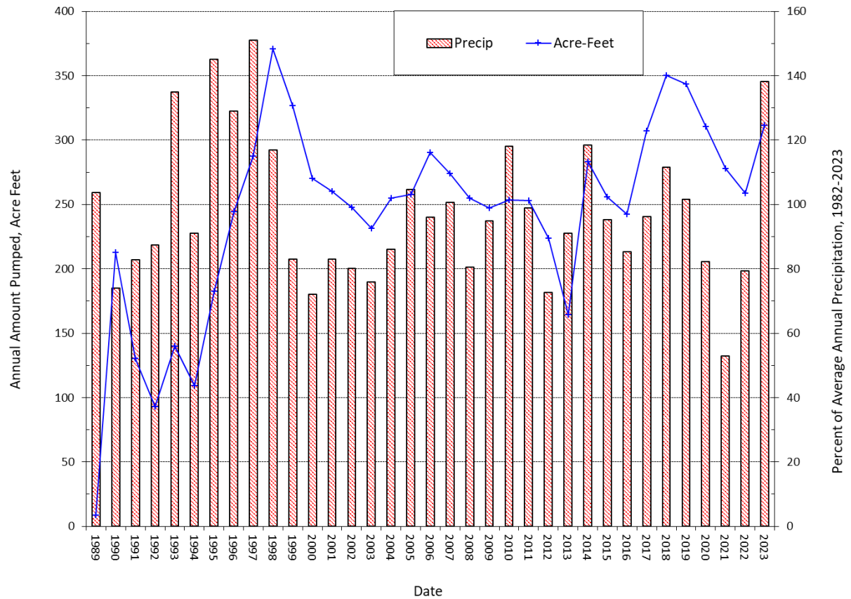
Figure 4-6. Annual amount of water pumped from the West Camp System compared to the average annual precipitation during the period 1982–2023.
