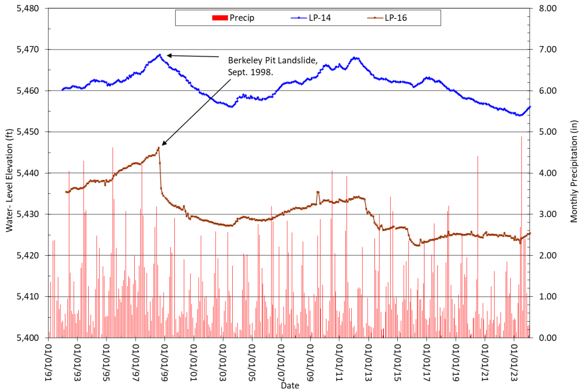
Figure 2-12. Water-level changes for wells LP-14 and LP-16 before and after the 1998 Berkeley Pit landslide.
