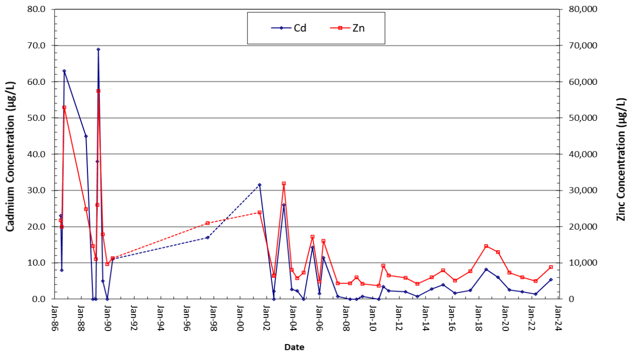
Figure 3-7. Anselmo Mine iron and arsenic concentrations (top) and cadmium and zinc concentrations (bottom) over time.
