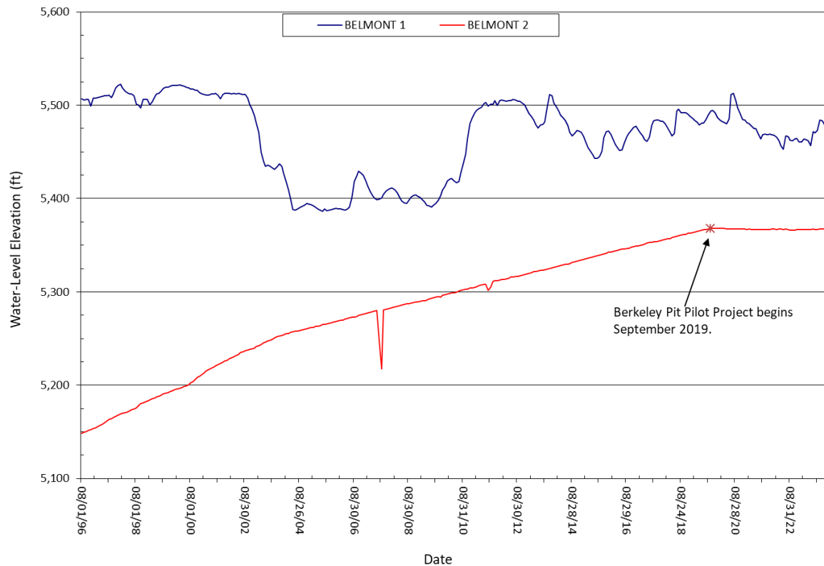
Figure 3-21. Water-level hydrograph comparisons between Belmont Well #1 and Belmont Well #2.
