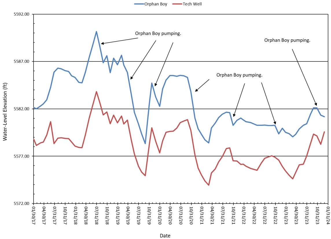
Figure 5-3. Hydrographs from Orphan Boy and Tech well show the influence of 2018–2023 Orphan Boy pumping events and monthly water-level readings, 2017–2023.
