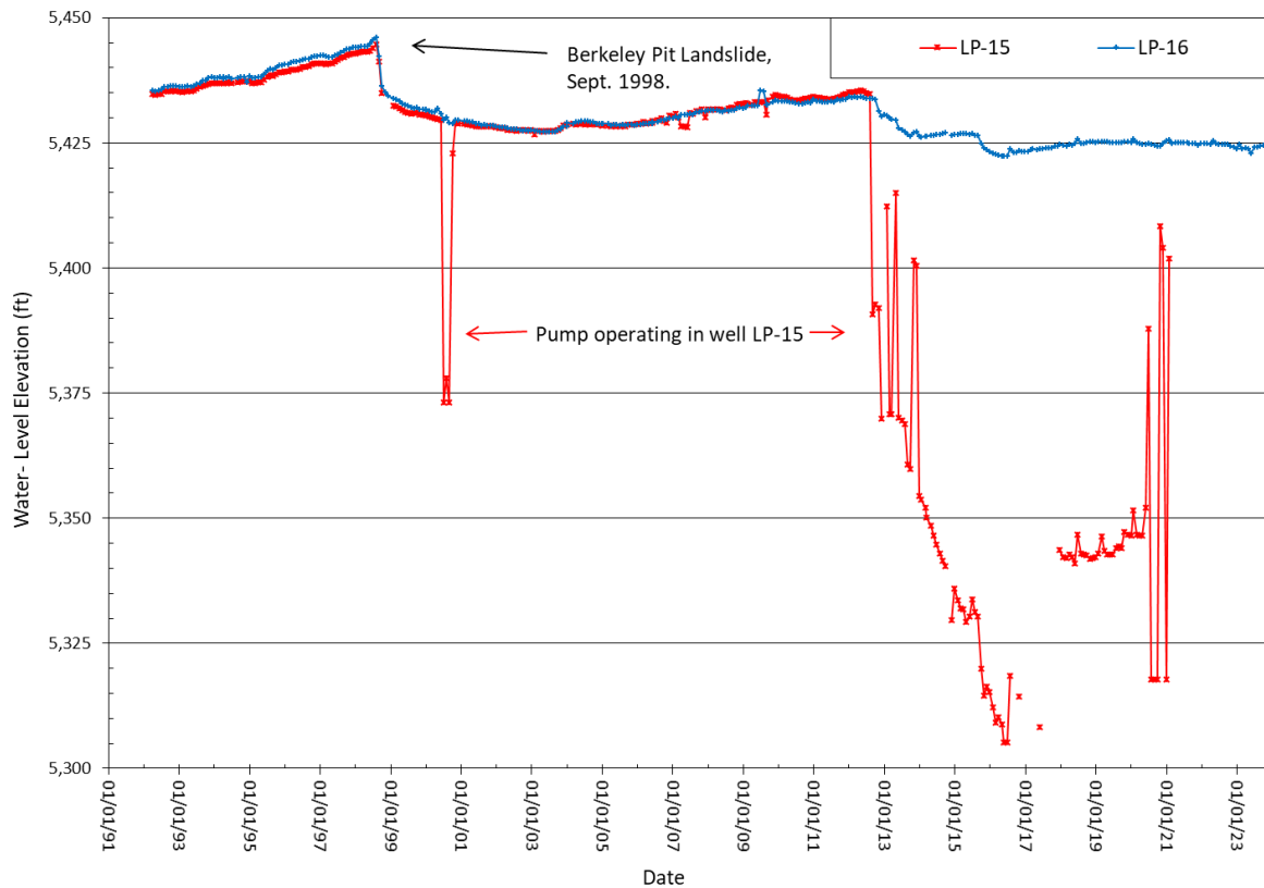
Figure 2-13. Hydrographs showing influence of dewatering on water levels in wells LP-15 and LP-16.
