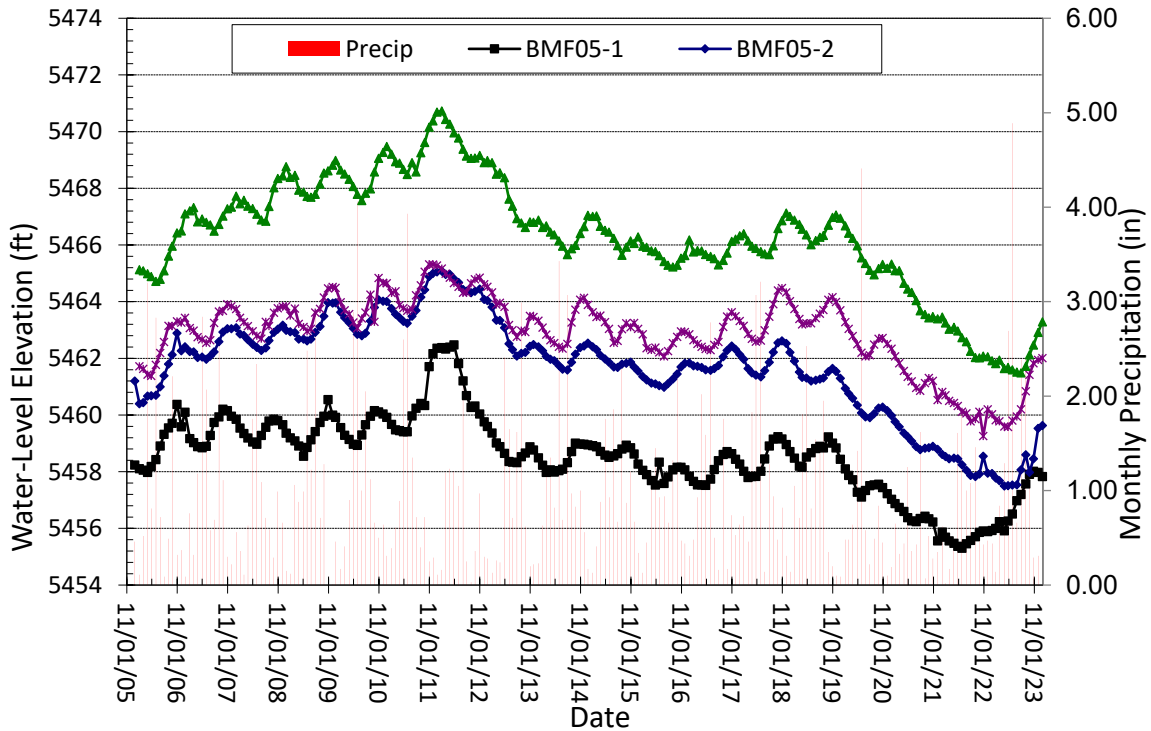
Figure 2-24. Monthly water levels versus precipitation, BMF05-series wells.
