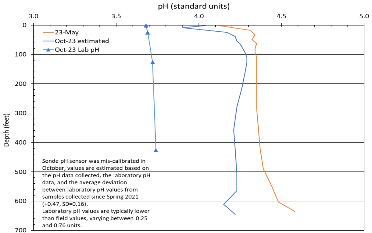
Figure 3-31. Berkeley Pit 2023 pH profiles.
