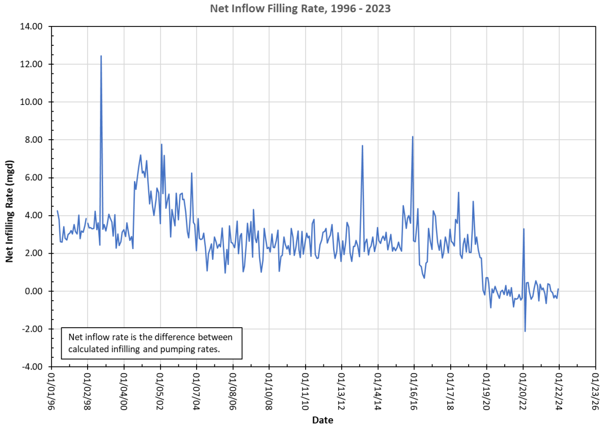
Figure 6-2. Berkeley Pit net filling rate, 1996–2023.
