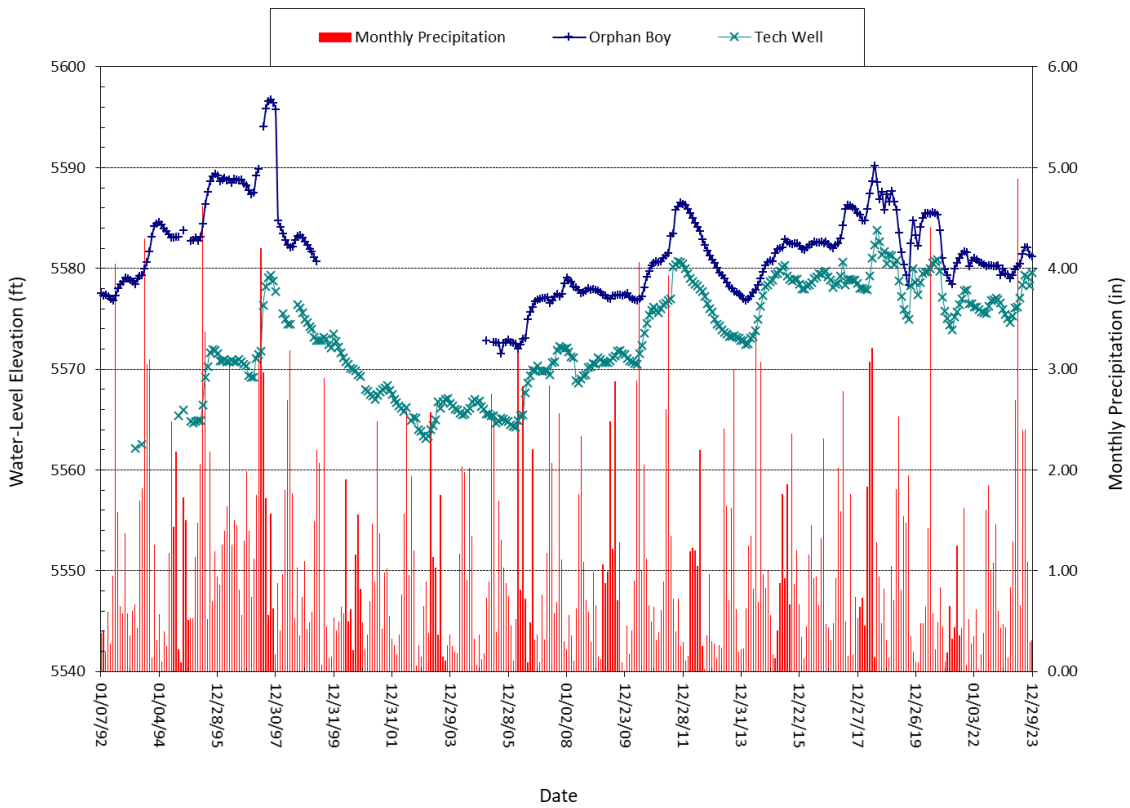
Figure 5-4. Water-level hydrograph for the Orphan Boy Mine and Montana Tech well.
