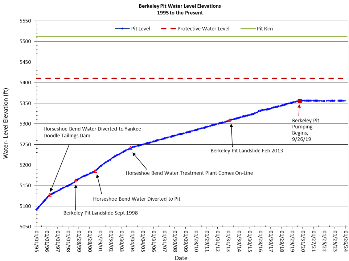
Figure 3-4. Berkeley Pit water-level hydrograph from 1995 to 2023.
