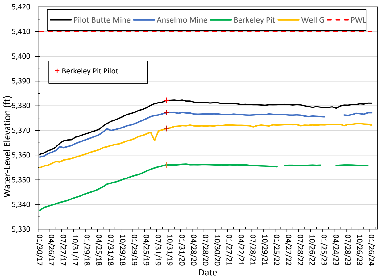
Figure 3-5. Water-level hydrograph for the Berkeley Pit and other selected bedrock monitoring sites, 2017–2023.
