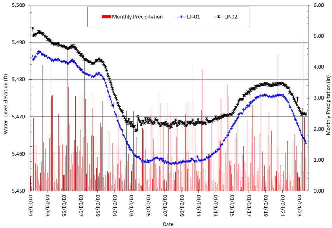
Figure 2-10. Hydrographs for wells LP-01 and LP-02 located north of the Pittsmont Waste Dump and south of the leach pads.
