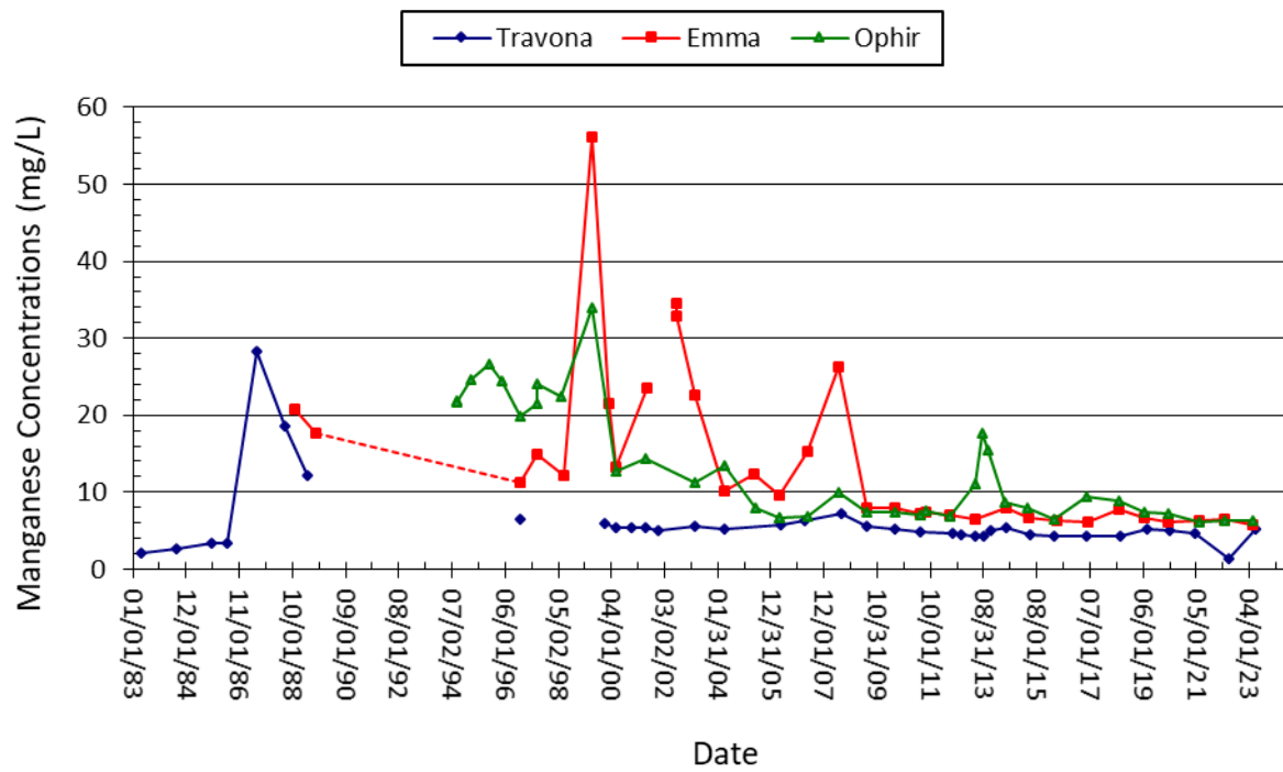
Figure 4-13. Iron (top) and manganese (bottom) concentrations in the West Camp mines.
