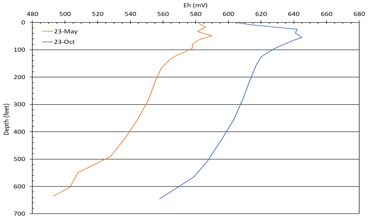
Figure 3-35. Berkeley Pit 2023 oxidation reduction profiles (Eh).
