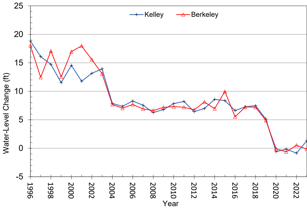
Figure 3-2B. Kelley Mine and Berkeley Pit annual water-level changes, 1996–2023.
