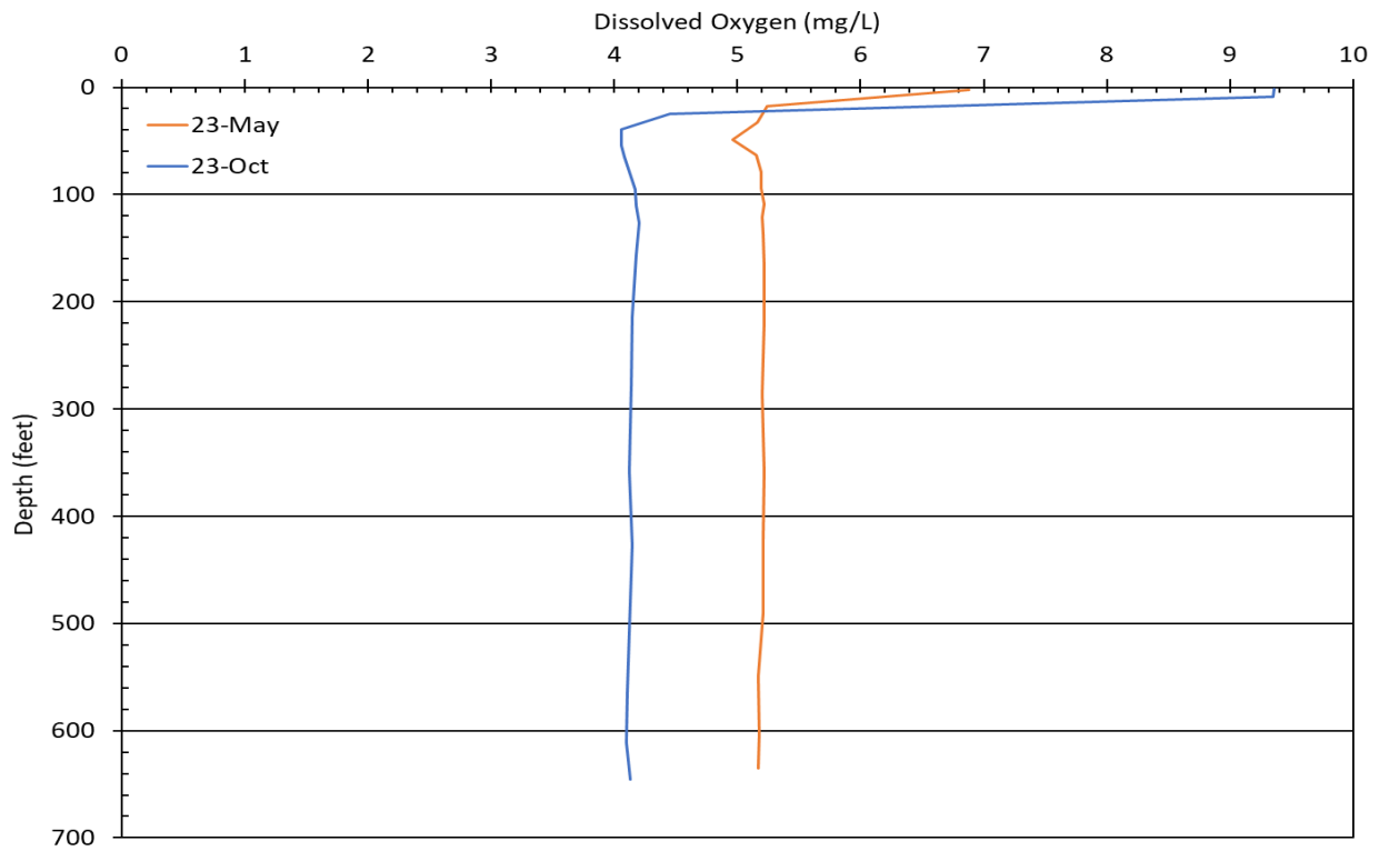
Figure 3-34. Berkeley Pit 2023 dissolved oxygen profiles.
