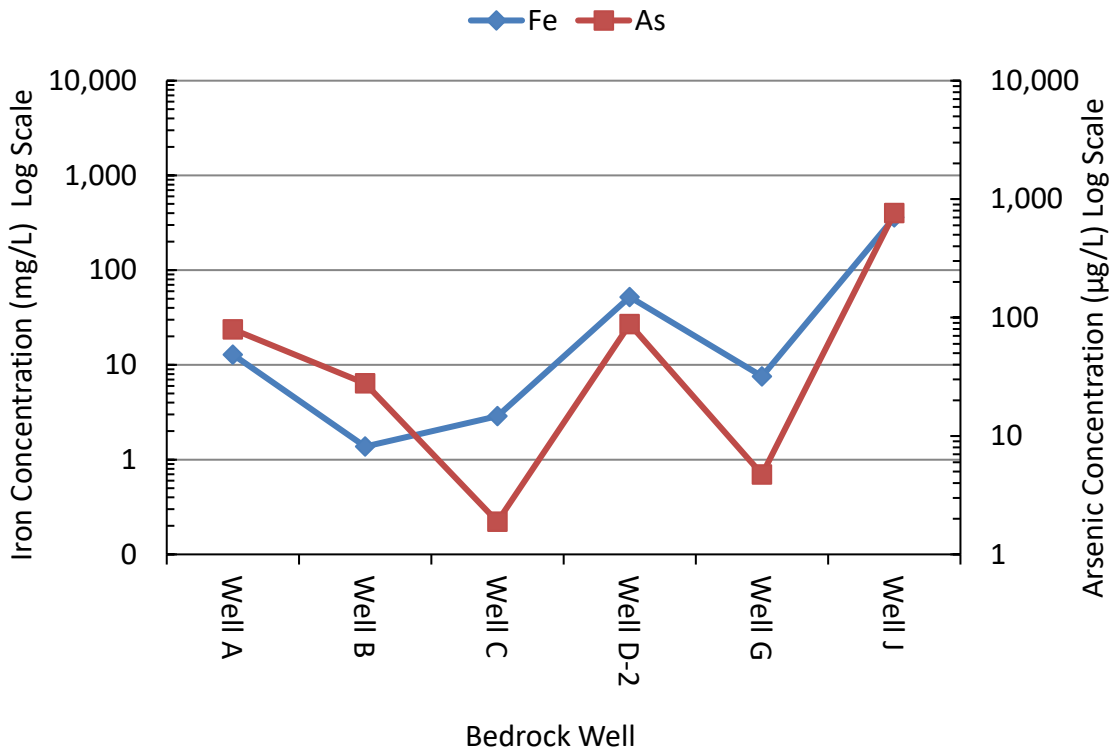
Figure 3-16. Bedrock well iron and arsenic concentration comparisons, spring 2023.
