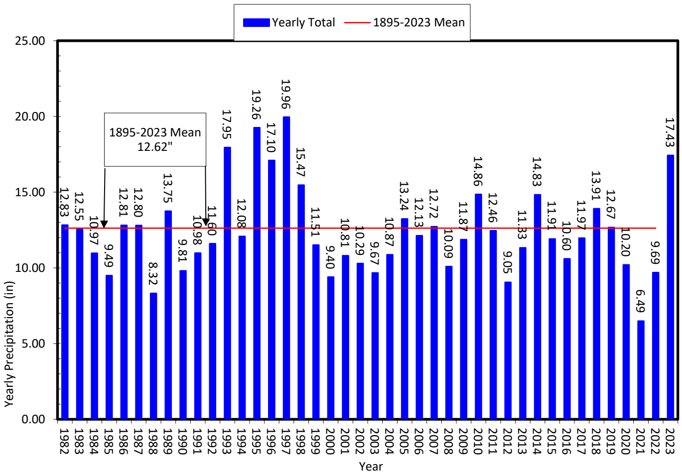
Figure 1-13. Annual precipitation totals 1982–2023, showing 1895–2023 mean.
