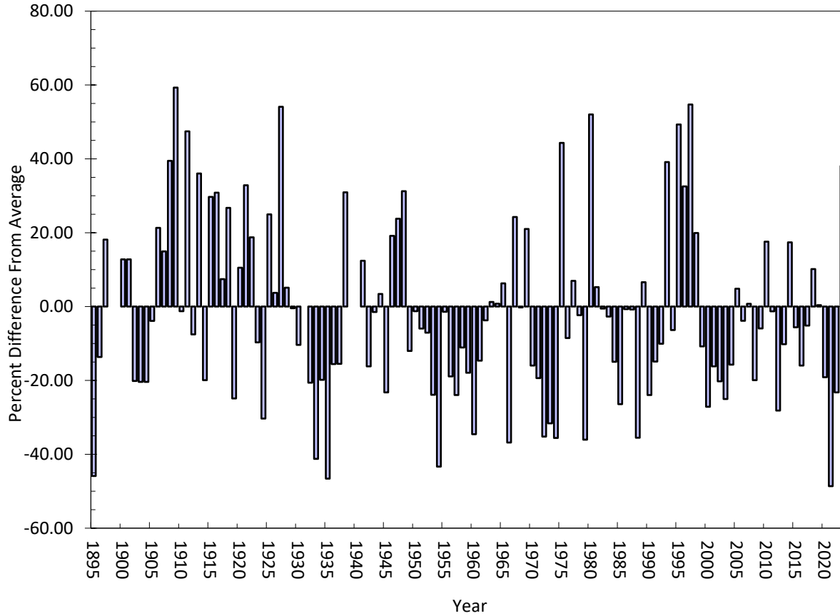
Figure 1-14. Percentage precipitation variation from normal, 1895–2023.
