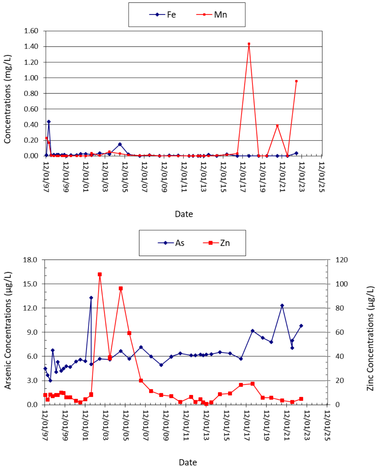
Figure 4-15. Selected water chemistry for West Camp well BMF96-4.
