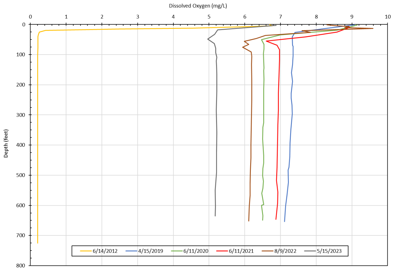
Figure 3-37. Comparison of dissolved oxygen profiles in the pit during spring 2012 and spring 2019–2023.
