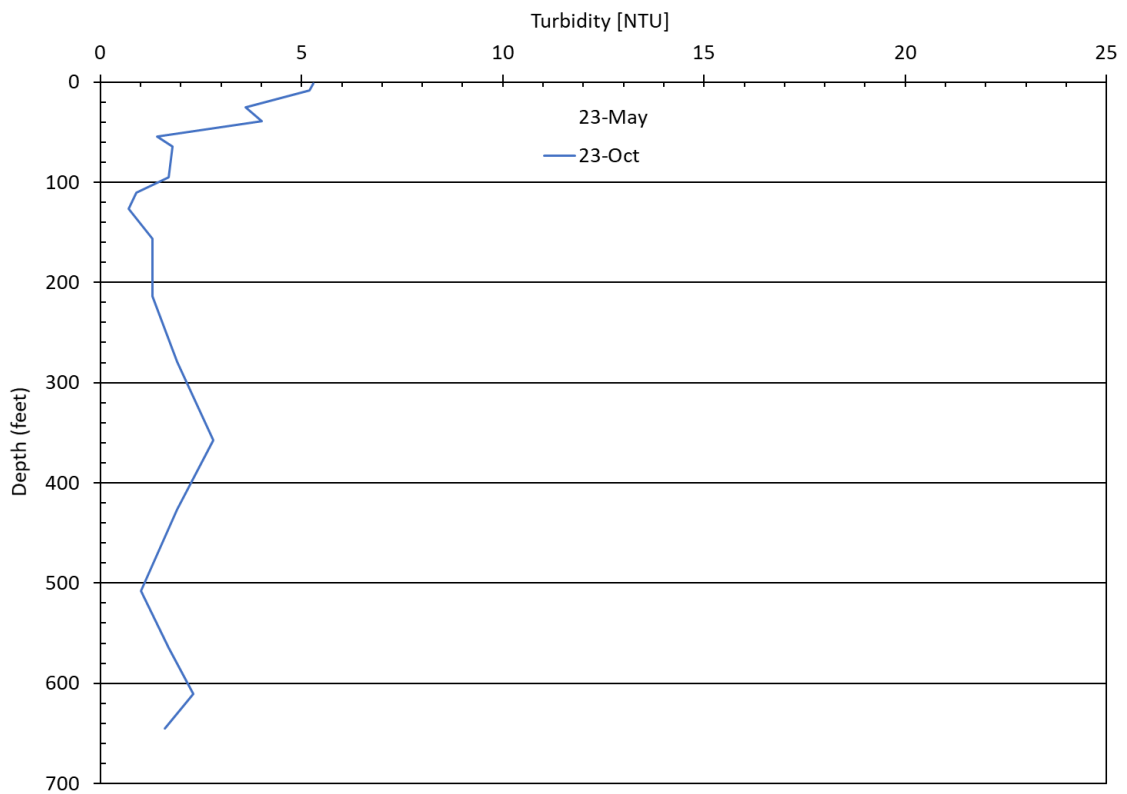
Figure 3-36. Berkeley Pit 2023 turbidity profiles. No data were collected in May due to a sensor malfunction.
