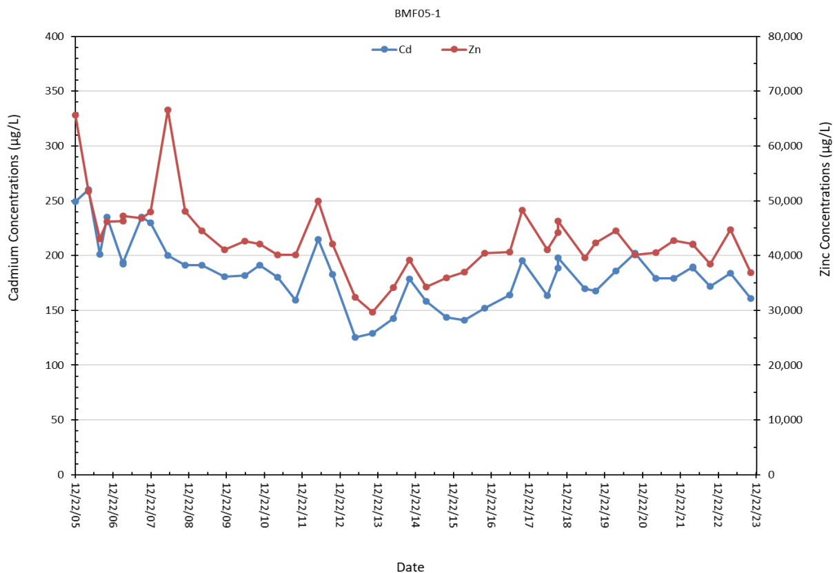
Figure 2-27. Cadmium and zinc concentration trends in well BMF05-1.
