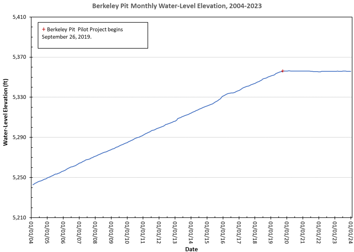
Figure 6-1. Berkeley Pit water-level elevation from 2004 through 2023. The Horseshoe Bend water-treatment plant came online in late 2003 and Horseshoe Bend water was no longer allowed to flow into the Berkeley Pit. The beginning of the Berkeley Pit Pilot Project is also shown.
