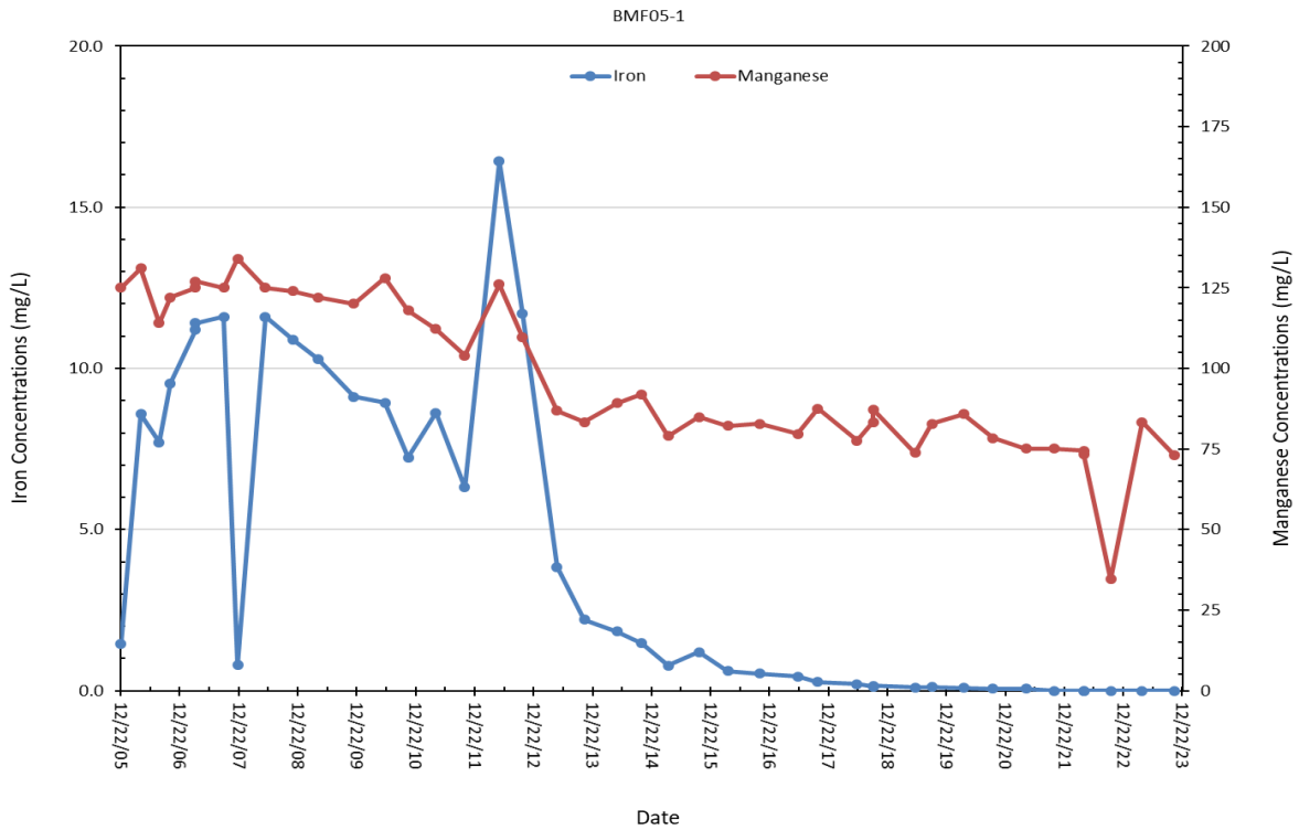
Figure 2-26. Iron and manganese concentration trends in well BMF05-1.
