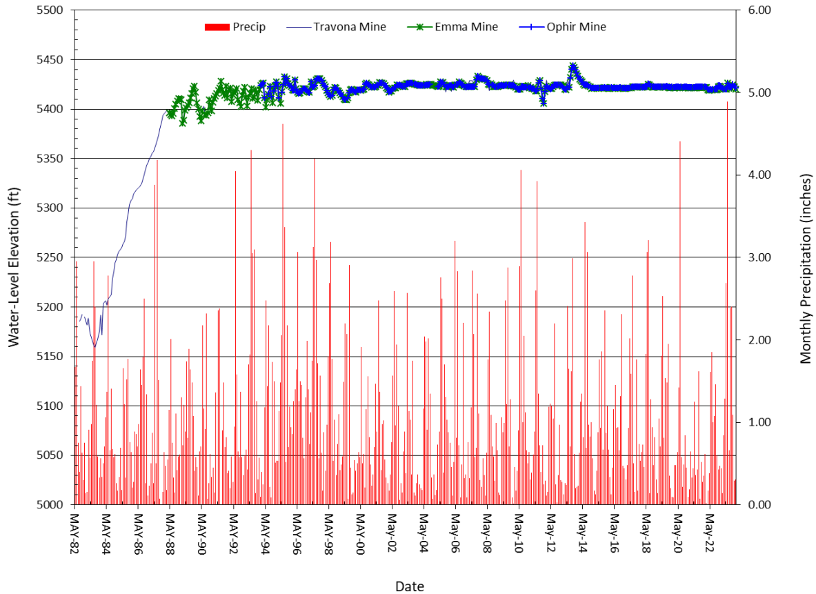
Figure 4-8. Water-level hydrographs for West Camp mines compared to monthly precipitation.
