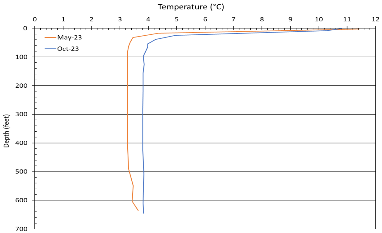
Figure 3-33. Berkeley Pit 2023 temperature profiles.
