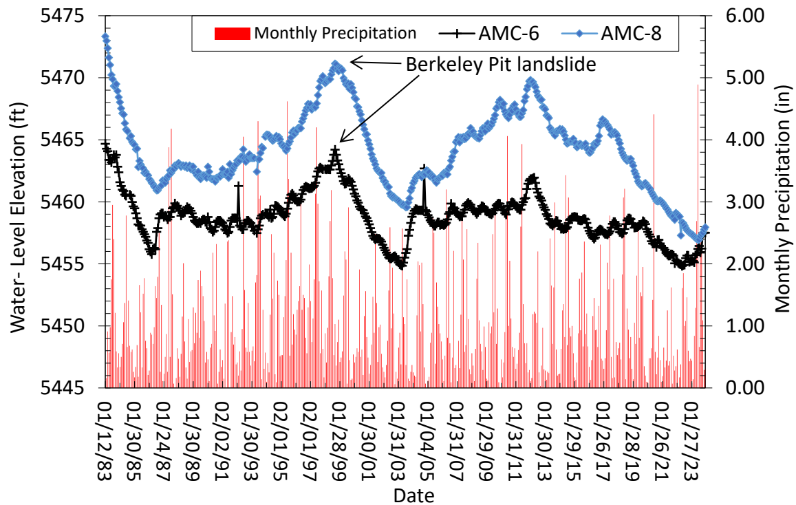
Figure 2-4. Water-level hydrographs for wells AMC-6 and AMC-8.
