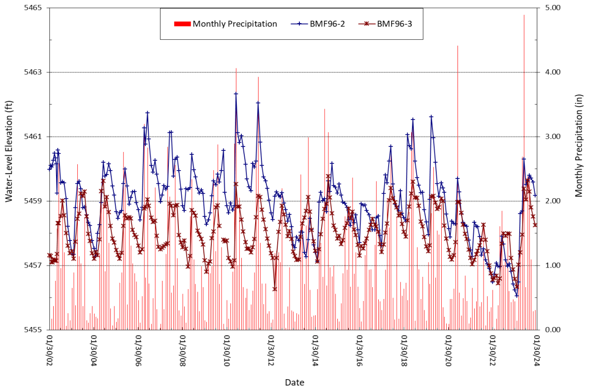
Figure 4-12. Water-level hydrographs for wells BMF96-2 and BMF96-3, 2002–2023.
