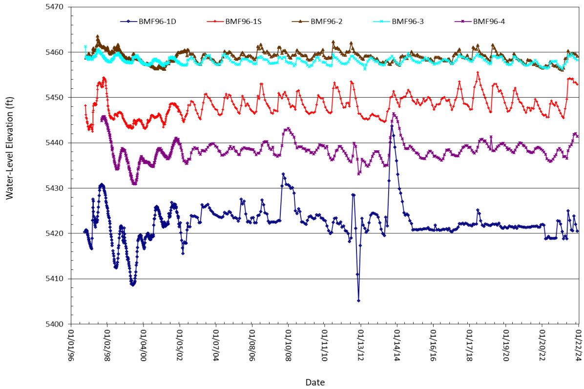
Figure 4-11. Water-level hydrographs for BMF96-series wells, 1996–2023.
