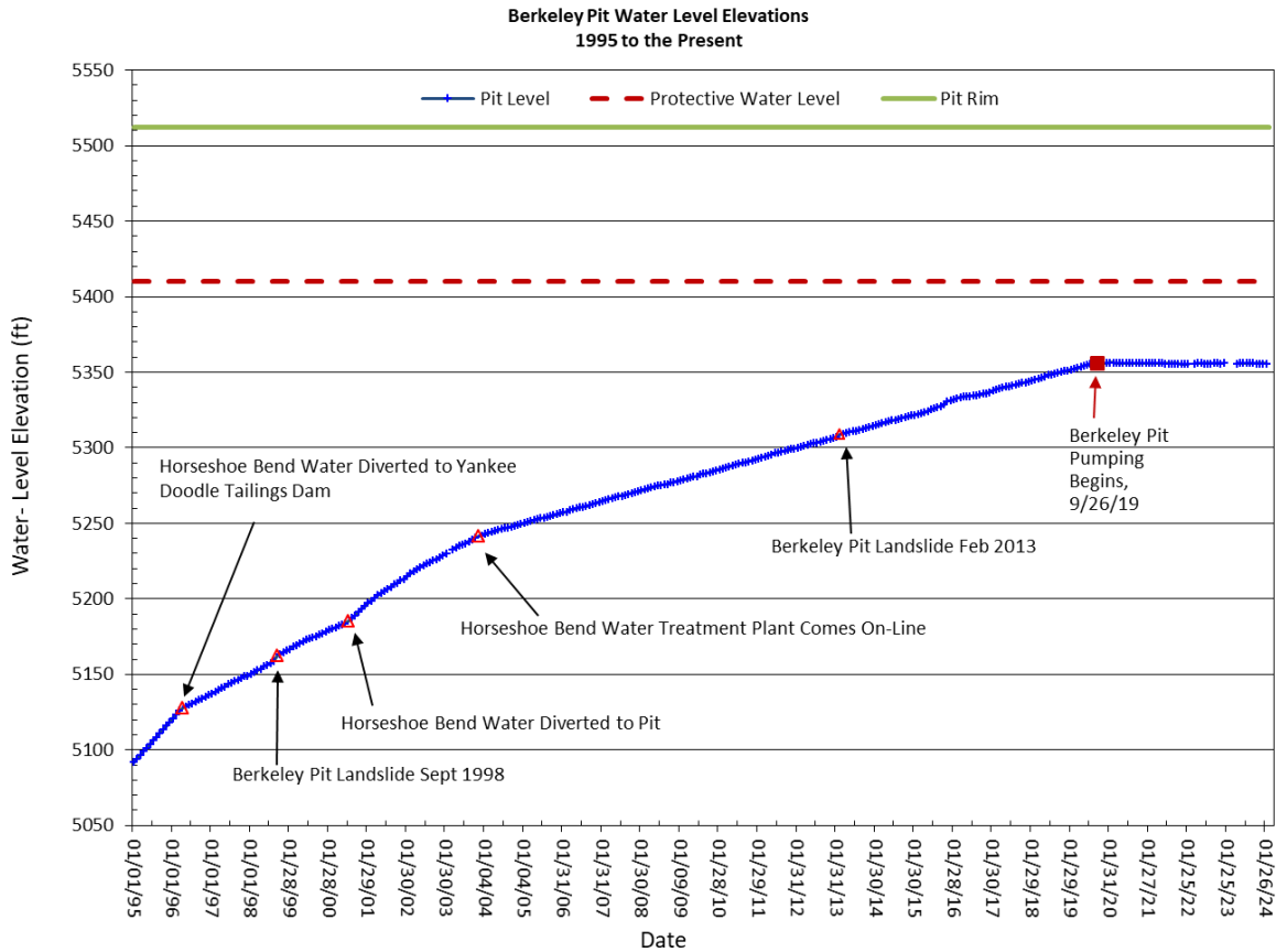
Figure 3-24. Water-level hydrograph of the Berkeley Pit, 1995–2023.
