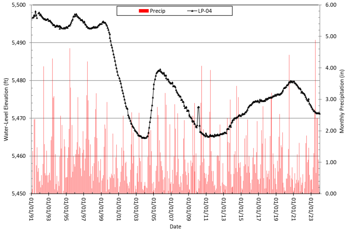
Figure 2-11. Hydrograph for well LP-04 located north of the Pittsmont Waste Dump and south of the leach pads.
