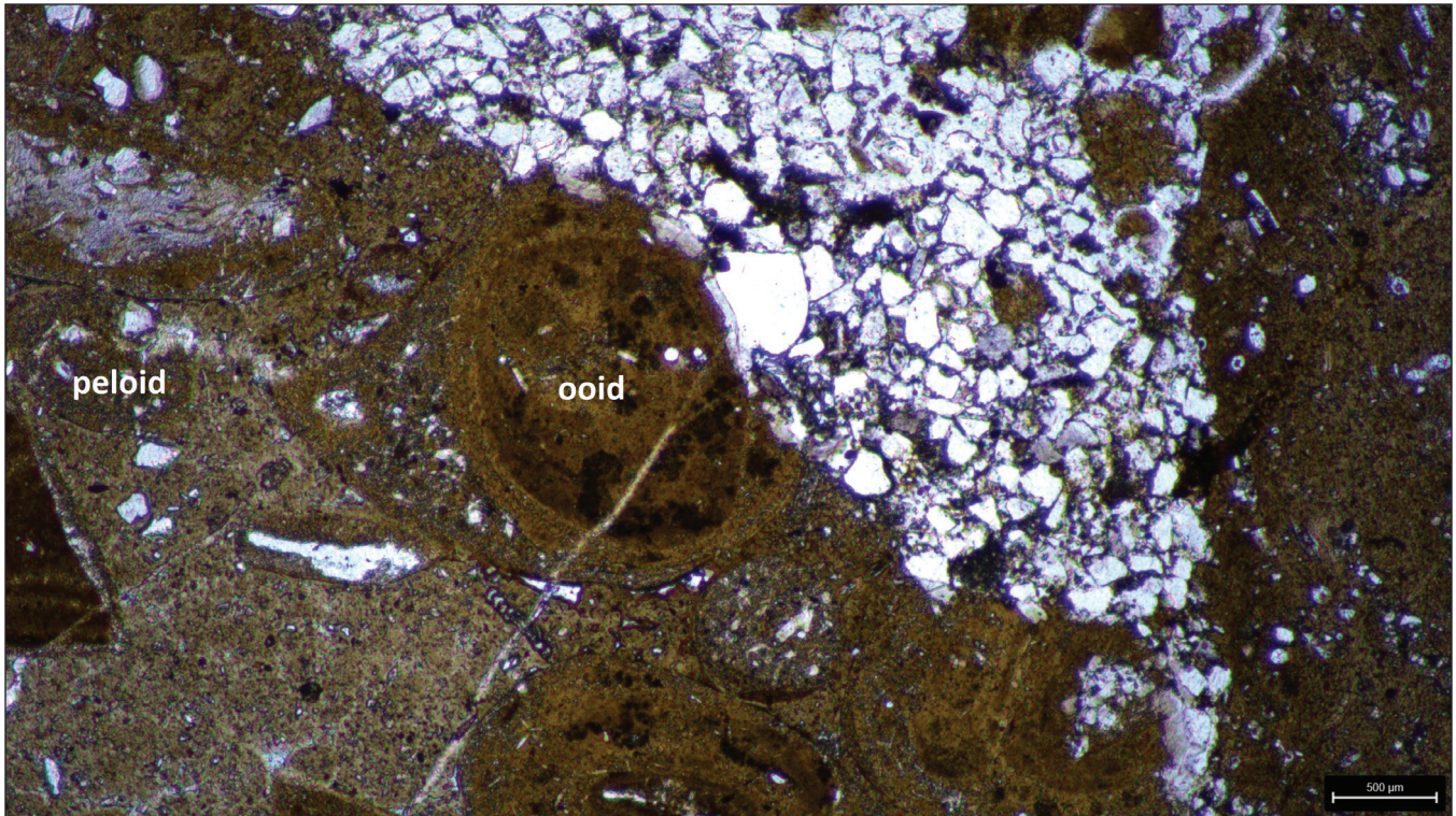
Figure 9. Plane-polarized transmitted light photomicrograph of sample ADV22PHO021: Phosphoria Formation siltstone with phosphorite clasts showing ooids and peloids (examples labeled).
