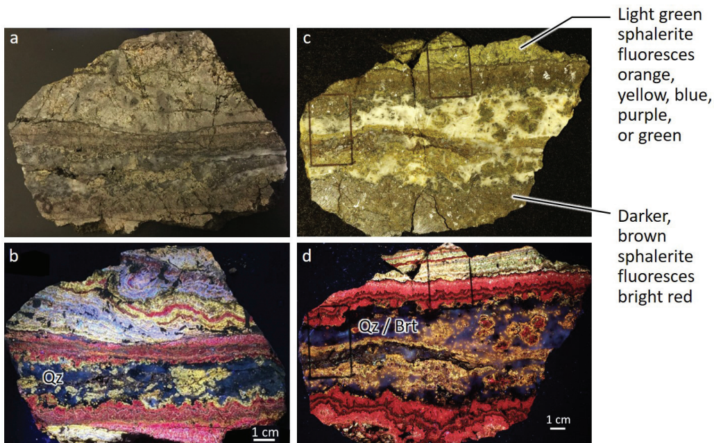
Figure 3. Samples from the Philipsburg mining district showing the two main types of sphalerite, light green and brown, and their respective fluorescence. Everything is sphalerite unless noted otherwise: Qz, quartz; Brt, barite. (a) CB-SA-04 under visible light; (b) CB-SA-04 under long-wave UV light; (c) CB-TF-01 under visible light; (d) CB-TF-01 under long-wave UV light.
