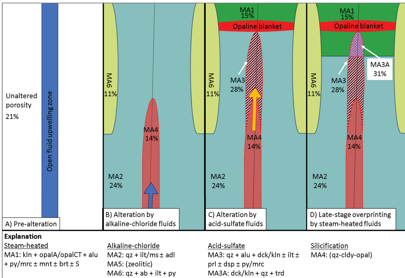
Figure 5. Schematic diagram of the progression of hydrothermal alteration with changes to mean porosity. (A) Pre-alteration. Unaltered Tuff of Sulphur Creek with an open conduit, shown in blue, and a mean porosity of 21%. (B) Alteration by alkaline-chloride fluids. Mineral assemblages (MA) associated with alkaline-chloride fluids, excluding MA5. Each color matches the color scheme used in Figure 2. The black line represents an open fracture or conduit for altering fluids (blue arrow) to follow. MA2 (light blue) alteration produces a moderate porosity increase to 24%. The pale green shoulders, MA6, are distal expressions with an 11% porosity. The red portion along the conduit is silicification, lowering porosity. (C) Alteration by acid-sulfate fluids. Influx of acid-sulfate fluids (orange arrow with red outline) produces MA3. MA3 alteration (pink with black lines) increased porosity to 28%. The appearance of MA1 (green) implies a lowering of the water table to allow the production of a steam-heated zone. The red blanket at the bottom of MA1 represents the deposition of opaline silica. (D) Late-stage overprinting by steam-heated fluids. Altering fluids stopped rising along the conduit, and the local water table continues to fall, expanding MA1 and overprinting MA3 to produce MA3A (purple with white cross-hatching).
