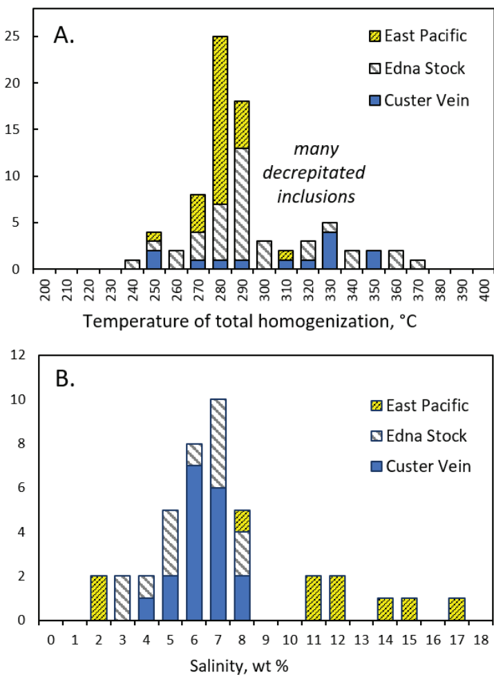
Figure 10. Histograms of fluid inclusions data: (A) total homogenization temperature; (B) salinity, wt% NaCl eq . The histogram columns in panel A are underrepresented for T > 300°C due to decrepitation of many CO 2 -rich inclusions prior to reaching the final homogenization temperature.
