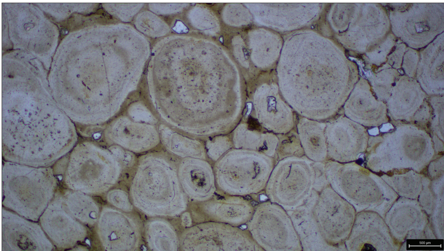
A plane-polarized transmitted light photomicrograph of weakly metamorphosed oolitic phosphorite from the Gravelly Mine, Powell County, Montana.
