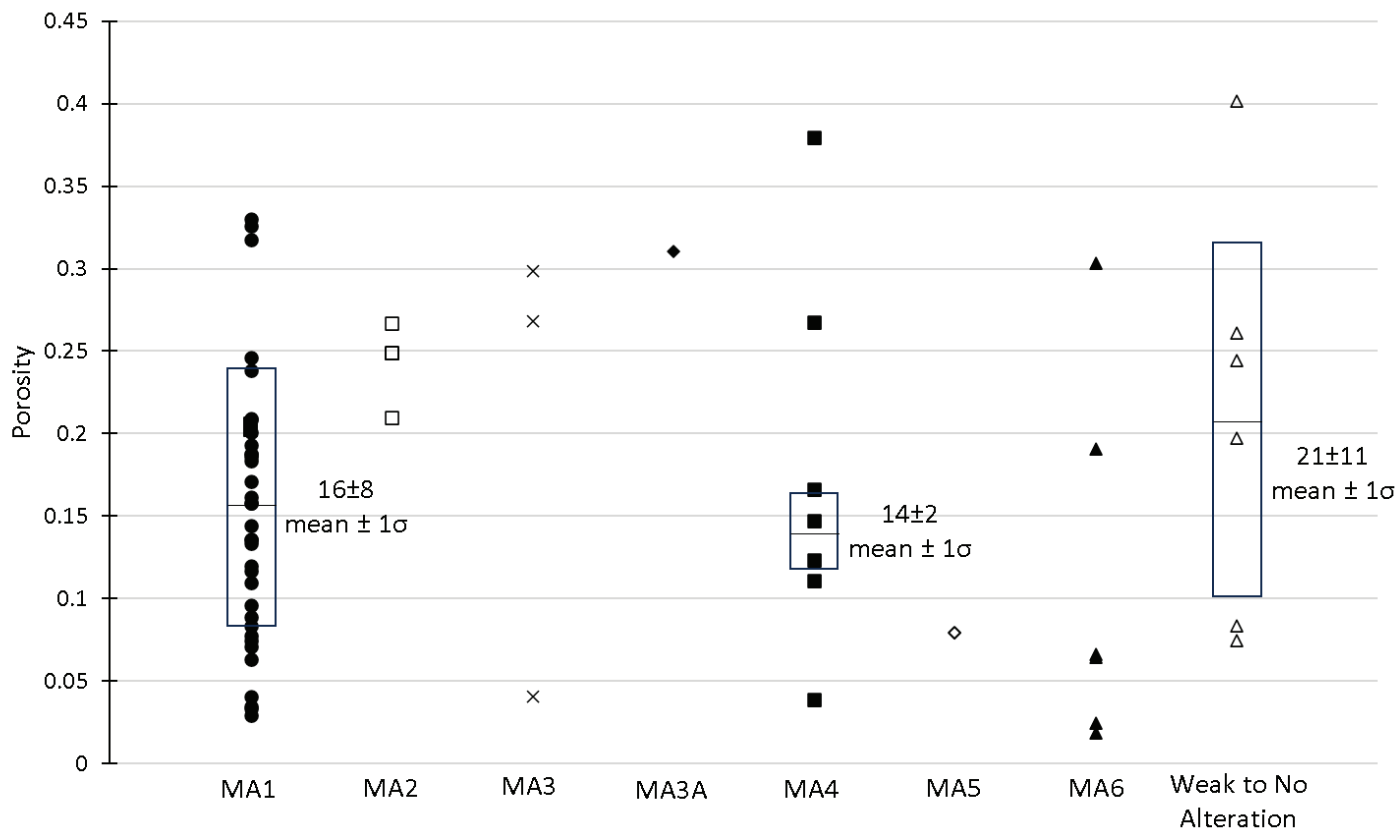
Figure 3. Porosity separated based on mineral assemblages in altered tuff and tuff with weak to no alteration. The general spread of porosity is similar between the alteration mineral assemblages. However, mean porosity values for MA1 (steam-heated alteration) and MA4 (silicification) are lower than tuff with weak to no alteration, indicating hydrothermal fluids are generally decreasing porosity in those mineral assemblages.
