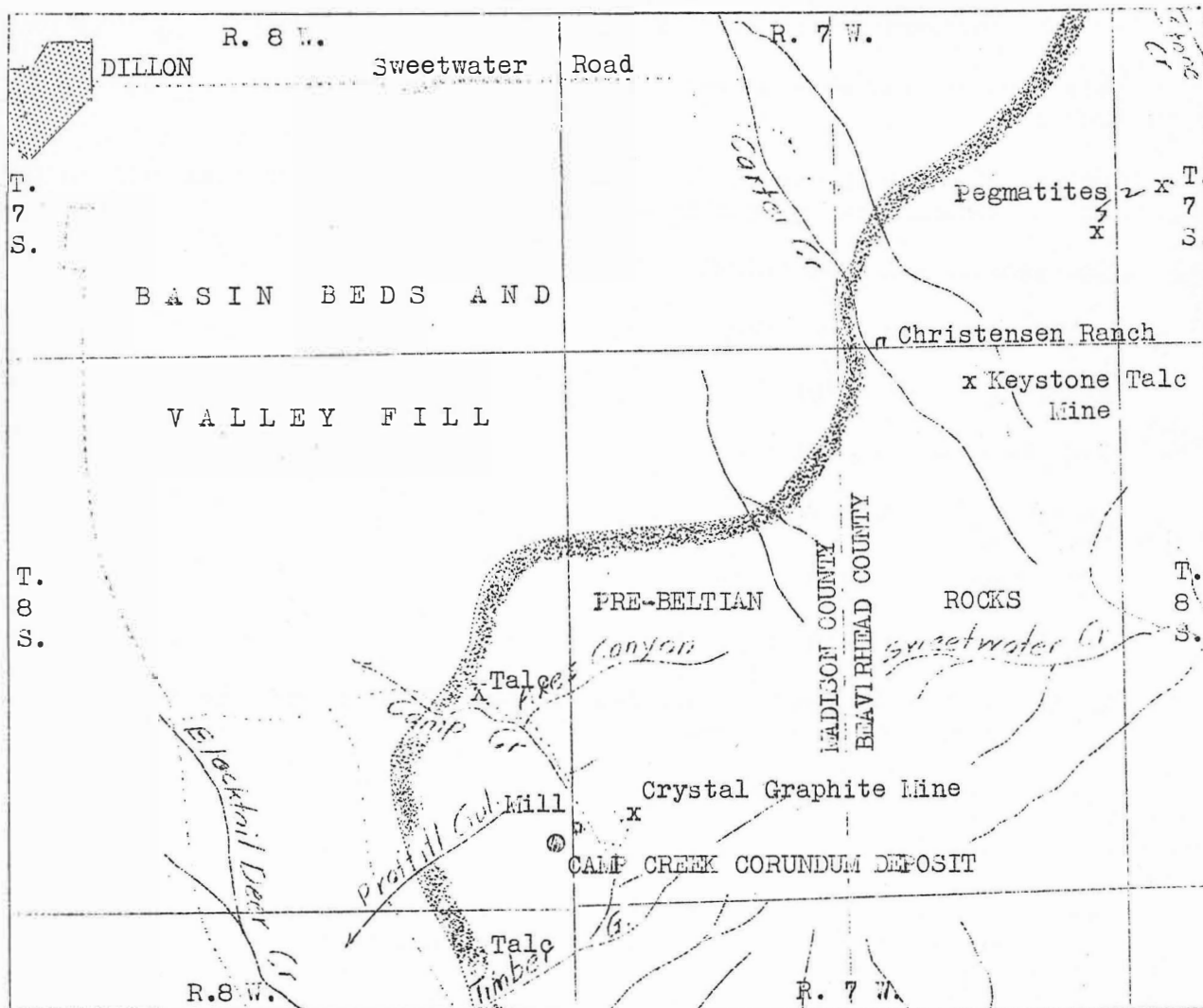
Figure 1.--Index map showing location of Camp Creek corundum deposit, Montana
