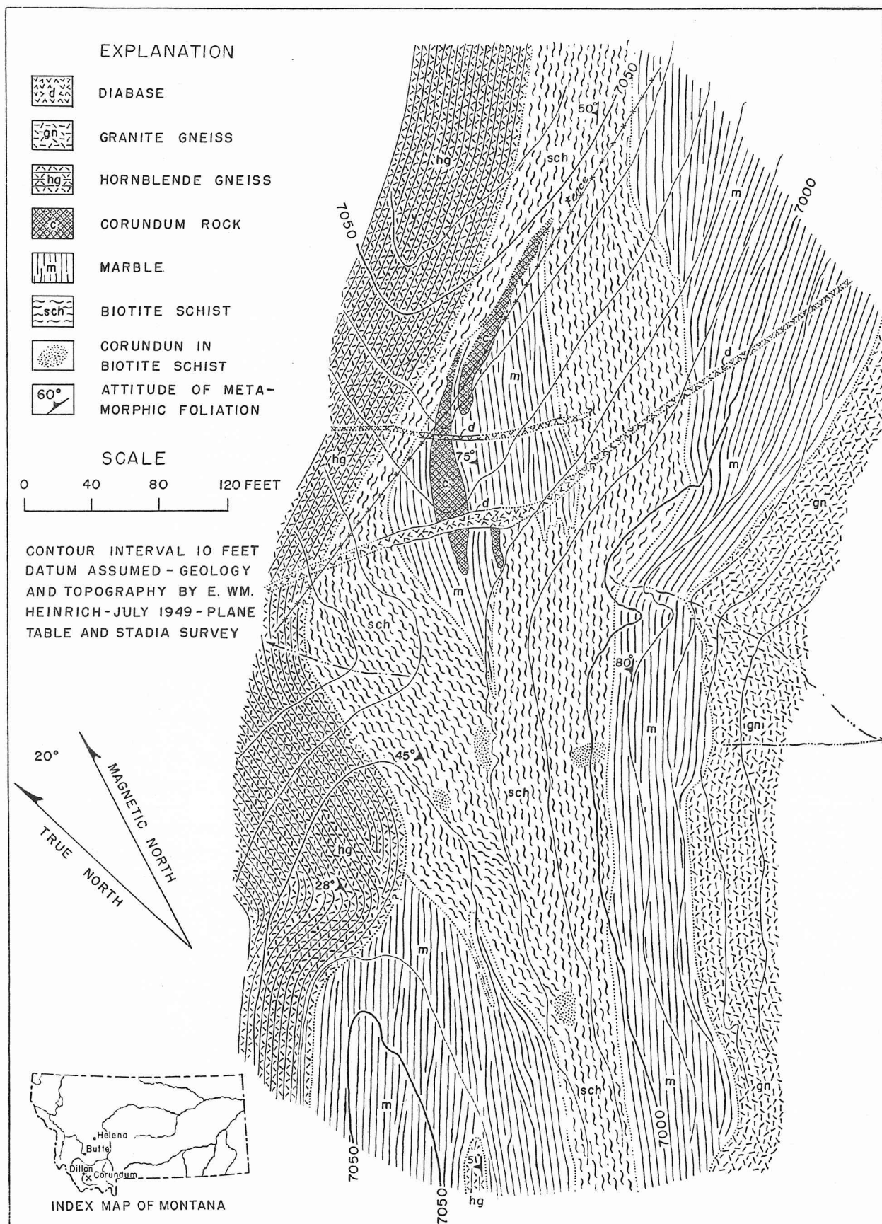
GEOLOGIC MAP OF THE CAMP CREEK CORUNDUM DEPOSIT, NE. 1/4 SEC. 36, T. 8 S., R. 8 W., BEAVERHEAD COUNTY, MONTANA.
