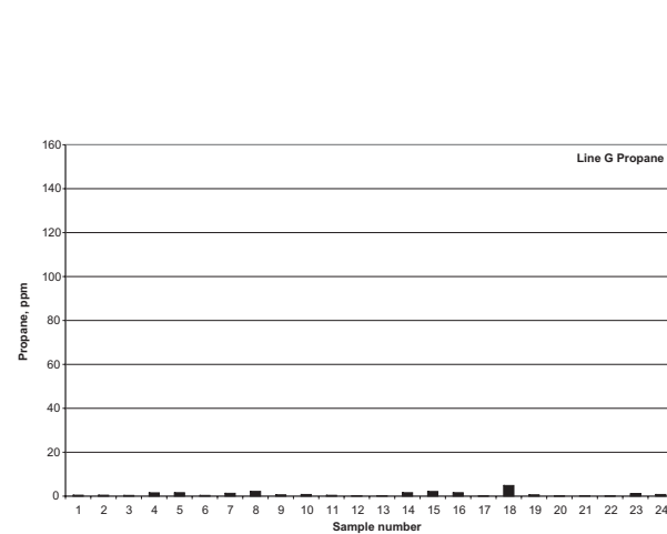
Plate 5. Butane + pentane and propane values for all sample lines.
