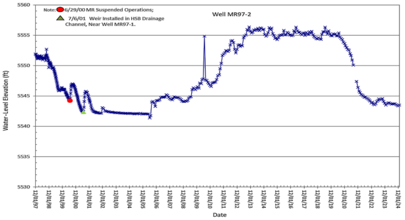
Figure 2-18. Water-level hydrograph for wells MR97-1 (top) and MR97-2 (bottom).
