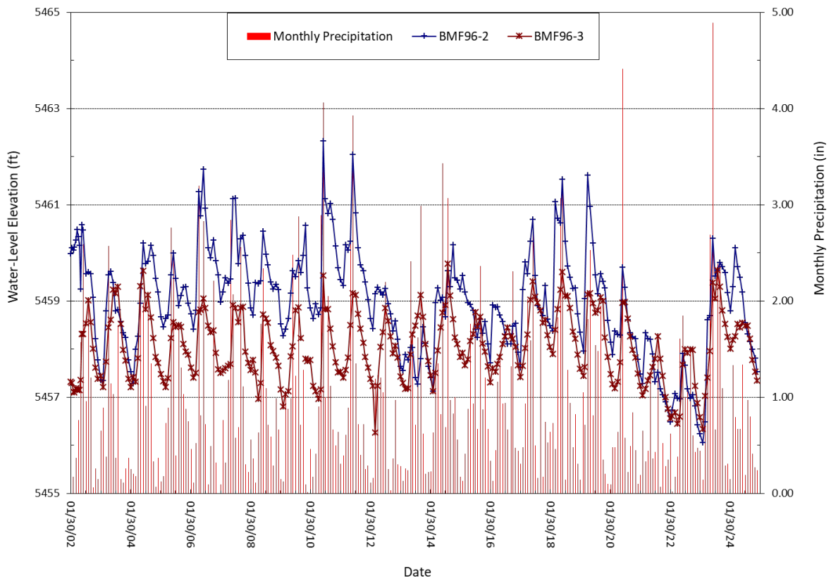
Figure 4-12. Water-level hydrographs for wells BMF96-2 and BMF96-3, 2002–2024.
