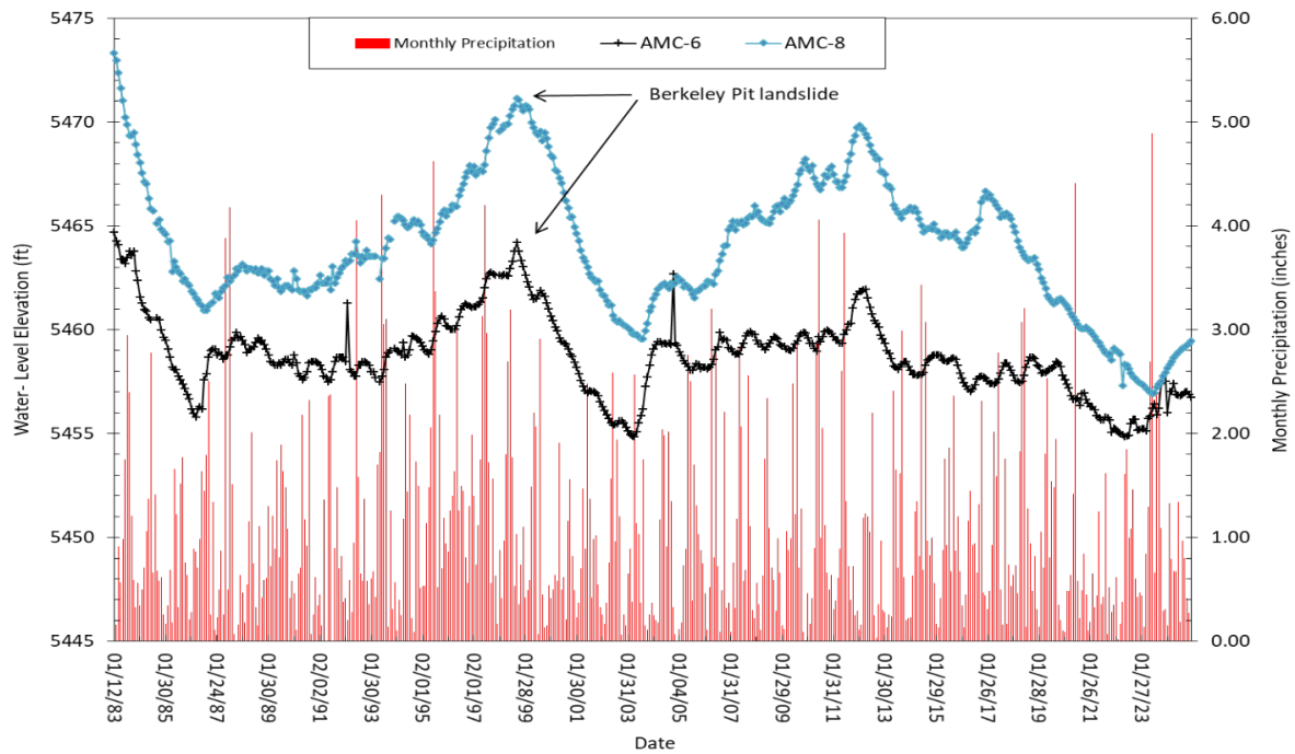
Figure 2-4. Water-level hydrographs for wells AMC-6 and AMC-8.
