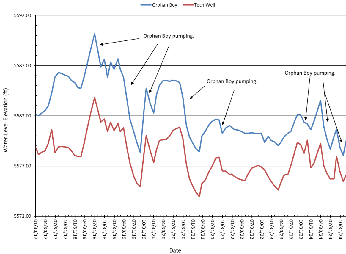
Figure 5-3. Hydrographs from the Orphan Boy and Montana Tech wells show the influence of 2018–2024 Orphan Boy pumping events and monthly water-level readings, 2017–2024.
