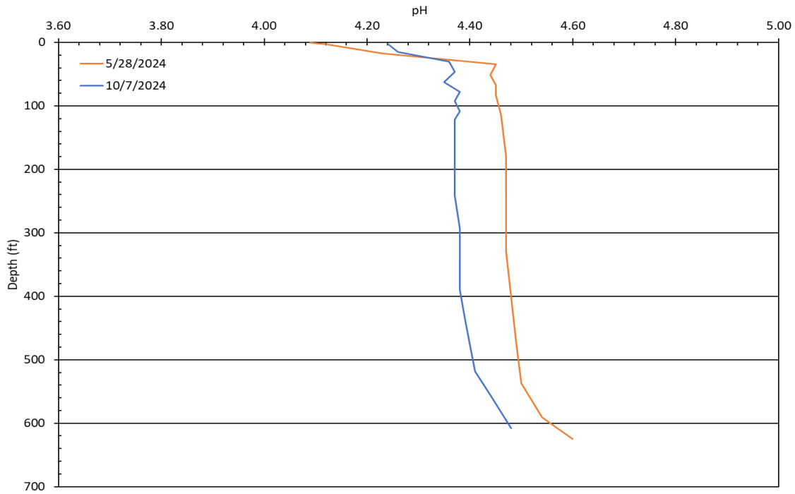
Figure 3-31. Berkeley Pit 2024 pH profiles.
