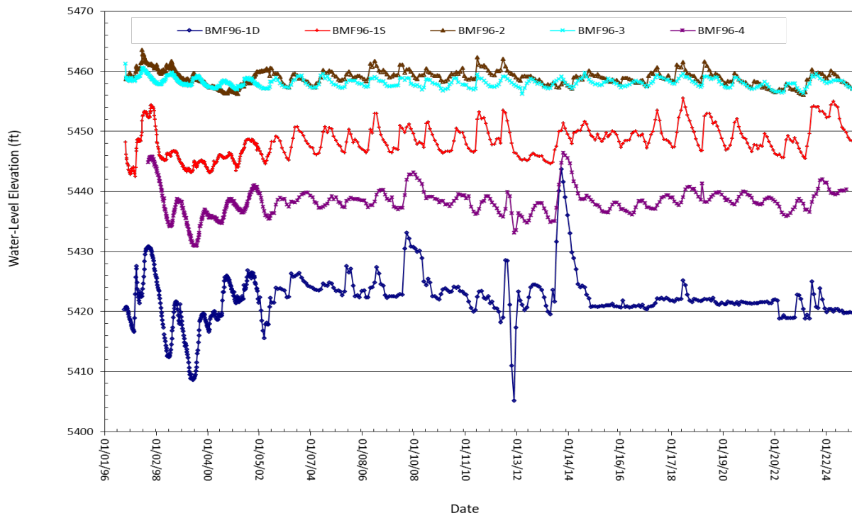
Figure 4-11. Water-level hydrographs for BMF96-series wells, 1996–2024.
