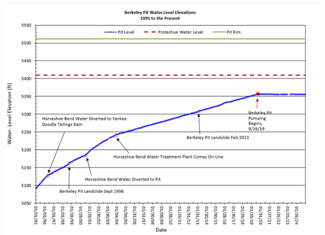
Figure 3-4. Berkeley Pit water-level hydrograph from 1995 to 2024.
