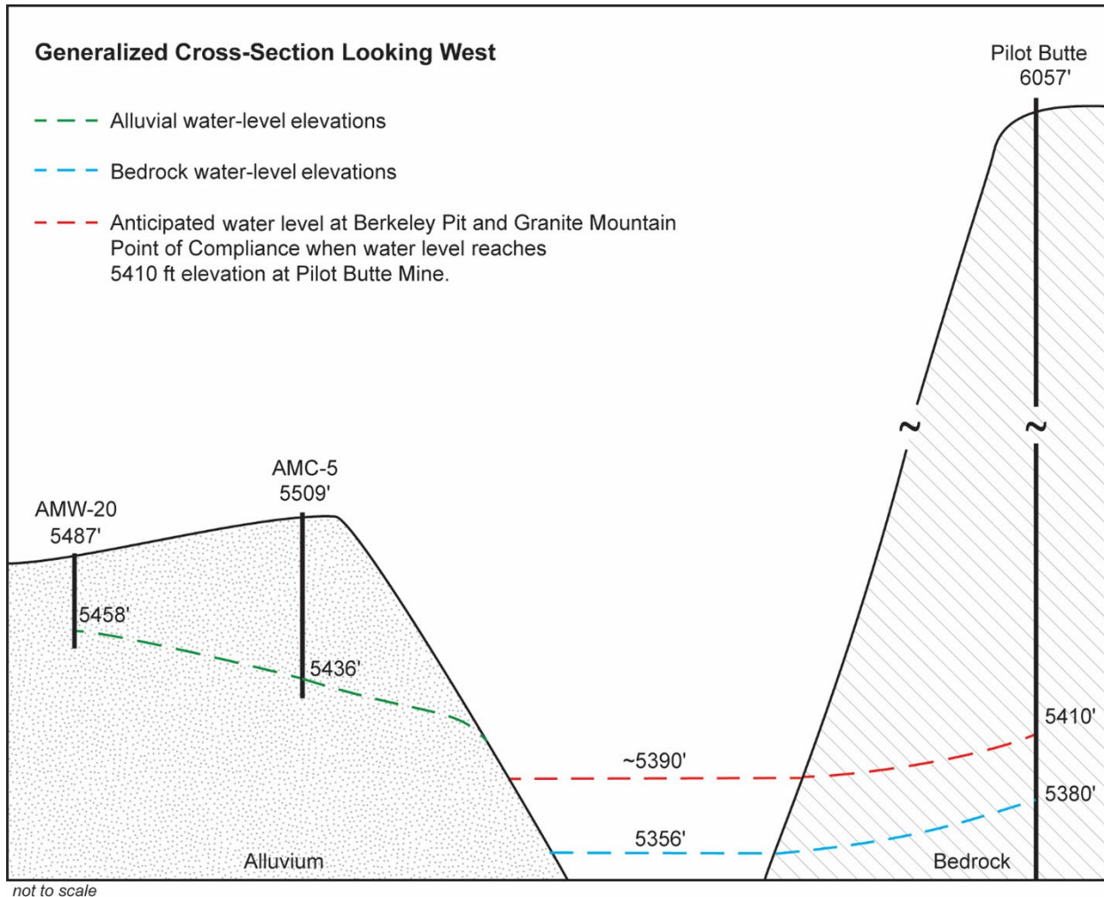
Figure 1-11. Generalized cross-section looking west through the Berkeley Pit depicting water-level elevations in bedrock and alluvial systems in December 2024 and projected elevations when the 5,410 Protective Water Elevation is reached at the Pilot Butte Mine (location shown in figure 1-10).
