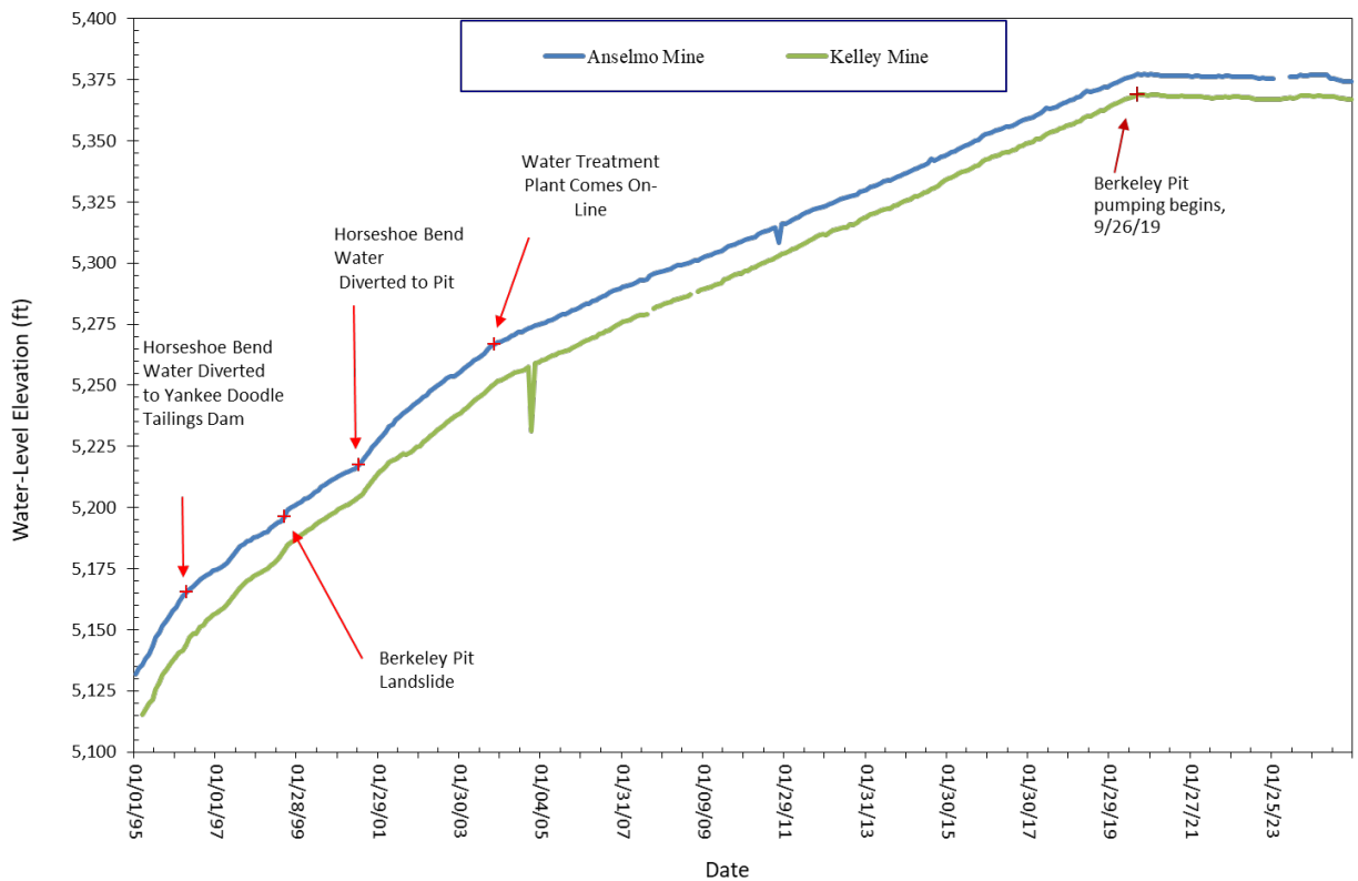
Figure 3-3. Water-level hydrograph for the Anselmo and Kelley mines from 1995 to 2024, and significant events that affected the rate of water-level rise.
