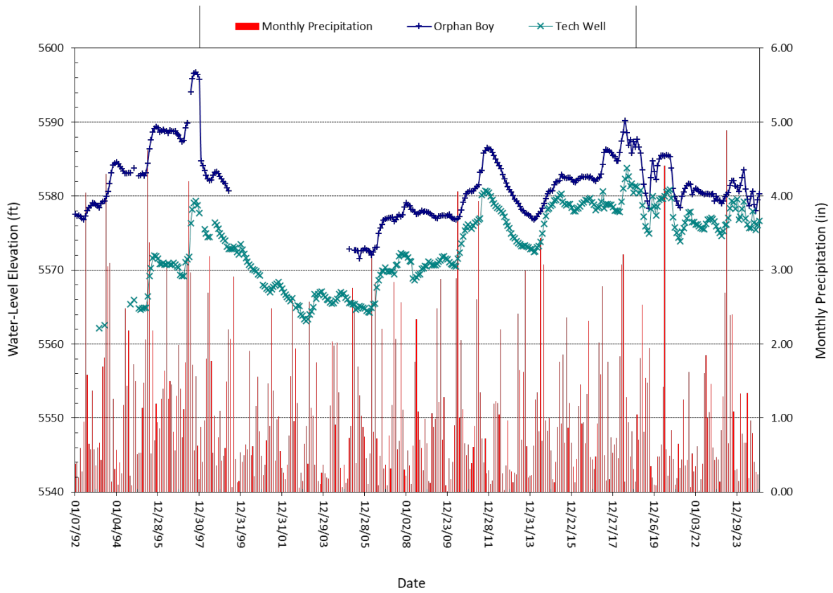
Figure 5-4. Water-level hydrograph for the Orphan Boy Mine and Montana Tech wells.
