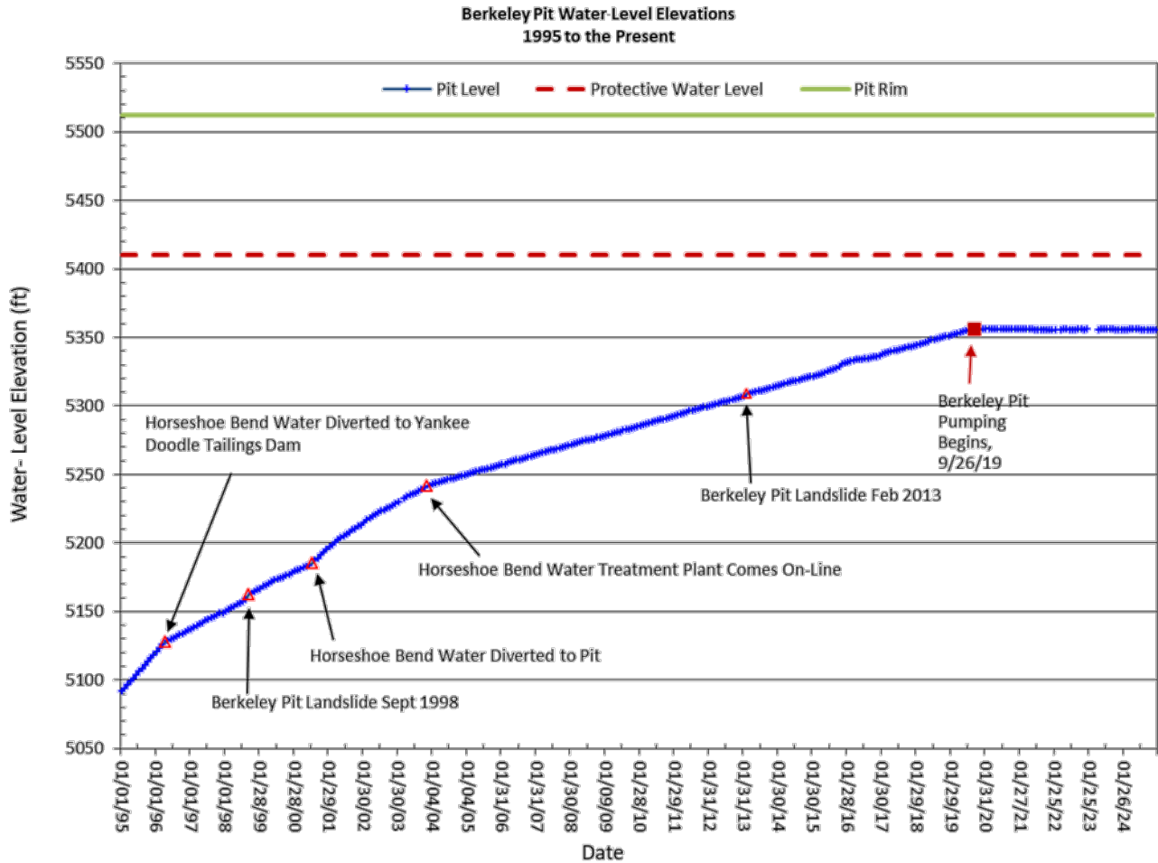
Figure 3-24. Water-level hydrograph of the Berkeley Pit, 1995–2024.
