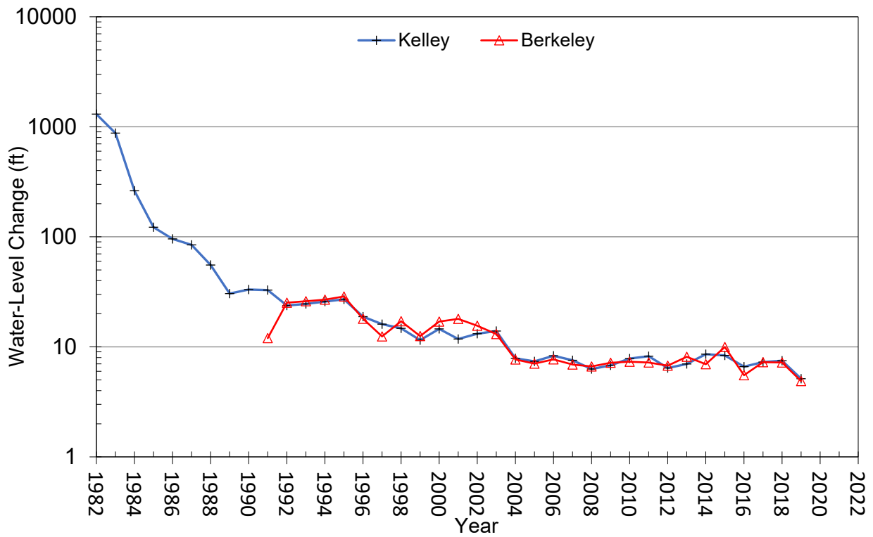
Figure 3-2A. Kelley Mine and Berkeley Pit annual water-level changes, 1982–2020.
