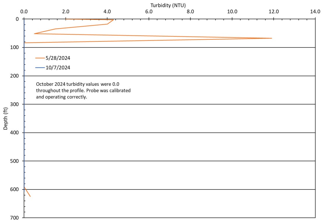
Figure 3-36. Berkeley Pit 2024 turbidity profiles.
