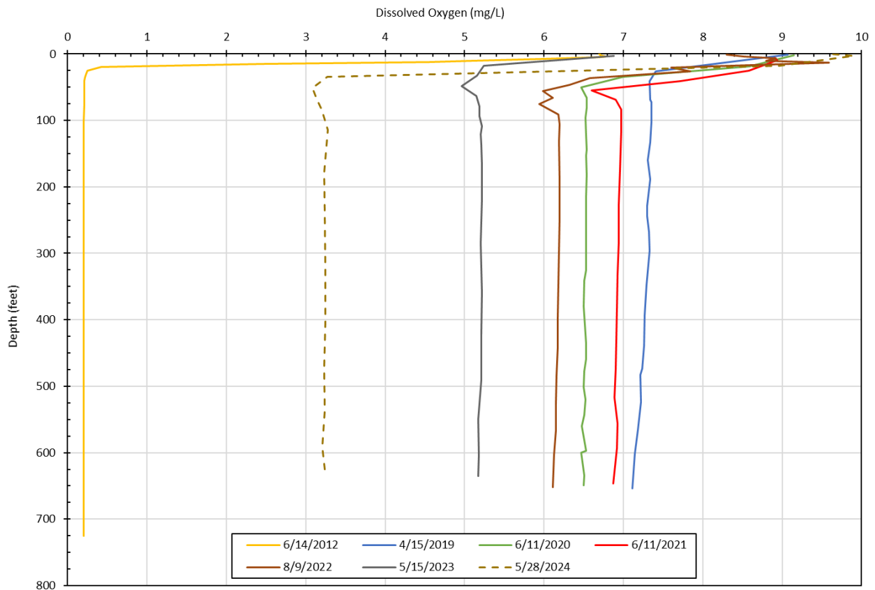
Figure 3-37. Comparison of dissolved oxygen profiles in the pit during spring 2012 and spring 2019–2024.
