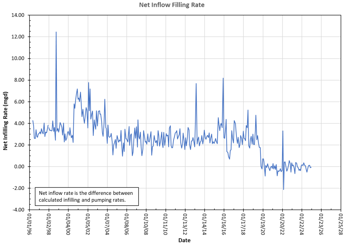
Figure 6-2. Berkeley Pit net filling rate, 1996–2024.
