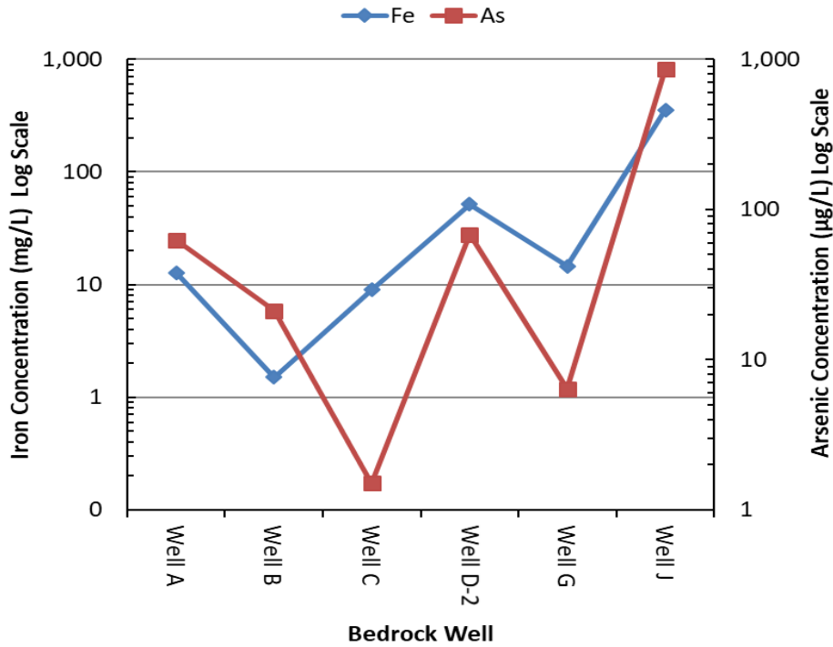
Figure 3-16. Bedrock well iron and arsenic concentration comparisons, spring 2024.
