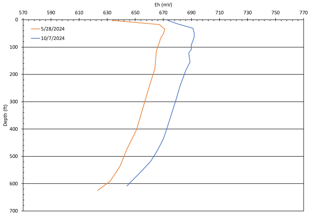
Figure 3-35. Berkeley Pit 2024 oxidation reduction profiles (Eh).
