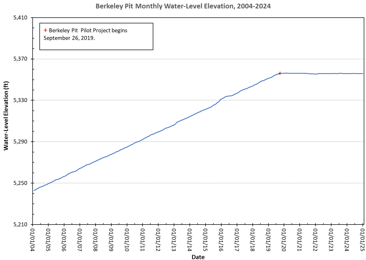
Figure 6-1. Berkeley Pit water-level elevation from 2004 through 2024. The Horseshoe Bend water-treatment plant came online in late 2003 and Horseshoe Bend water was no longer allowed to flow into the Berkeley Pit. The beginning of the Berkeley Pit Pilot Project is also shown.
