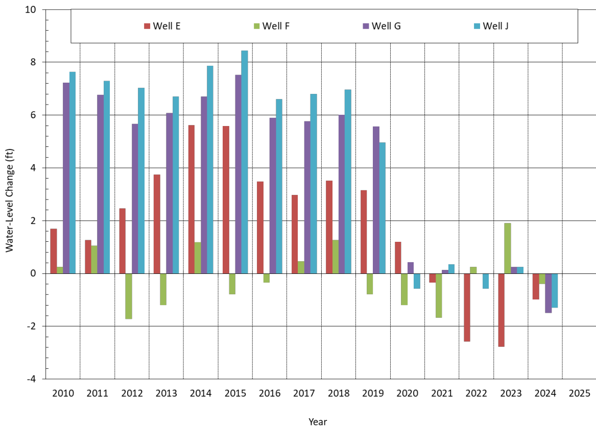
Figure 3-9. Annual water-level change in bedrock wells from 2010 to 2024.
