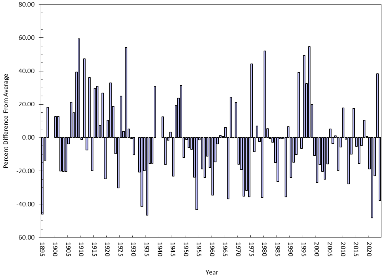
Figure 1-14. Percentage precipitation variation from normal, 1895–2024.
