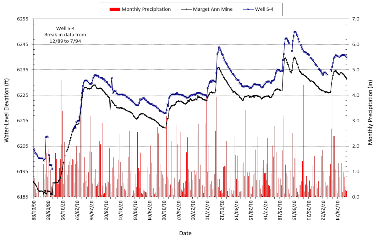
Figure 5-5. Water-level hydrograph for the Marget Ann Mine and well S-4.
