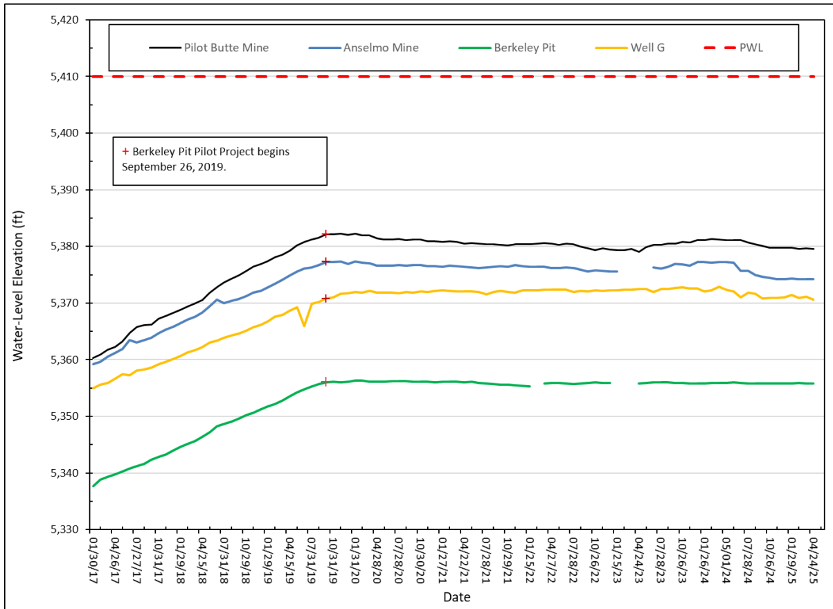
Figure 3-5. Water-level hydrograph for the Berkeley Pit and other selected bedrock monitoring sites, 2017–2024.
