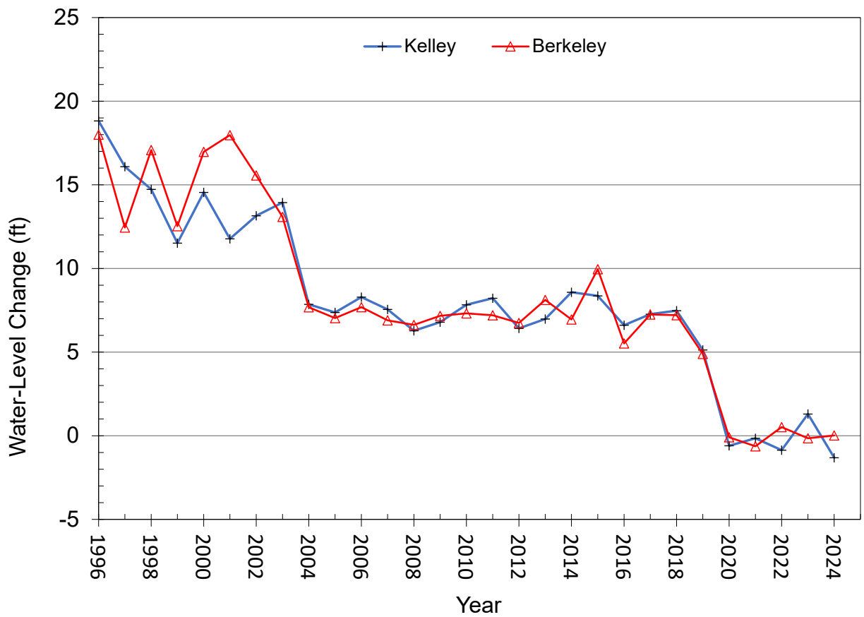
Figure 3-2B. Kelley Mine and Berkeley Pit annual water-level changes, 1996–2024.
