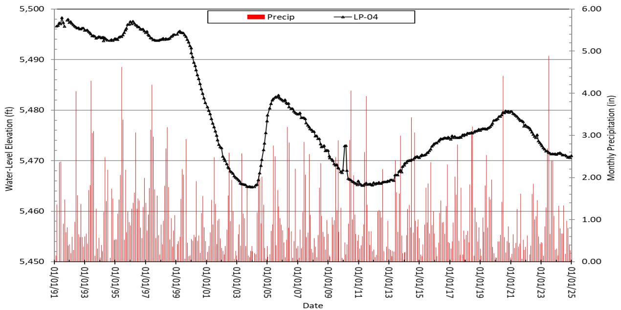
Figure 2-11. Hydrograph for well LP-04 located north of the Pittsmont Waste Dump and south of the leach pads.
