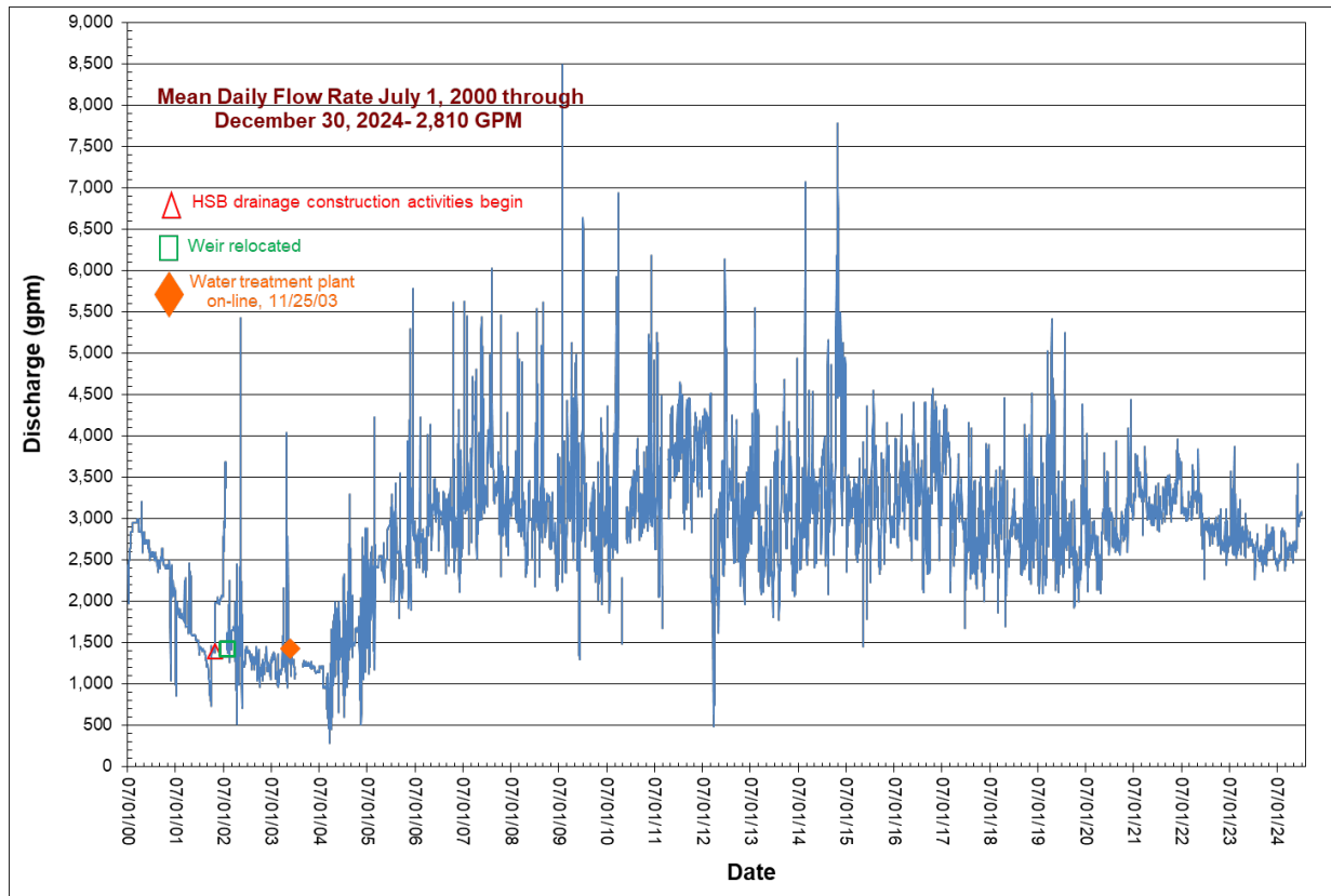
Figure 3-26. Horseshoe Bend Drainage flow rate, July 2000 through December 2024.
