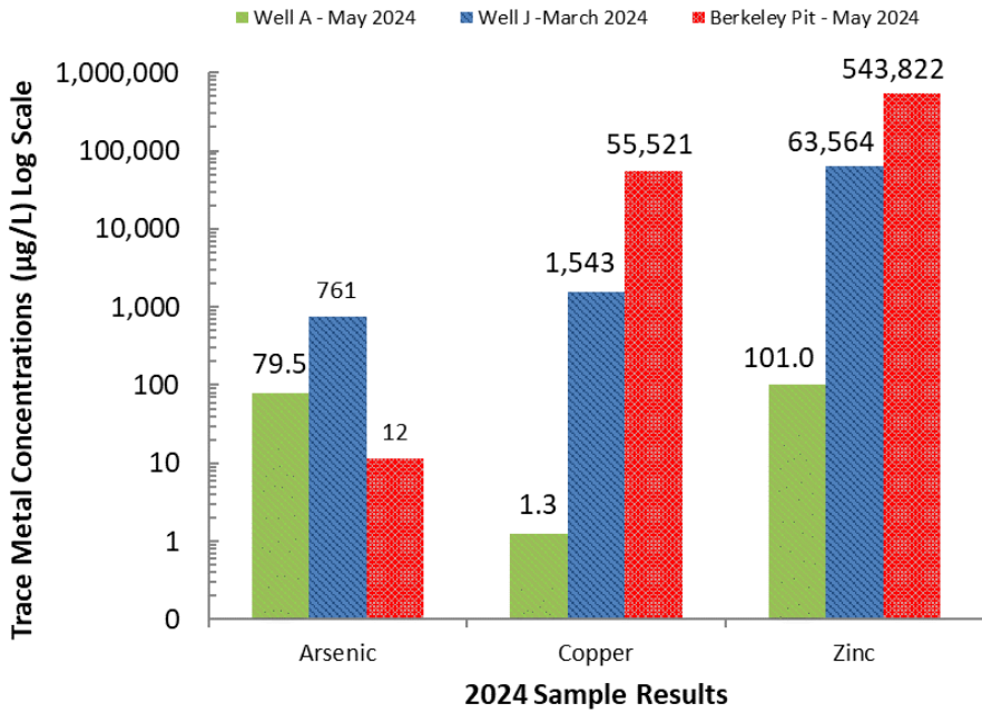
Figure 3-17. Selected trace metal comparisons among bedrock wells A, J, and the Berkeley Pit 4-ft depth sample.
