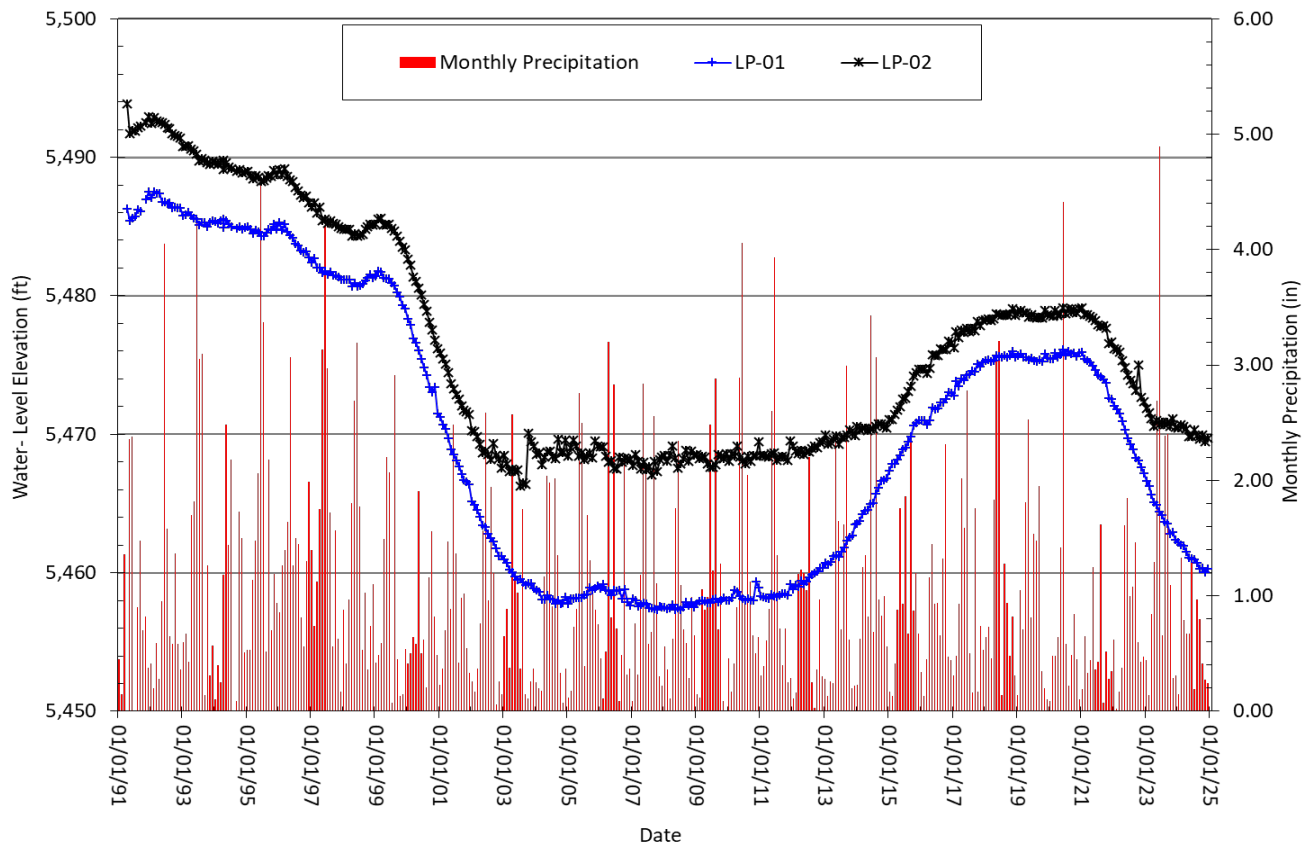
Figure 2-10. Hydrographs for wells LP-01 and LP-02 located north of the Pittsmont Waste Dump and south of the leach pads.
