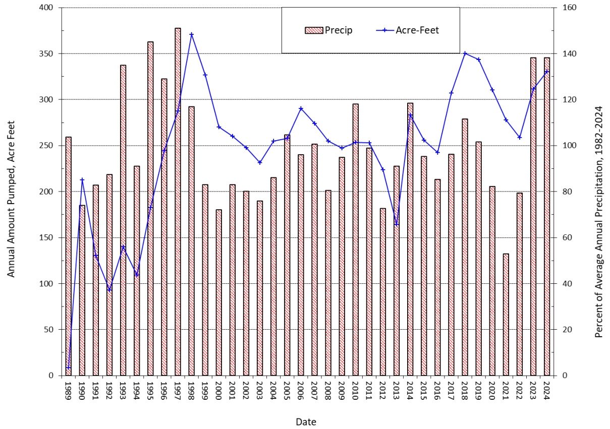
Figure 4-6. Annual amount of water pumped from the West Camp System compared to the average annual precipitation during the period 1982–2024.
