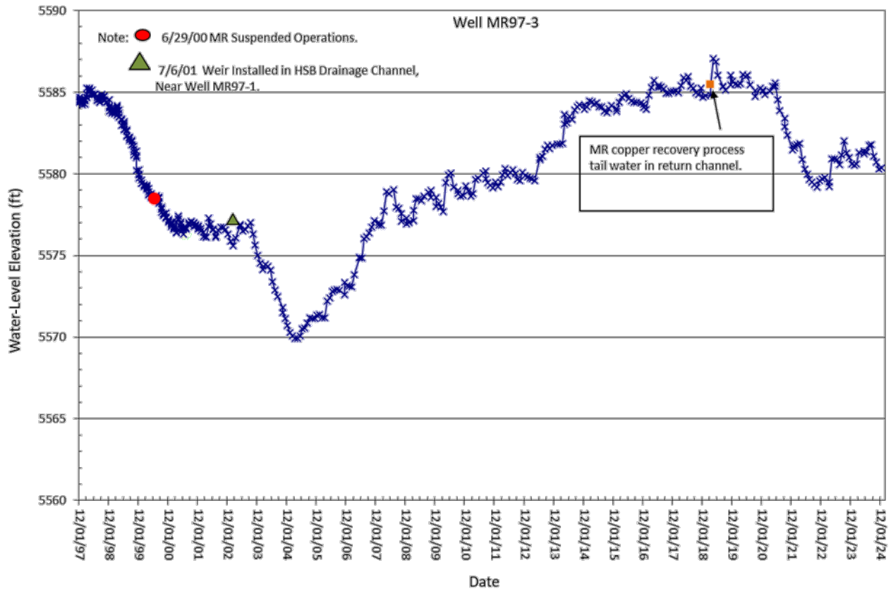
Figure 2-19. Water-level hydrograph for well MR97-3.
