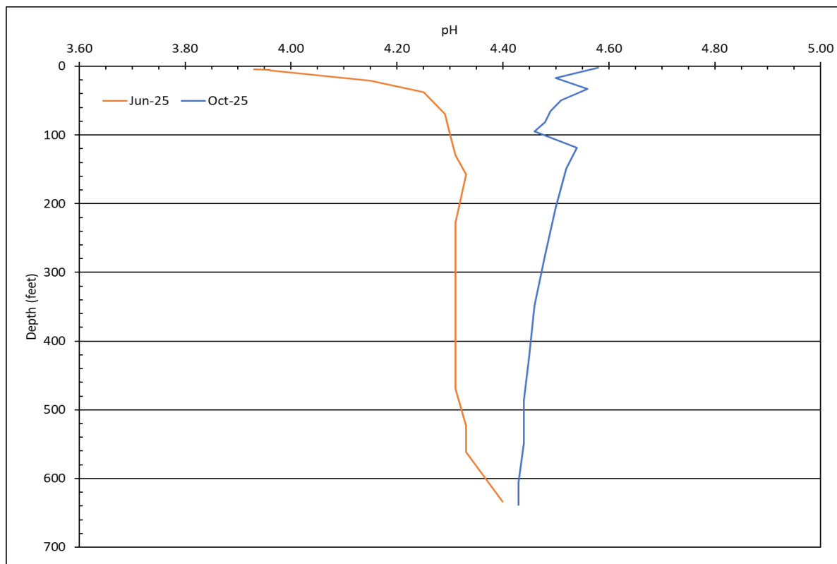
Figure 3-31. Berkeley Pit 2025 pH profiles.
