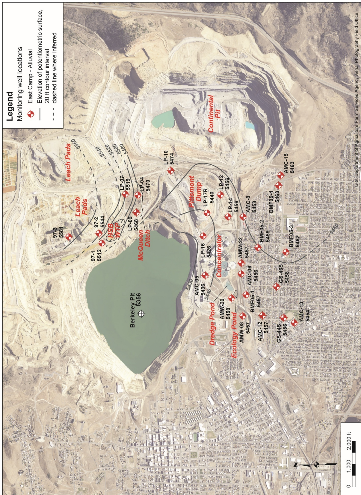
Figure 2-14. Alluvial aquifer potentiometric map for December 2025 (contour interval is 20 ft).
