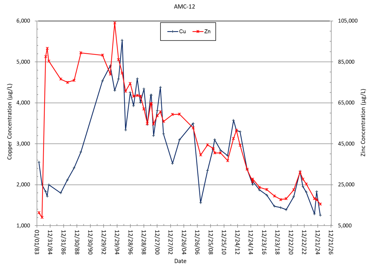
Figure 2-8. Copper and zinc concentration changes over time for well AMC-12.
