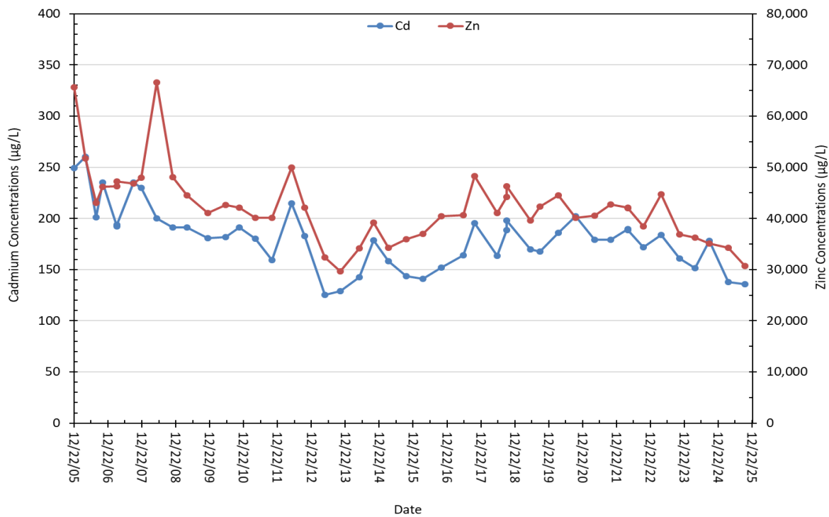
Figure 2-27. Cadmium and zinc concentration trends in well BMF05-1.
