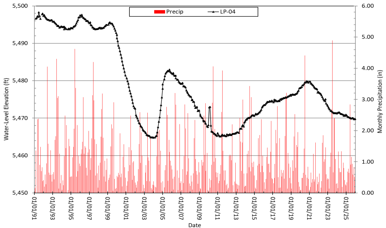
Figure 2-11. Hydrograph for well LP-04 located north of the Pittsmont Waste Dump and south of the leach pads.
