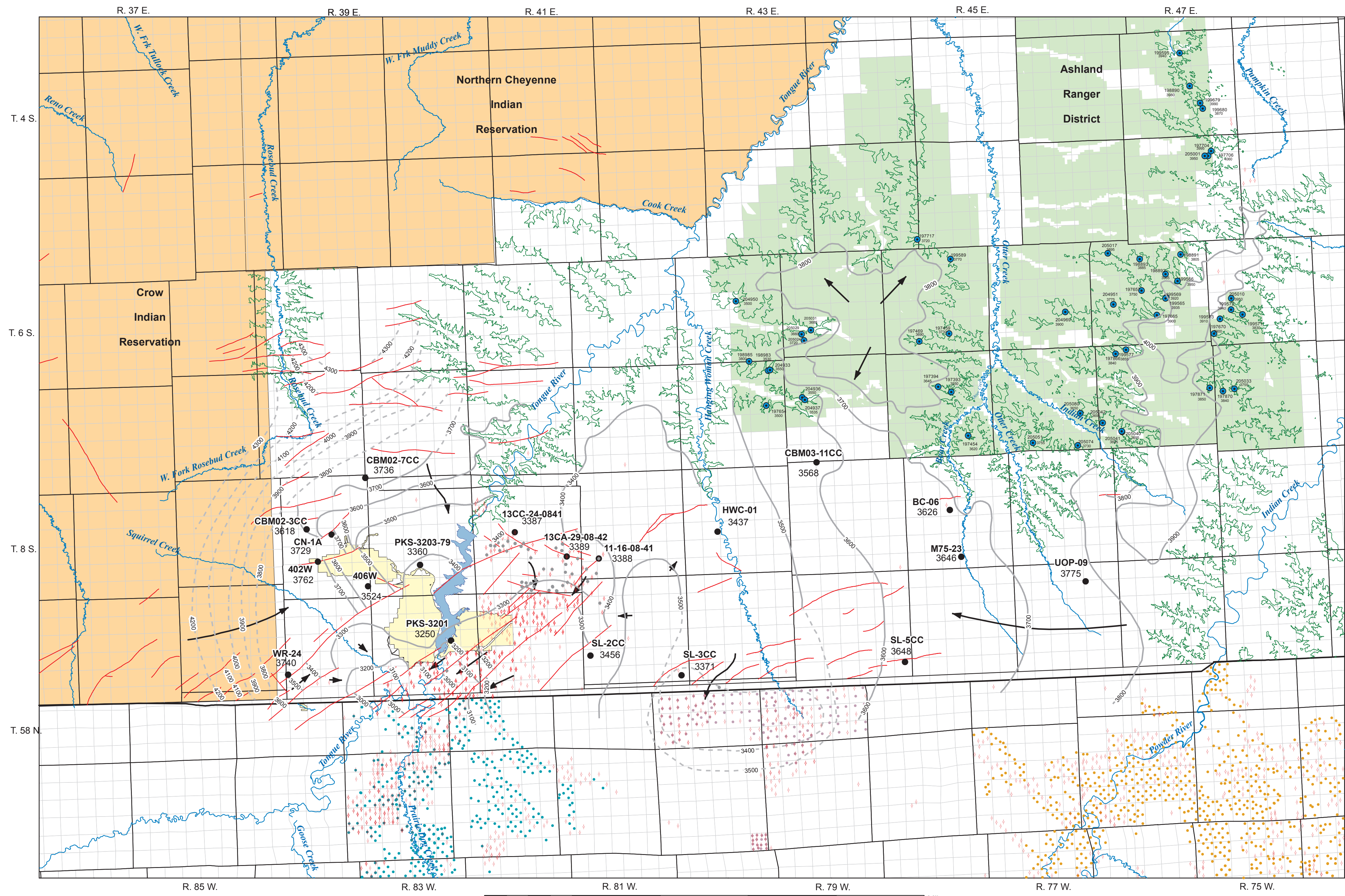
Plate 3. Potentiometric surface of the Canyon coal in the southern portion of the Powder River Basin, Montana, 2013.
