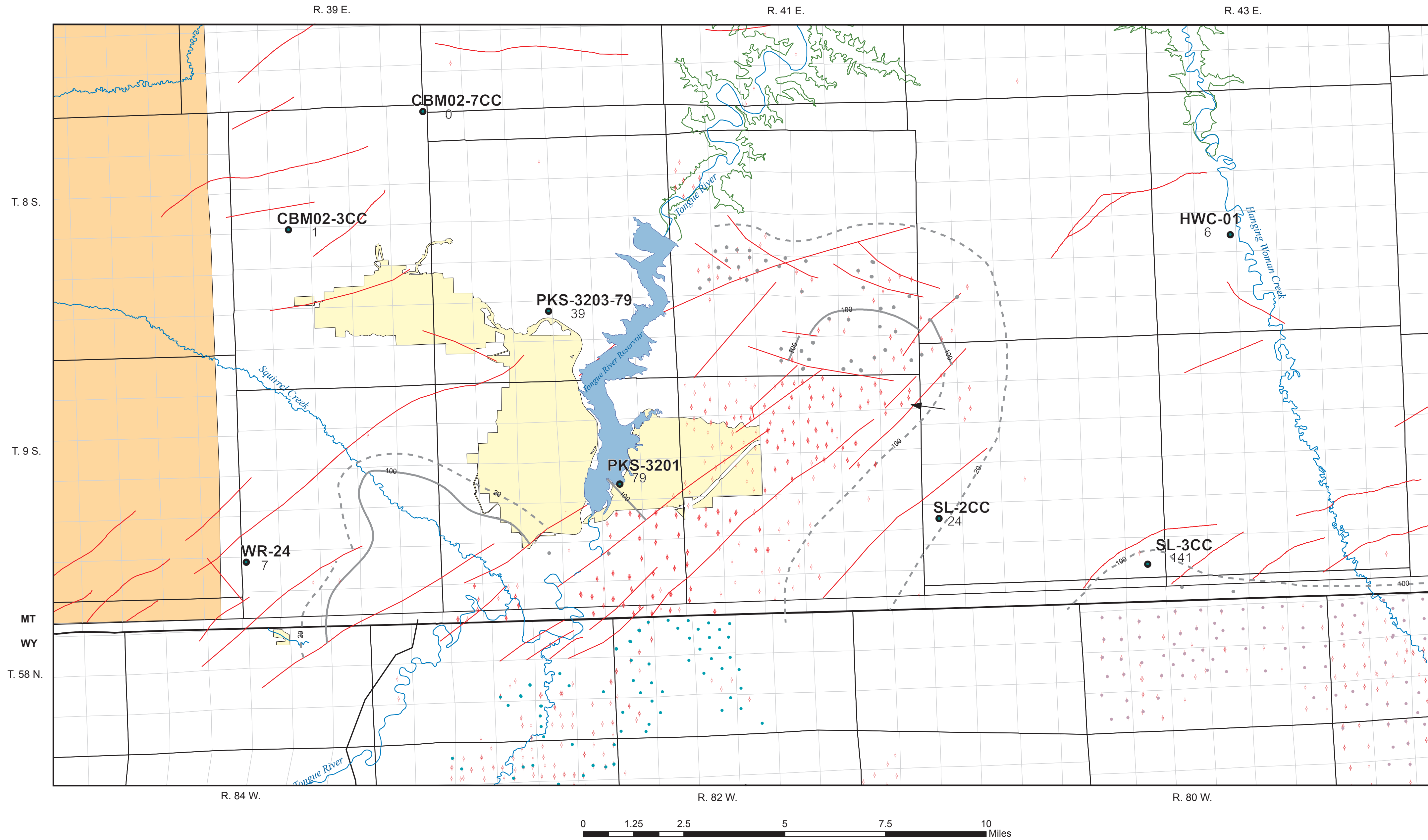
Plate 5. Area of CBM-related potentiometric decline for the Canyon coal in the southern portion of the Powder River Basin, Montana, 2014
