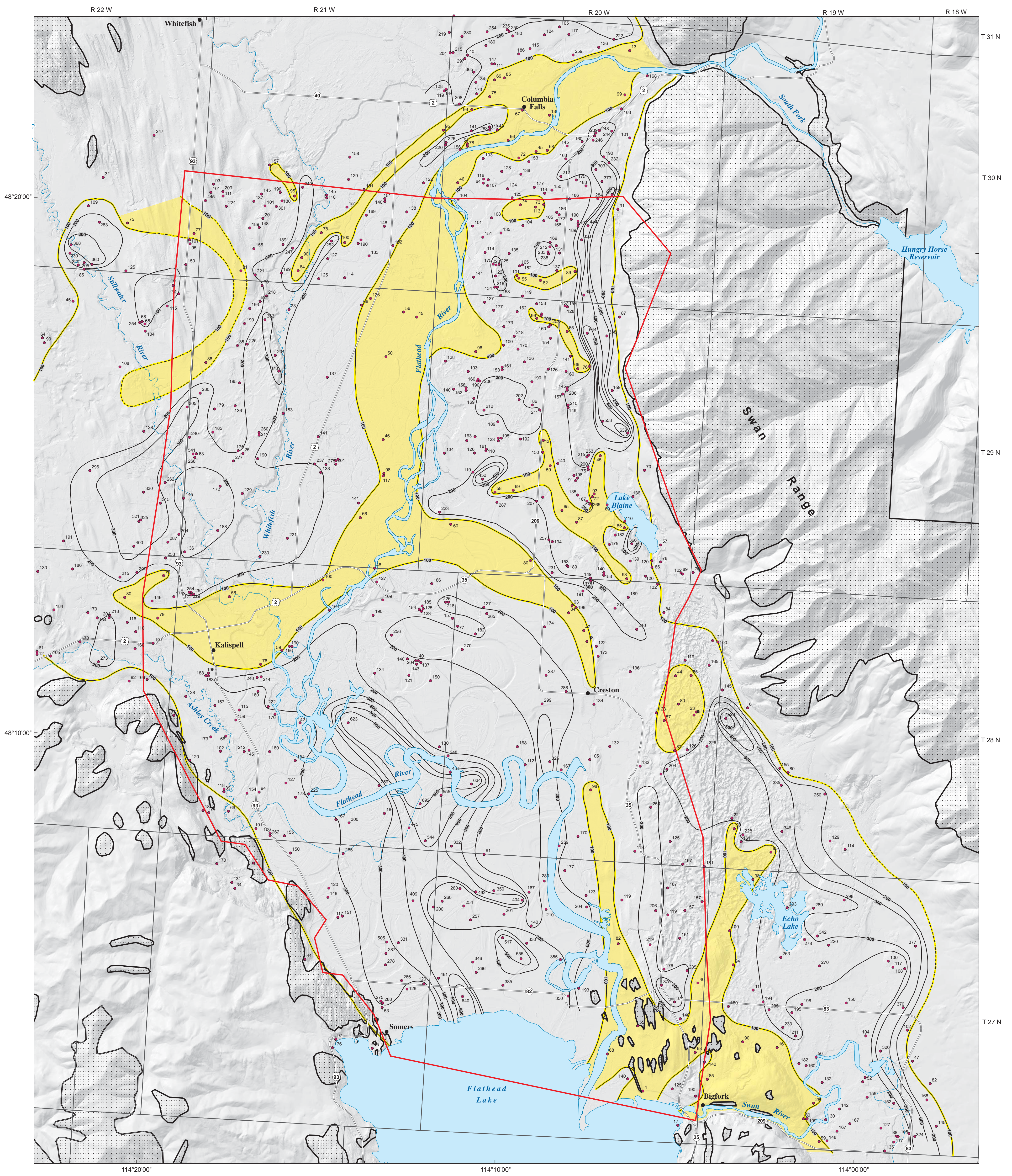
Plate 1. Lacustrine-till Aquitard Thickness Map
