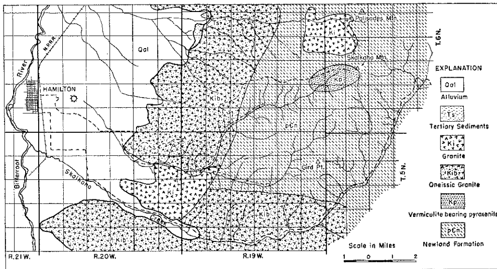
Figure 10.—Map showing location of Vermiculite deposits near Hamilton, Montana.
