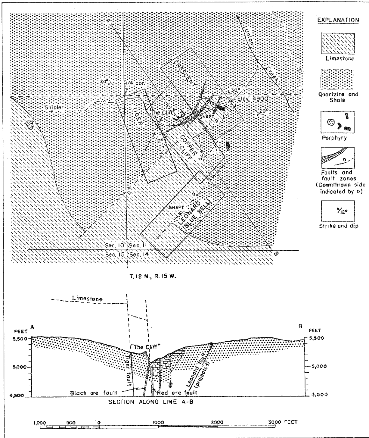
Figure 5.—Geologic map and section of the vicinity of Copper Cliff, Garnet Range, Mont. (From U.S.G.S. Bulletin 660, p. 216.)
