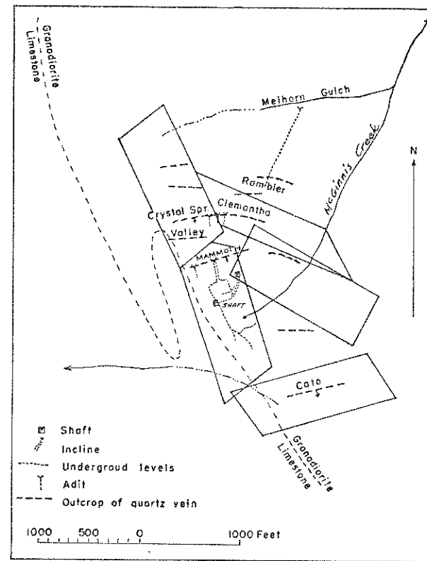
Figure 4.—Veins at Coloma, Garnet Range, Montana. (From U.S.G.S. Bulletin 660, p. 196.)
