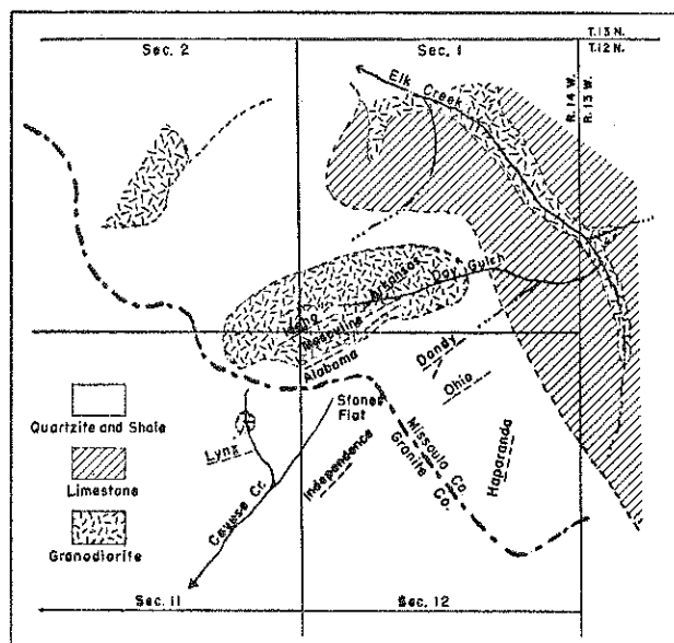
Figure 2.—Veins at the Head of Elk Creek, Garnet Range, Montana.
