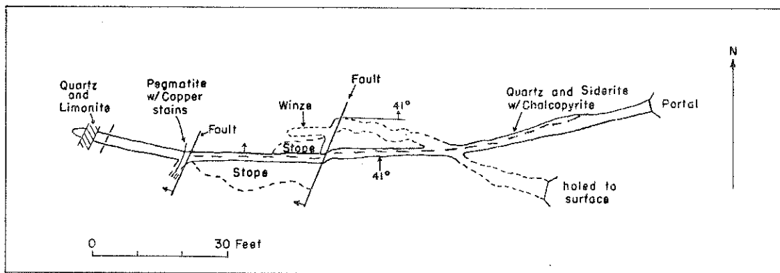
Figure 8-Sketch map of middle adit, Lawyers Combination Mine, Lolo Creek District.
