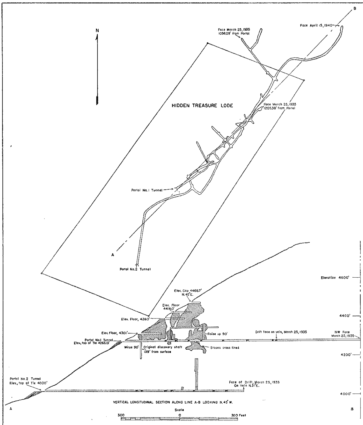
Figure 6.—Plan and Section, Underground Workings, Hidden Treasure Mine. (After Piquette, 1940.)
