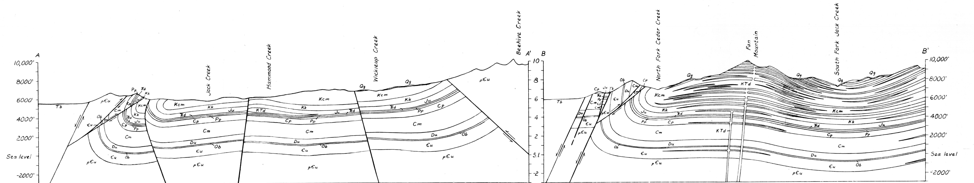
SECTION ALONG LINE B-B'
