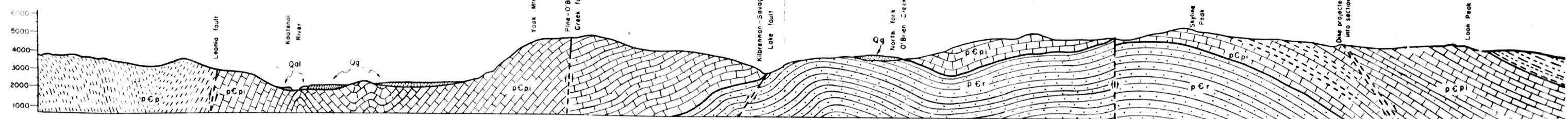
SECTION A-A' (W. 1/2) GEOLOGIC MAP SOUTH HALF YAAK RIVER QUADRANGLE LINCOLN COUNTY, MONTANA
