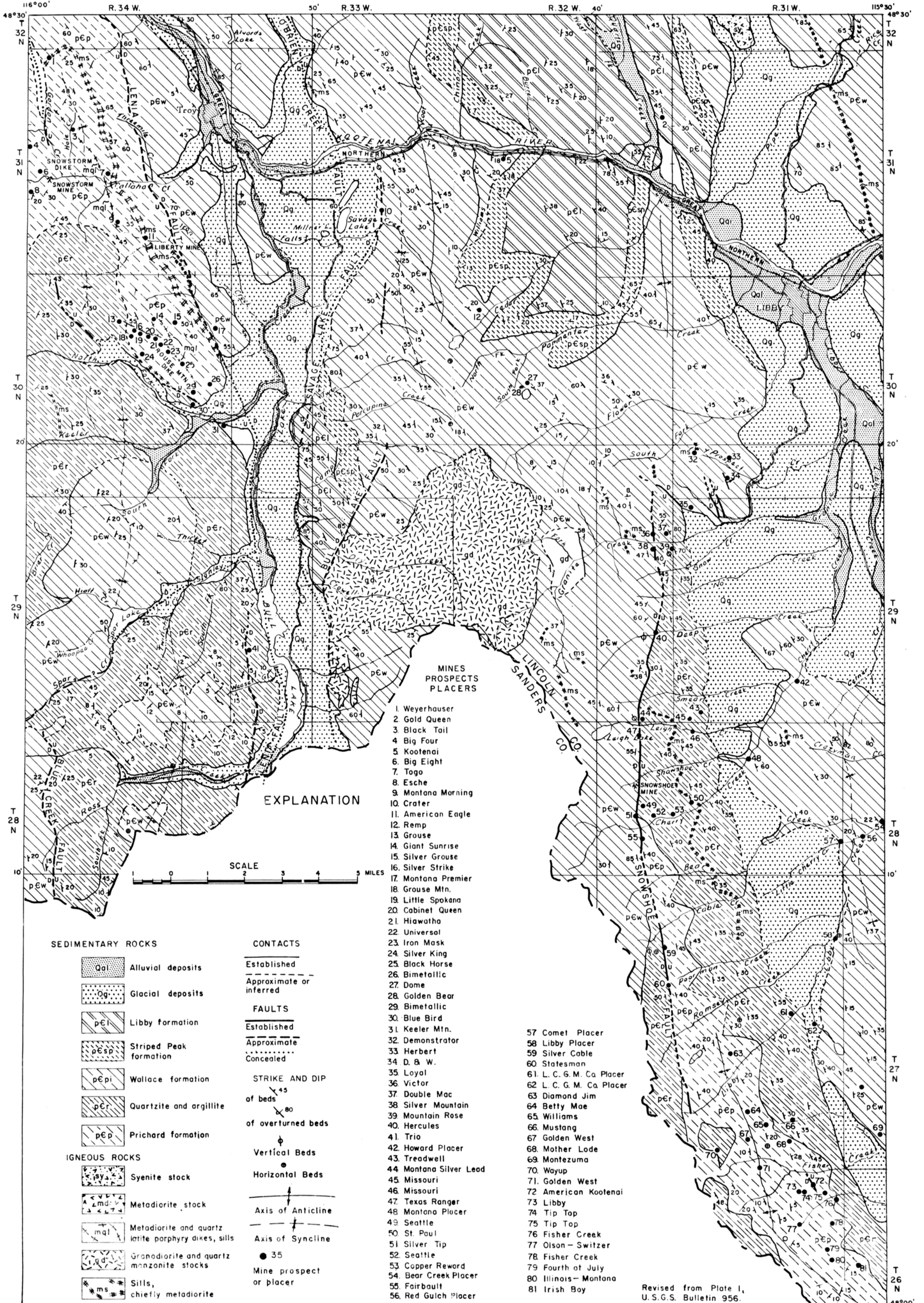
GEOLOGIC MAP OF SOUTHWEST PART OF LINCOLN COUNTY, MONTANA
