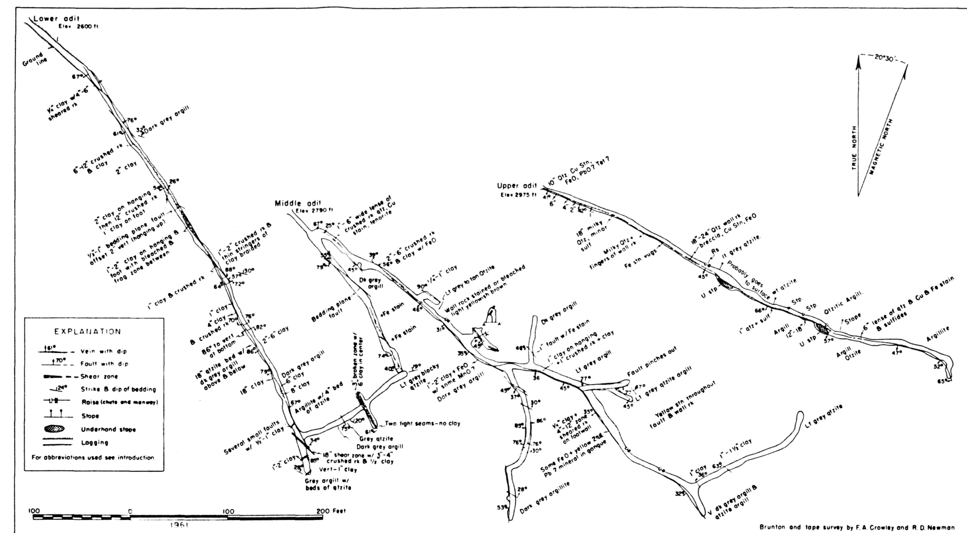
D—Geologic map of workings of Silver King mine, Thompson River mining district.
