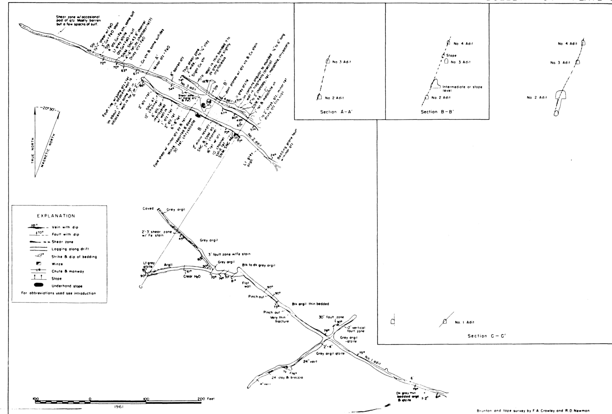
C—Geologic map with sections of workings of the Raven mine, Thompson River mining district.
