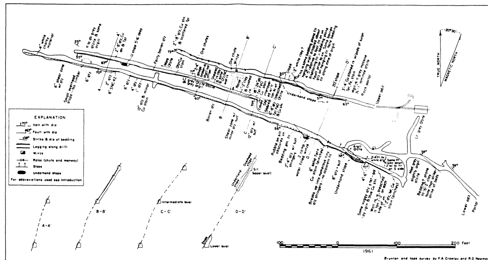
B—Geologic map with sections of workings of Copper King mine, Thompson River mining district.
