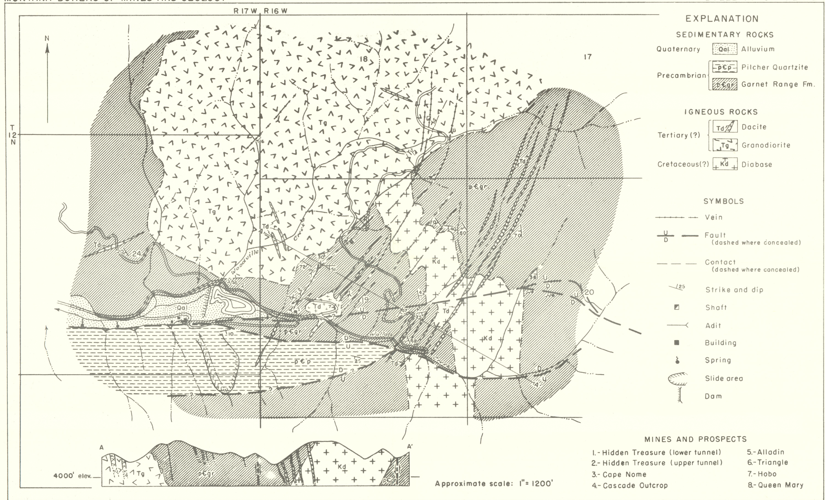
GEOLOGIC MAP OF THE CLINTON MINING DISTRICT MISSOULA COUNTY, MONTANA
