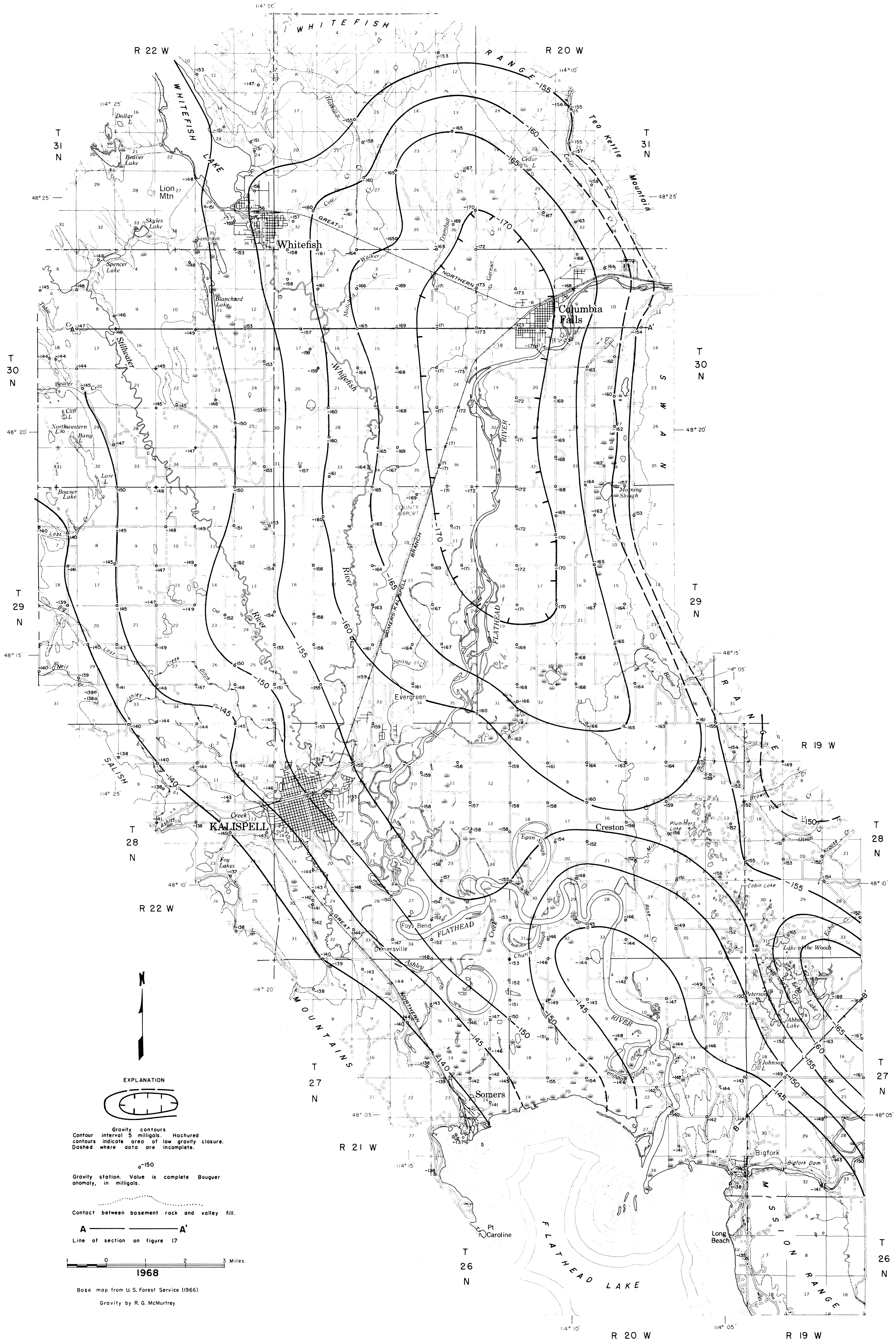
BOUGUER GRAVITY MAP OF THE KALISPELL VALLEY AND ADJACENT HIGHLANDS
