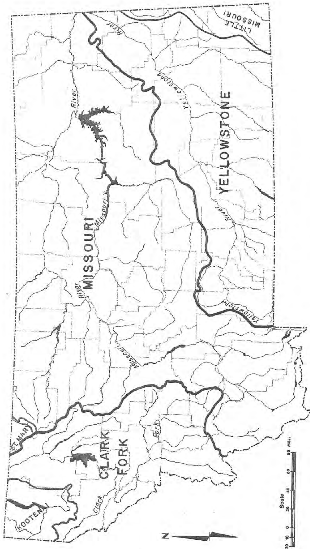
MAJOR DRAINAGE BASINS
