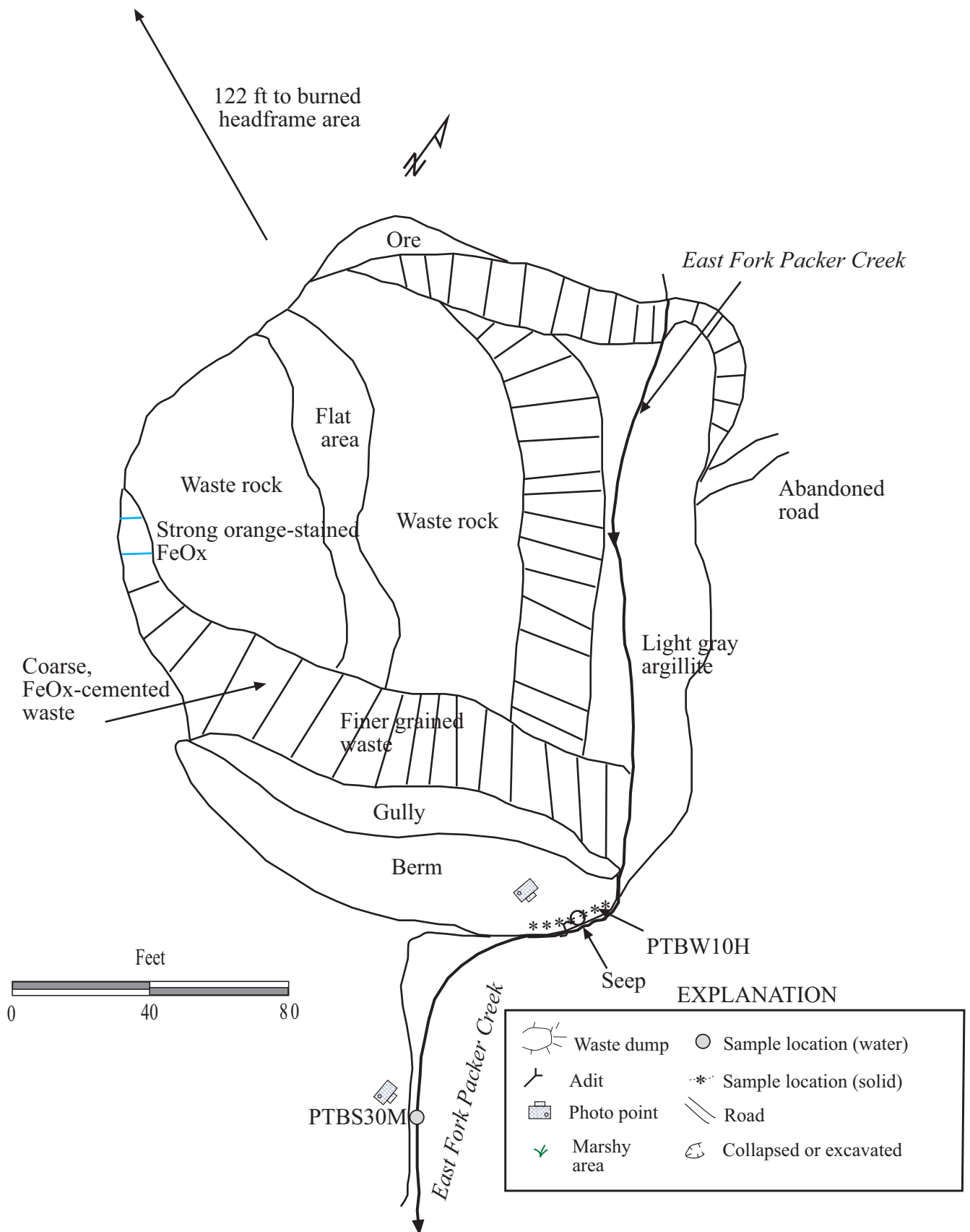
Figure 15. The Tarbox Mine waste-rock dump and ore pile were situated in the original channel of the East Fork of Packer Creek as inventoried on 08/08/01.
