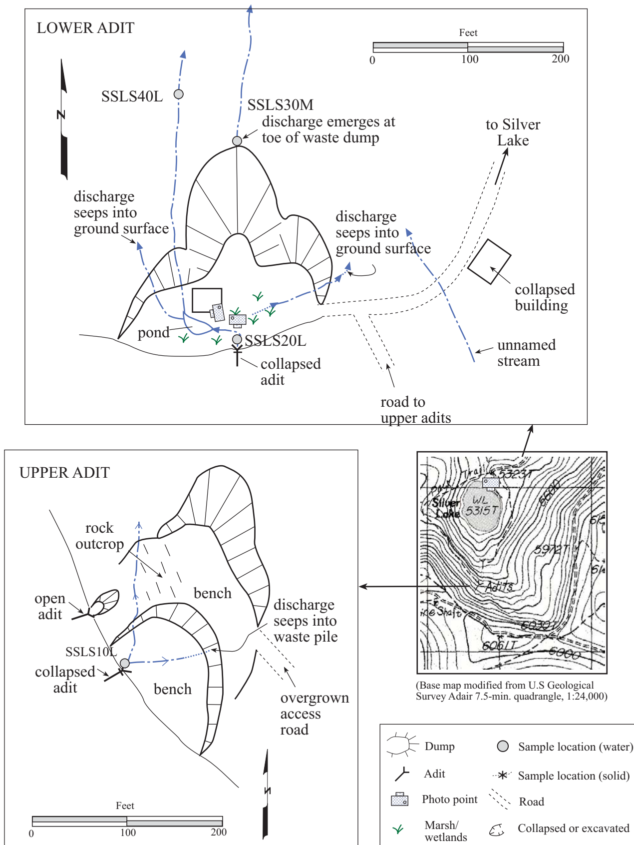
Figure 20. The St. Lawrence area had two adit discharges, a seep, and eroding waste-rock dumps, as mapped 07/12/01.
