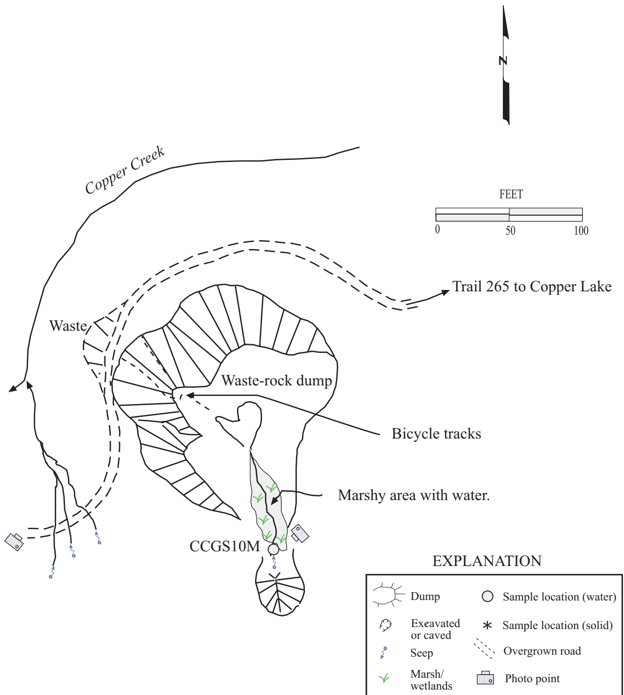
Figure 19. The mine near Copper Lake had both an adit discharge and numerous natural seeps, as mapped 07/25/01.
