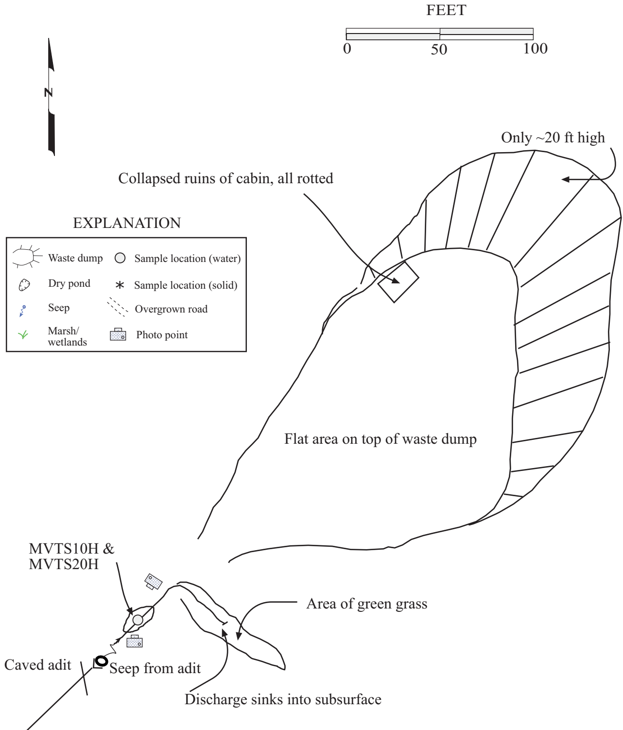
Figure 24. The small discharge at the Vulcan Tunnel at the Nancy Lee mine site soaked into the ground less than 50 ft from the adit, as mapped 07/24/01.
