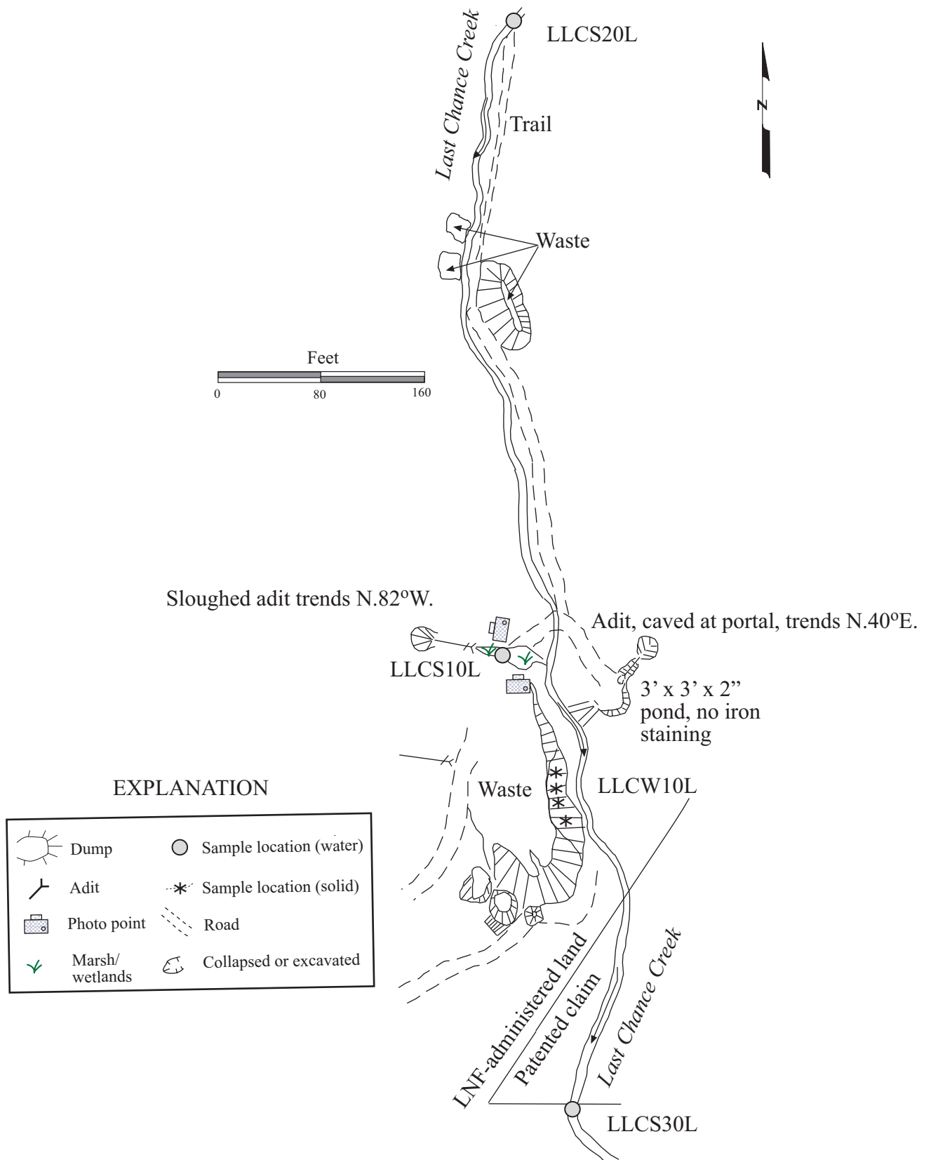
Figure 13. The adits at the Last Chance Mine leaked water and the largest discharge was sampled on 08/08/01.
