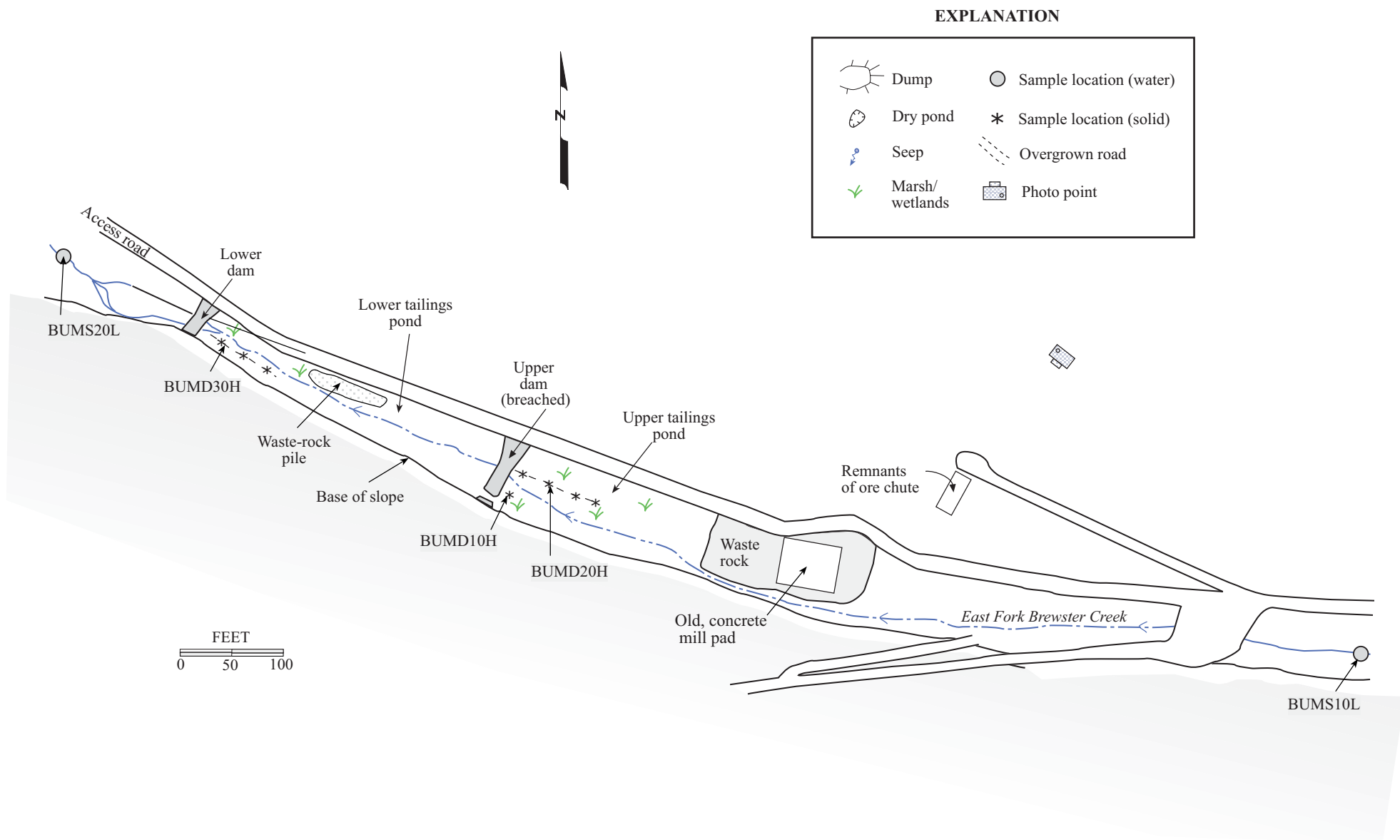
Figure 7. The mill on the East Fork of Brewster Creek had two dams that created catch ponds, which were mapped and sampled 10/20/00 and 07/23/01.
