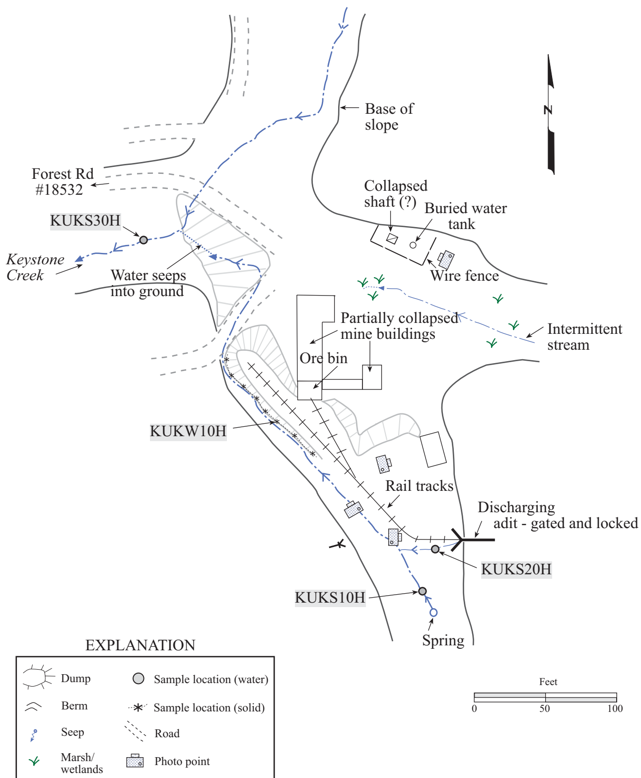
Figure 22. The Upper Keystone Mine consisted of a discharging gated adit, a streamside waste-rock dump, and potentially hazardous buildings.
