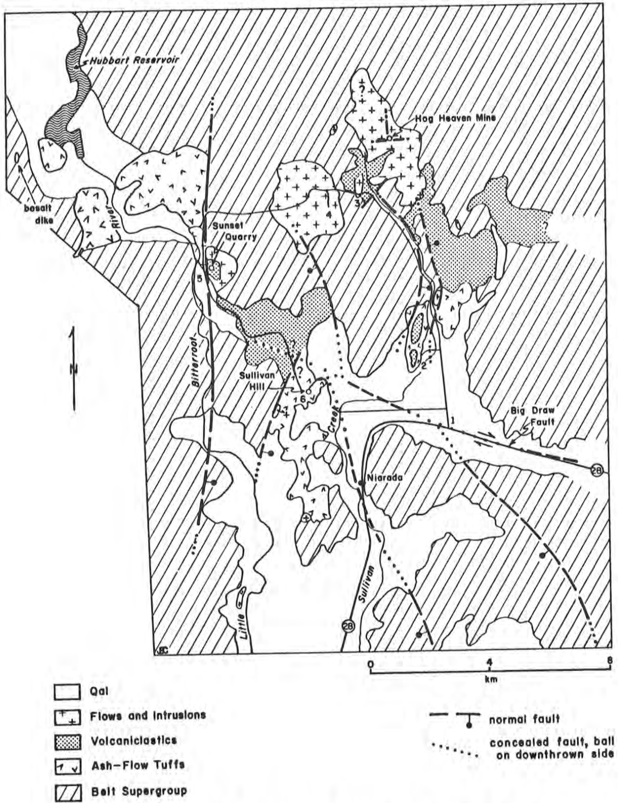
Figure 1. Geologic map of Hog Heaven volcanic field showing field trip route and stops.
