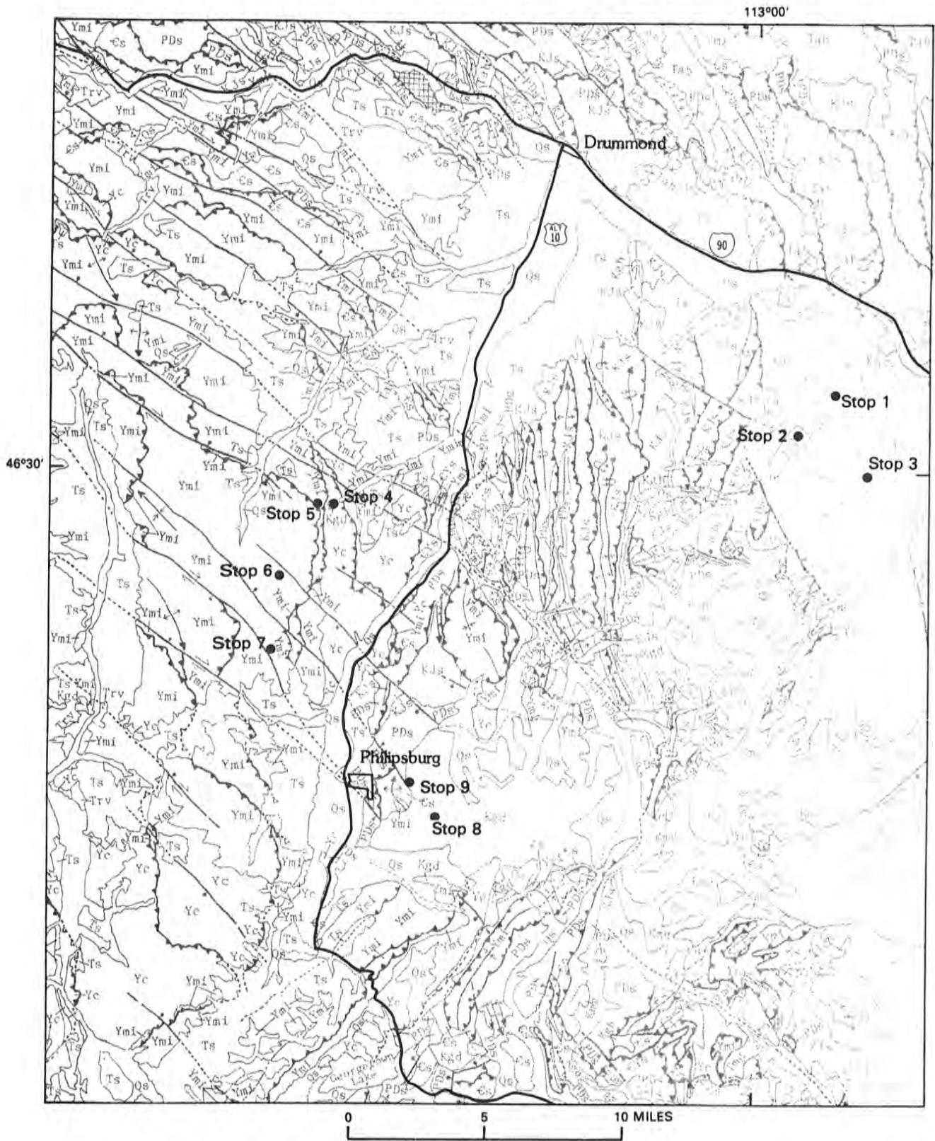
Figure 4-2. Generalized geologic map of John Long Mountains and Flint Creek Range showing field trip stops and major highways (geology from Wallace, 1987b).
