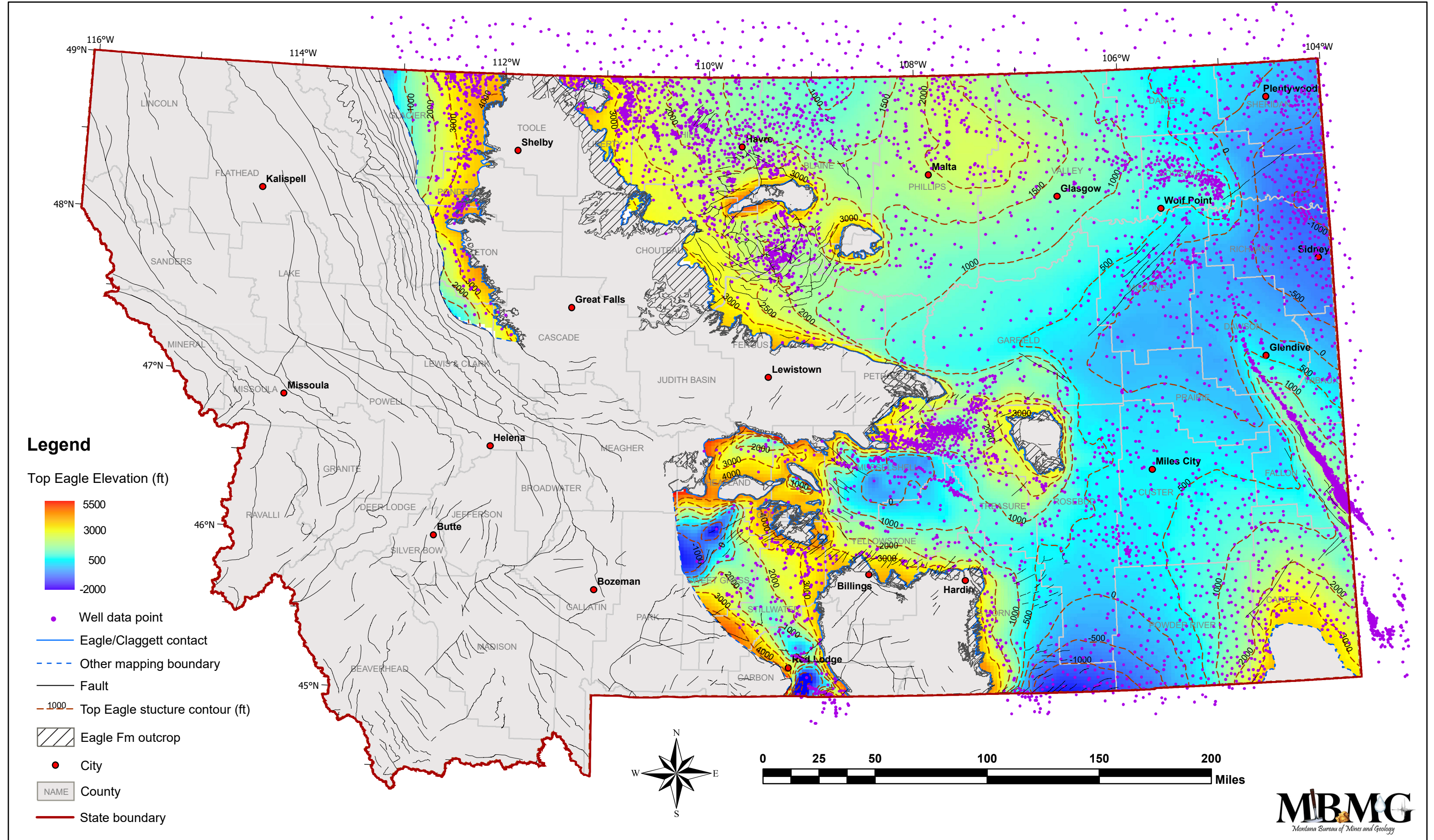
Structure Map of the Eagle Formation, Central and Eastern Montana Jay A. Gunderson
