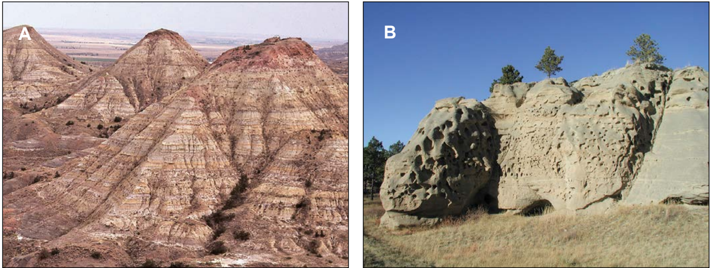
Figure 8. (A) Tongue River Member, near Savage, Montana. (B) Ekalaka Member, near Ekalaka, Montana.
