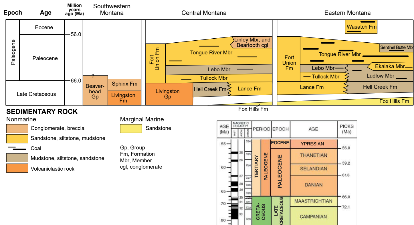
Figure 3. Correlation diagram for synorogenic units in central and eastern Montana, and selected synorogenic units in southwestern Montana. Inset time scale from Walker and others, 2018.
