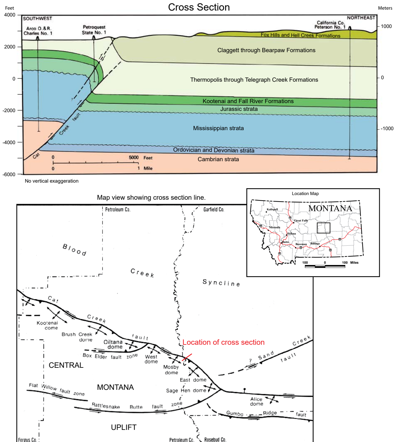
Figure 17. Cross section across Cat Creek Anticline/Fault, northern Central Montana Uplift. Modified from Nelson (1993).
