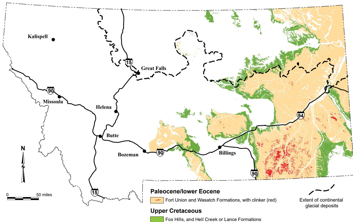
Figure 5. Distribution of Upper Cretaceous Fox Hills, and Hell Creek or Lance Formations; and Paleocene/lower Eocene Fort Union and Wasatch Formations.
