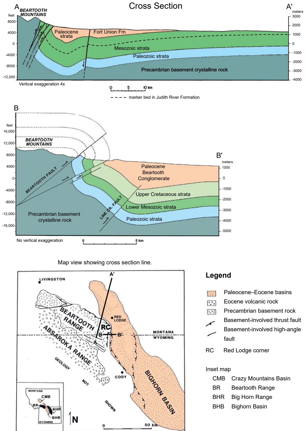
Figure 13. Cross sections across Beartooth Uplift into the Bighorn Basin. A–A' modified from Hagen and others (1985); B–B' and index map modified from DeCelles and others (1991b).
