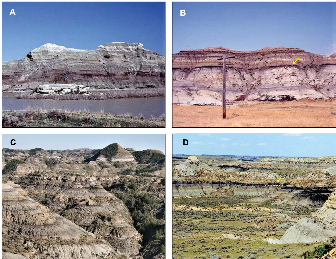
Figure 7. (A) Hell Creek Formation near Webster, Montana. (B) Hell Creek Formation–Ludlow Member contact (~K-Pg boundary) north of Baker, Montana. (C) Ludlow Formation, Makoshika State Park, S.M. Roberts photo. (D) Hell Creek Fm–Tullock Member contact (~K-Pg boundary), Garfield County, Montana, J.H. Hartman photo. Arrows indicate contact positions in (B) and (D).
