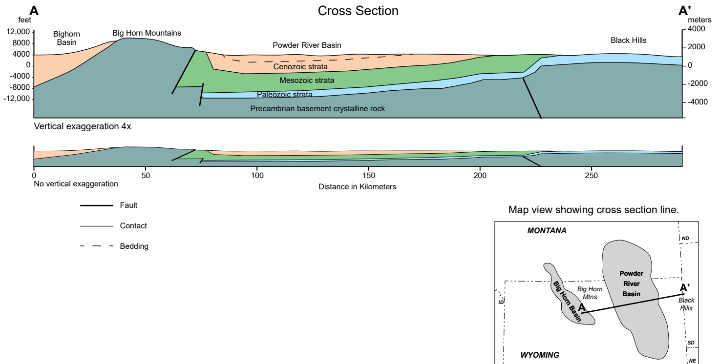
Figure 15. Cross section from eastern Bighorn Basin across Big Horn Mountains and Powder River Basin to Black Hills. Modified from Robbins (1994).
