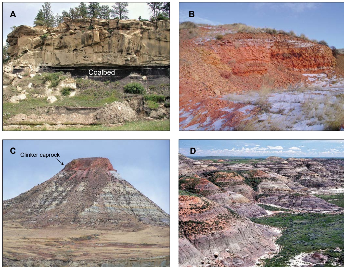
Figure 9. (A) Mammoth coalbed, Bull Mountains Basin near Roundup, Montana, K.B. Waren photo. (B) Clinker bed, C.W. Schwartz photo. (C) Tongue River Member with clinker caprock near Terry, Montana, G.N. Abdo photo. (D) Clinker along Hell Creek–Ludlow contact, near Baker, Montana.
