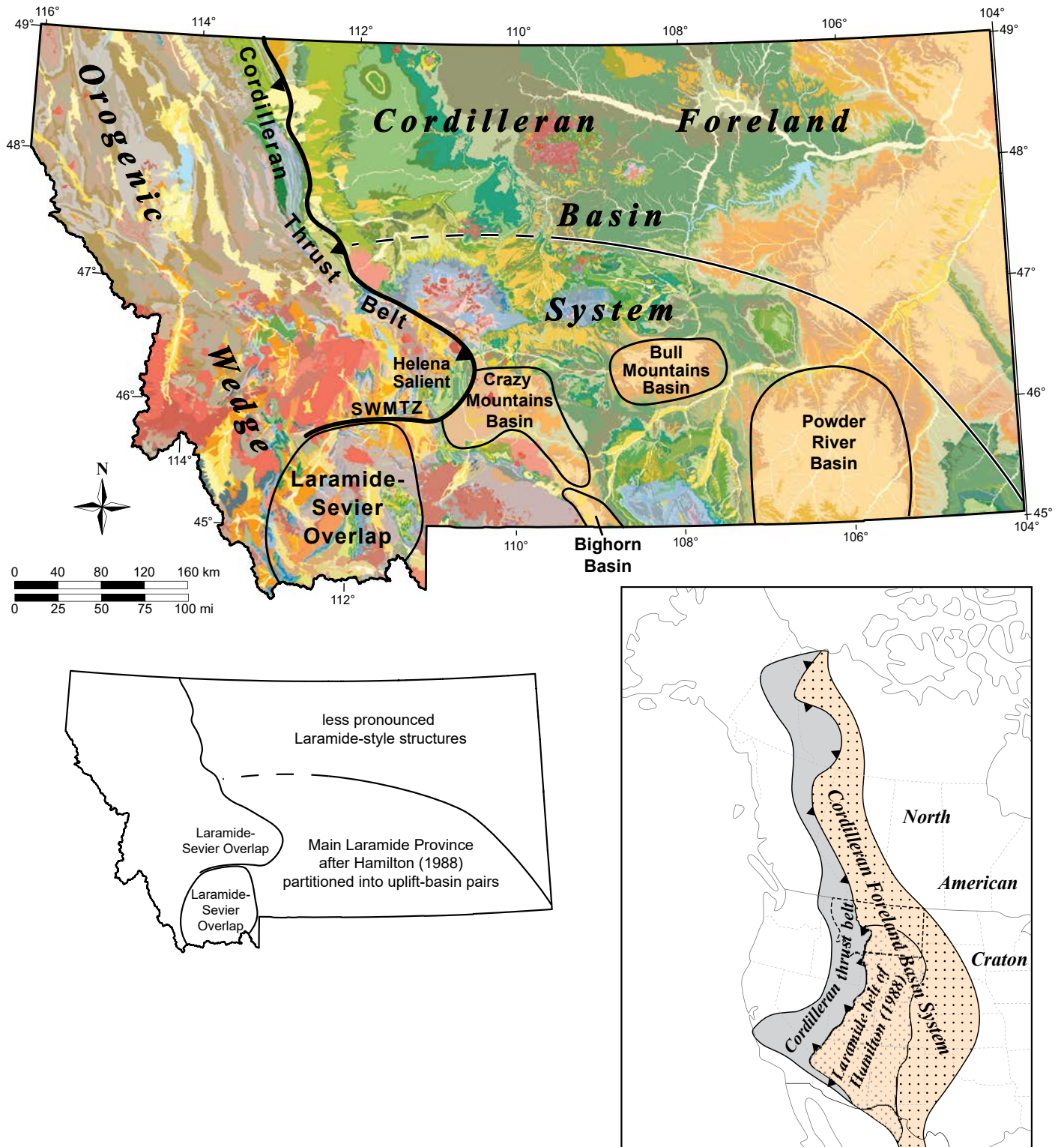
Figure 1. Orogenic provinces and Laramide basins in Montana during Late Cretaceous through earliest Eocene time. Modified from Hamilton (1988), Kulik and Schmidt (1988), and DeCelles (2004). SWMTZ, Southwest Montana Transverse Zone.
