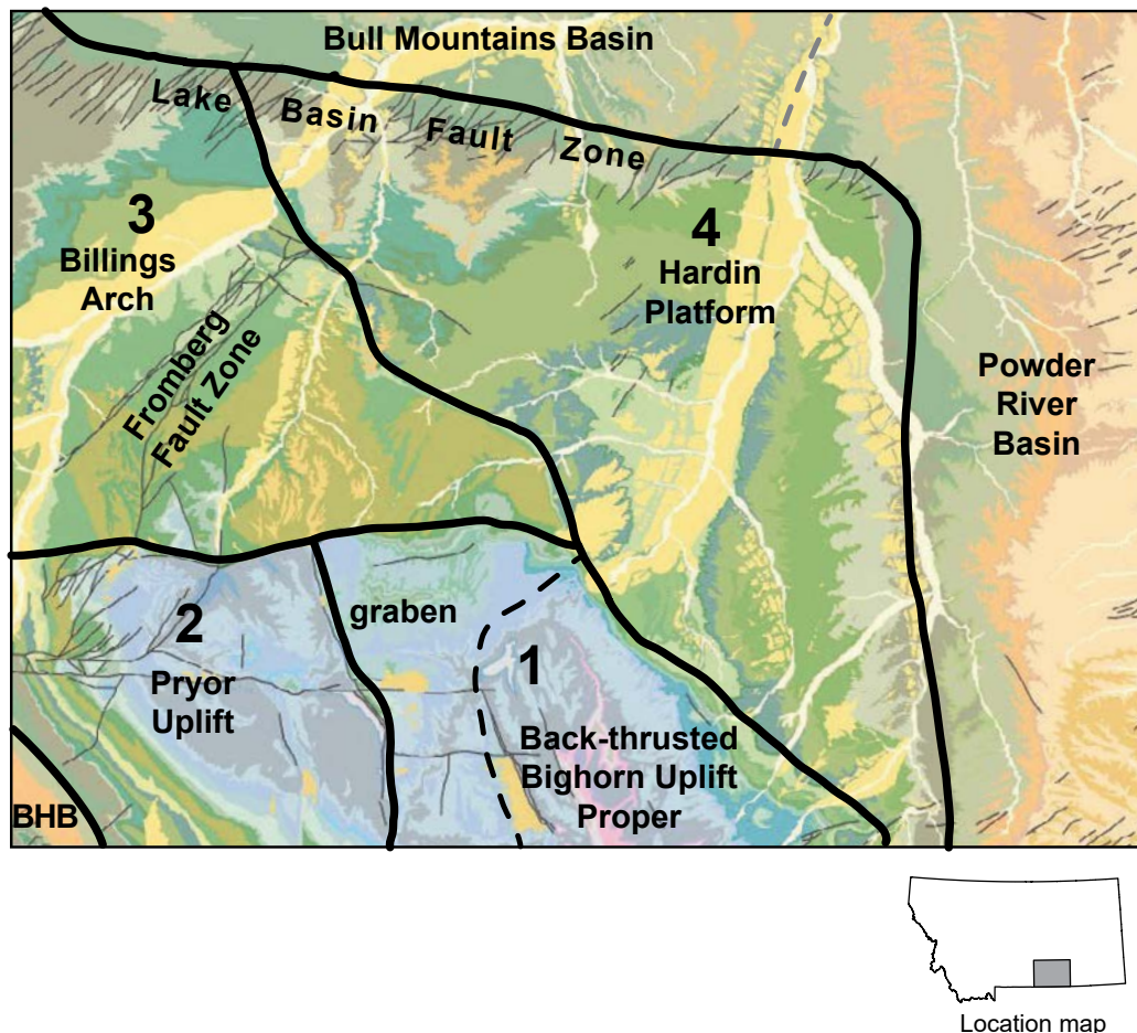
Figure 14. Greater Bighorn Uplift domains and adjacent basins. BHB, Bighorn Basin. Modified from Naus (2000).
