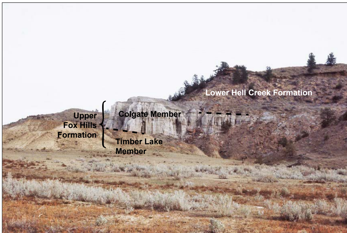
Figure 6. Upper Fox Hills Formation showing Colgate Member, and lower Hell Creek Formation near Glendive, Montana.
