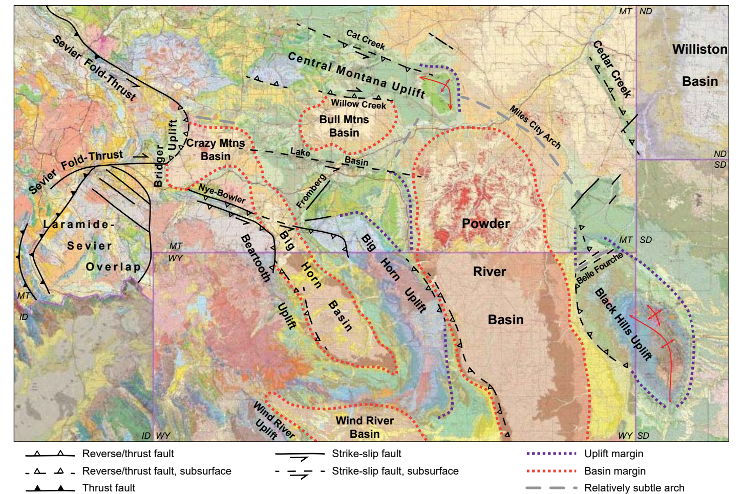
Figure 2. Regional Laramide uplifts, basins, linear features, and other structures. State geologic map base from U.S. Geological Survey National Geologic Map Database.
