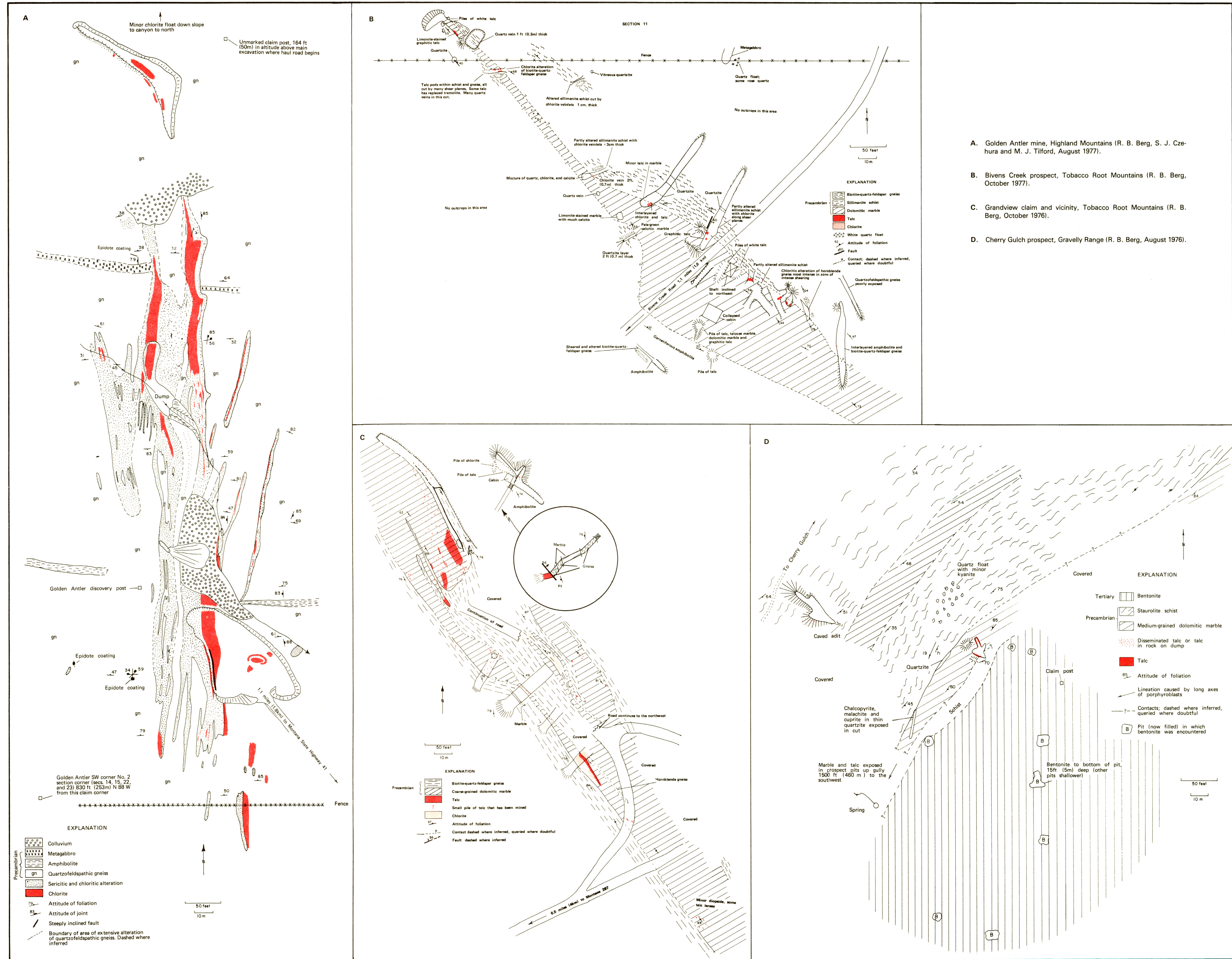
Geologic maps of the Golden Antler mine, Bivens Creek prospect, Grandview claim and Cherry Gulch prospect.
