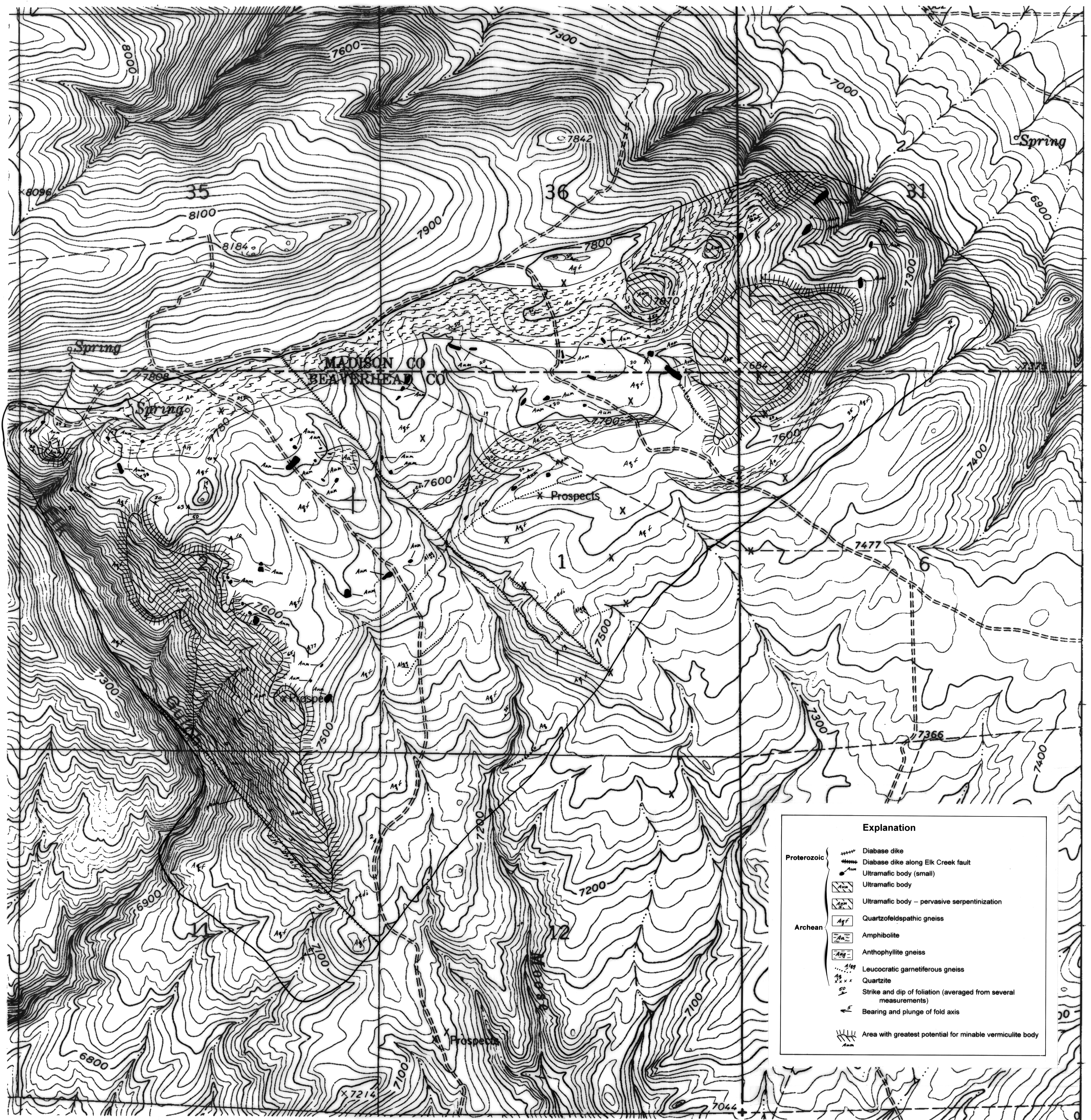
Figure 3. Interpretive geologic map of the Elk Creek vermiculite deposit. Montana Bureau of Mines and Geology Open-File Report MBMG 335.
