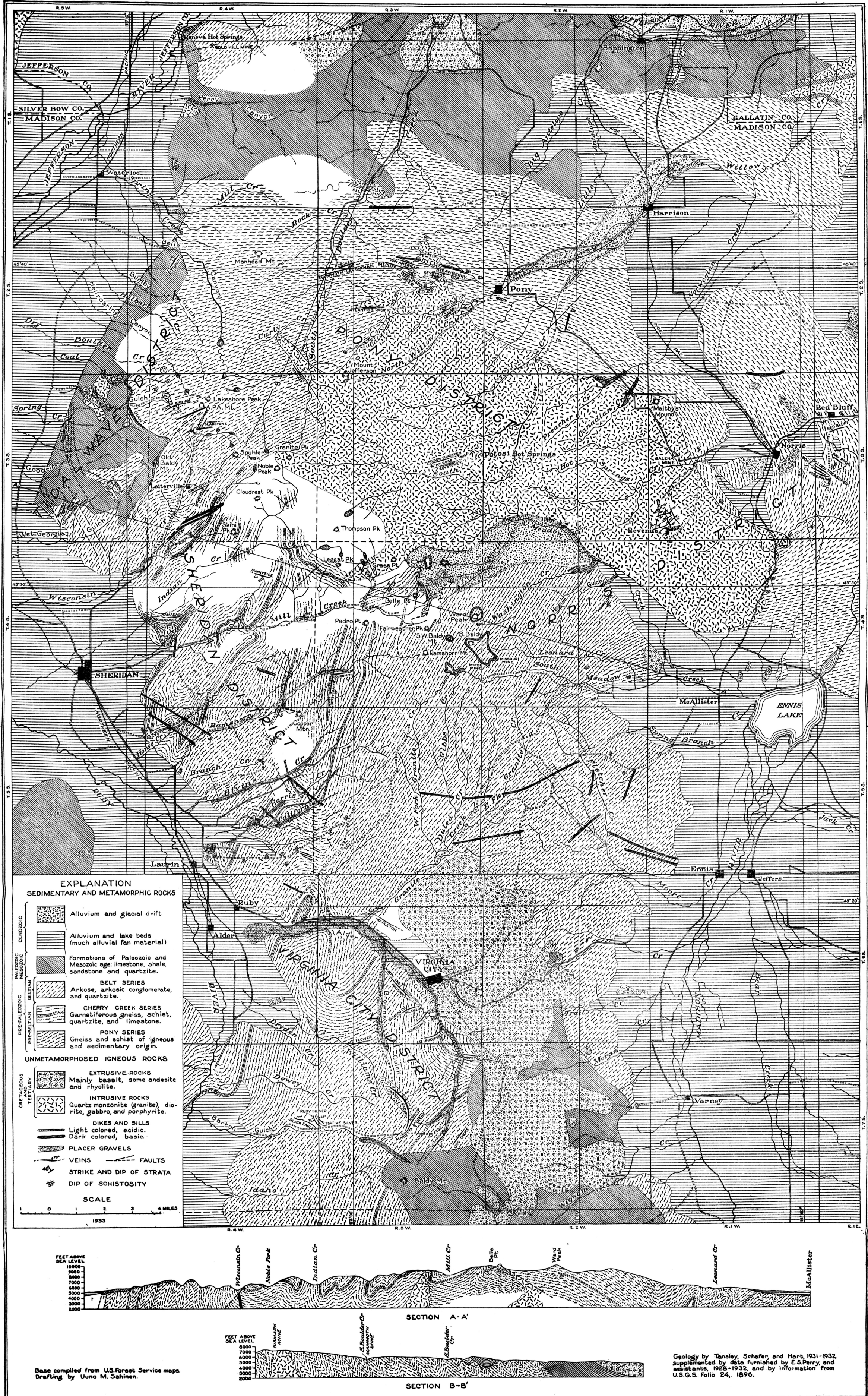
GEOLOGIC MAP AND SECTIONS OF THE TOBACCO ROOT MOUNTAINS, MADISON COUNTY, MONTANA
