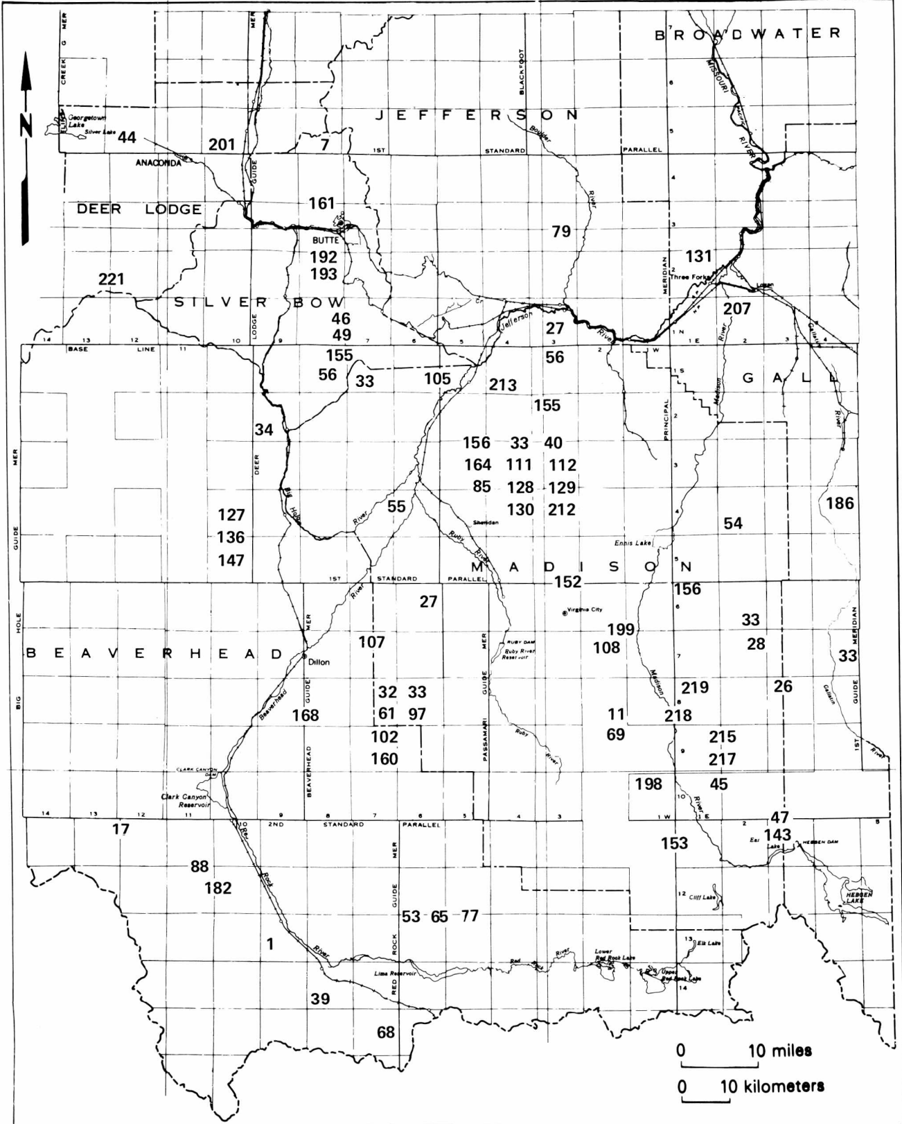
Index Map of Southwestern Montana compiled by Richard B. Berg 1985
