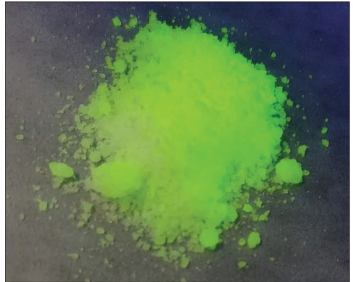
Figure 2. A sample of a Tb phosphor (terbium(III) nitrate hexahydrate) phosphorescing a visible green color in response to ultraviolet ("black") light. Photo by Leiem (CC-BY-SA-4.0).
